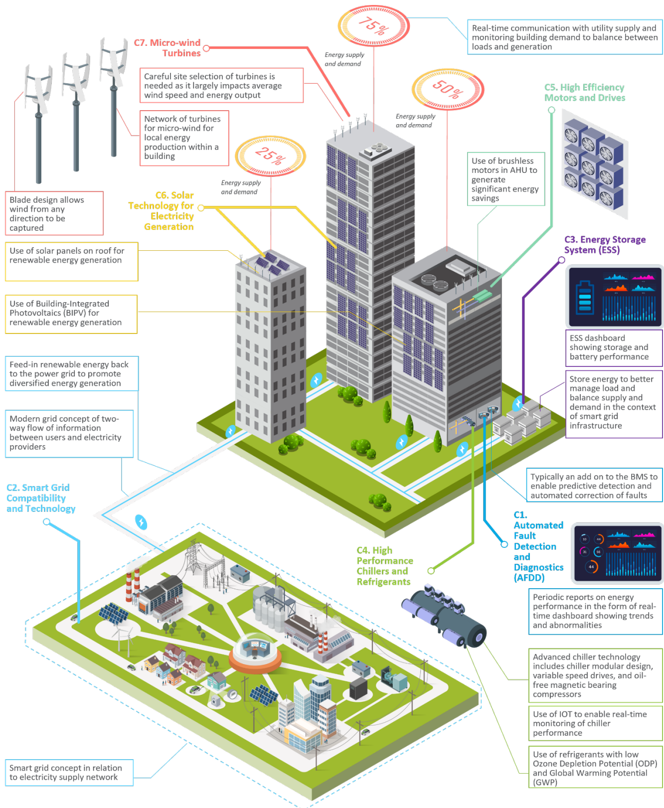
Figure 6 – Building strategies on energy performance
