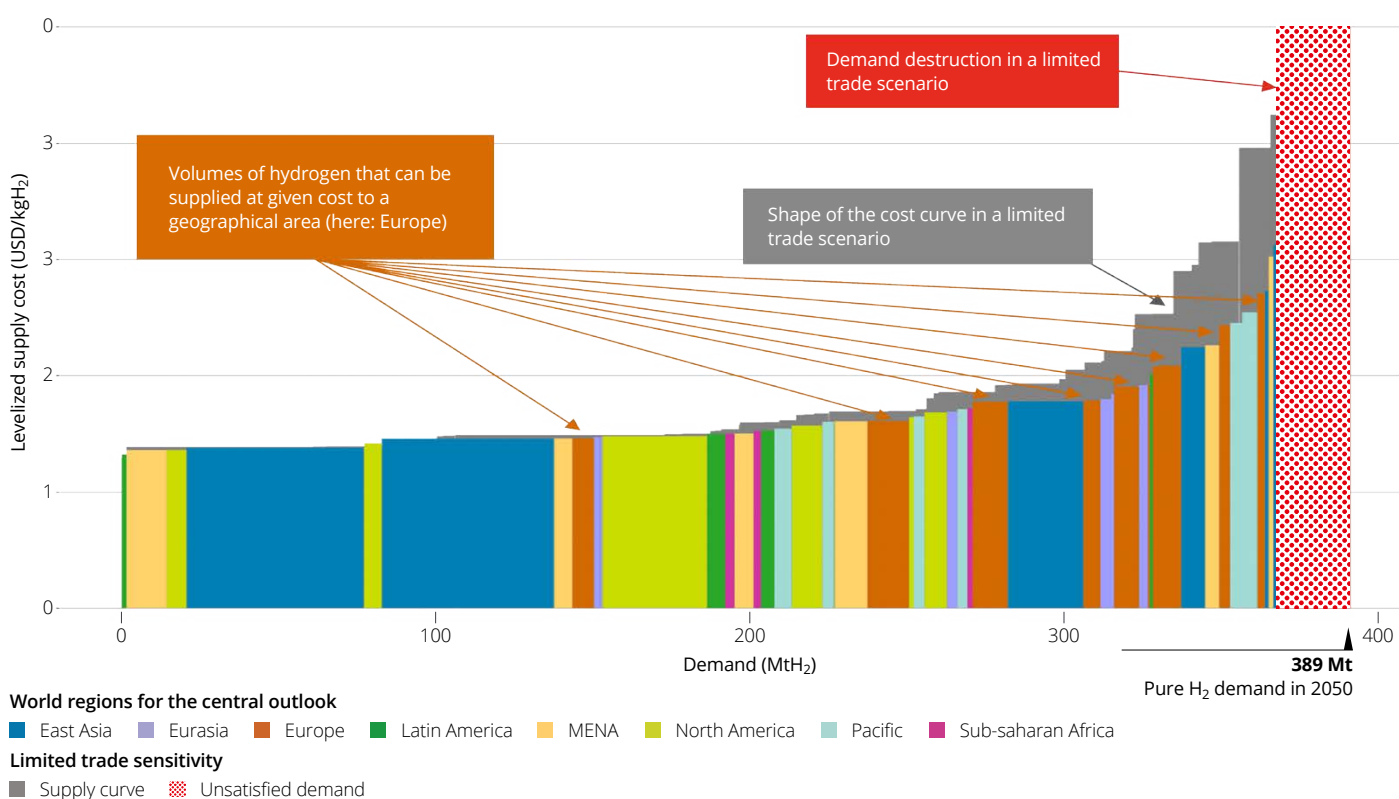
Figure 19. Global landed cost curve for pure hydrogen demand per consuming regions, 2050
