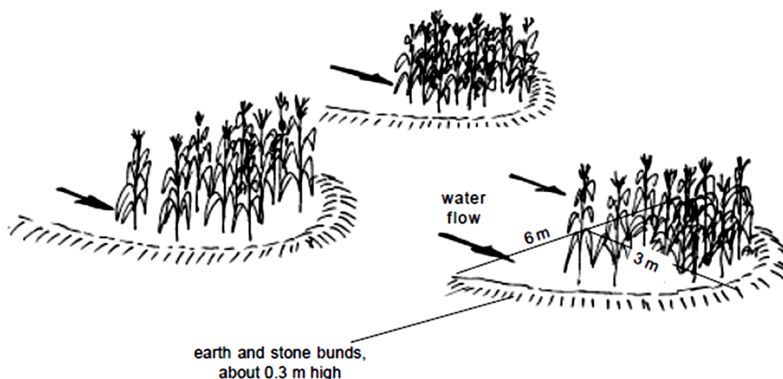
FIGURE 5-7 - HALF-MOON MICROCATCHMENTS
