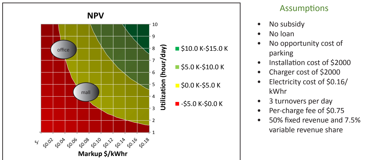
Figure 1: Sensitivity of NPV on Utilization (hours/day) and Electricity Sale Markup ($/kW•h), which is correlated to consumers' willingness to pay
