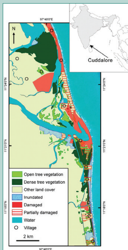
FIGURE 5.1 Pre-tsunami vegetation cover and post-tsunami damage in Cuddalore District, Tamil Nadu, India
