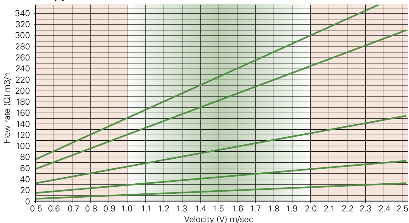
Velocities in pipes of various diameters at various flow rates*
