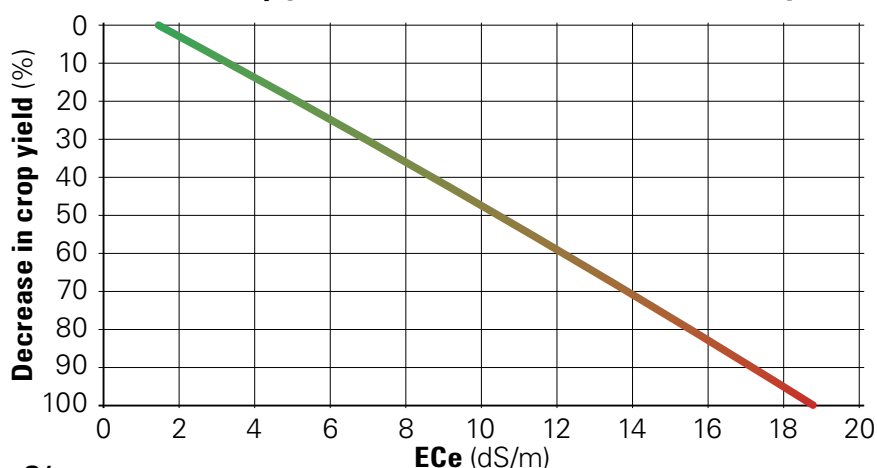
The decrease in crop yield varies with the level of soil salinity
