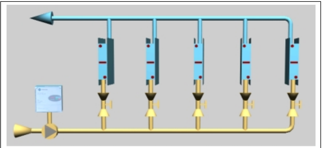
Figure 7 - Direct Return Piping
