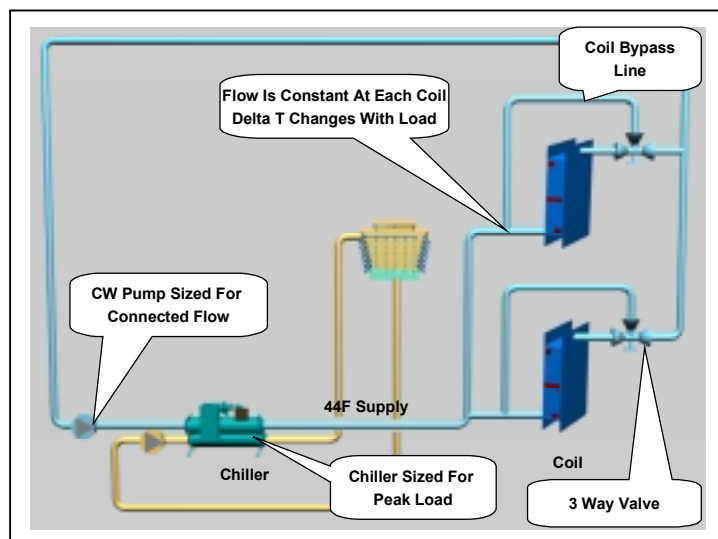
Figure 24 - Three-way Valves
