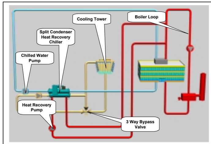
Figure 62 - Split Condenser Type Heat Recovery
