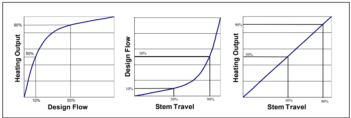
Figure 21 - Coil and Control Valve Performance Curves
