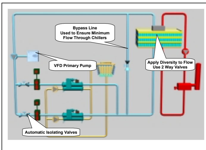
Figure 67 - Variable Primary Flow System
