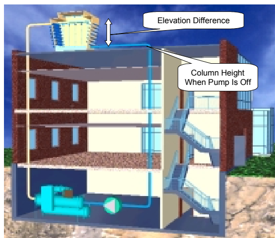
Figure 4 -Open Loop
