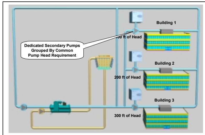
Figure 46 - Multiple Secondary Loops
