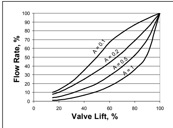
Figure 23 - Distortion of Equal Percentage Valve Characteristic
