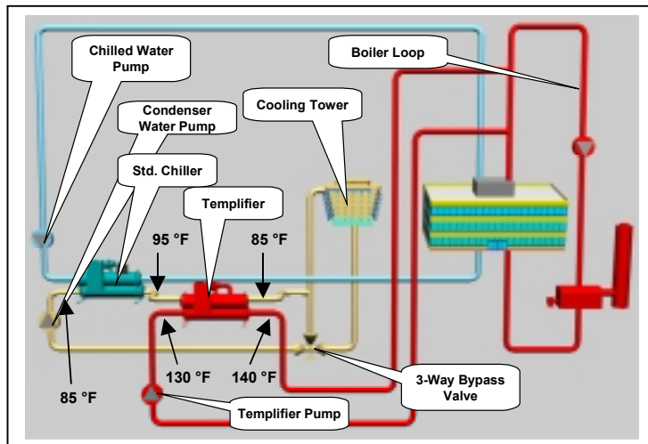
Figure 65 - Templifier™ in a Condenser Loop
