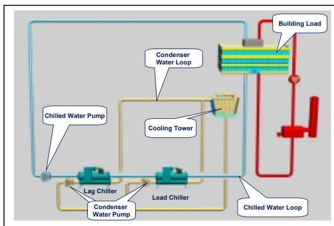
Figure 40 - Typical Series Chiller System
