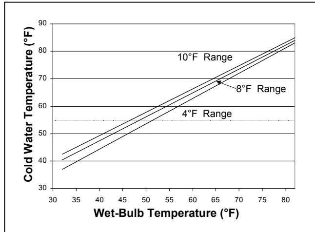
Figure 58 - Cooling Tower Performance Optimized For Free Cooling
