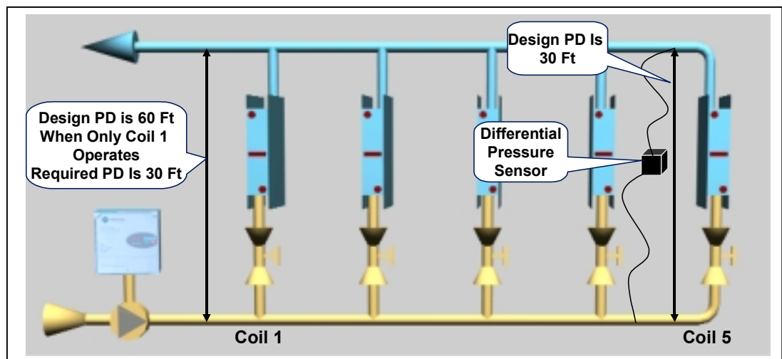
Figure 12 - Secondary Pump Control in Direct Return Systems
