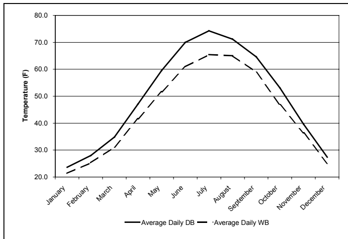
Figure 28 - Annual Ambient Drybulb Vs. Wetbulb
