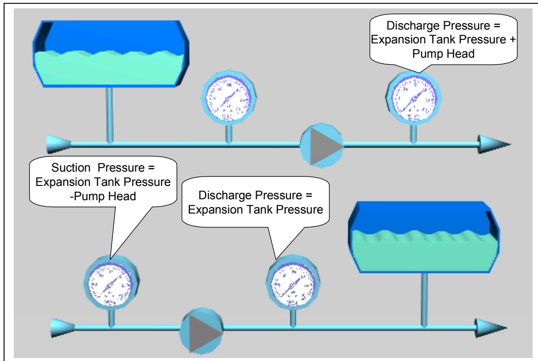
Figure 5 - Expansion Tank Location
