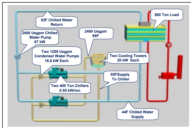
Figure 37 – Basic Parallel Chiller System Operation
