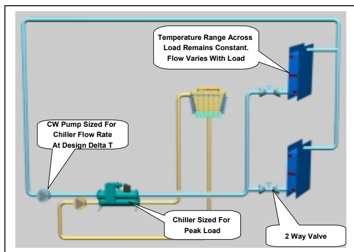
Figure 25 - Two-Way Valves
