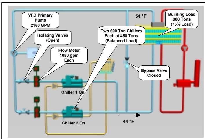
Figure 66, - Basic Variable Primary Flow Operation
