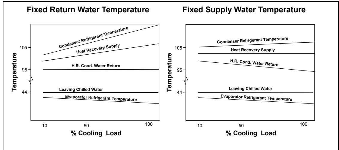
Figure 63 - Heat Recovery Chiller Control Options
