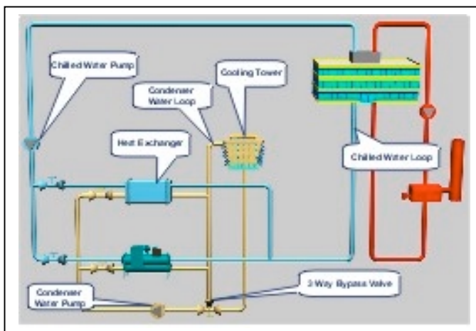
Figure 54, Waterside Free Cooling With Heat Exchanger In Parallel
