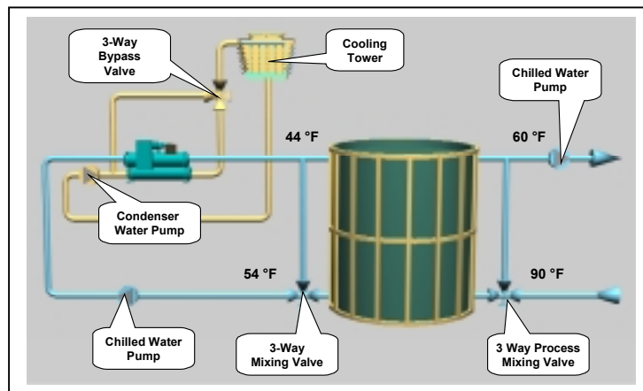
Figure 75 - Process Piping Arrangement
