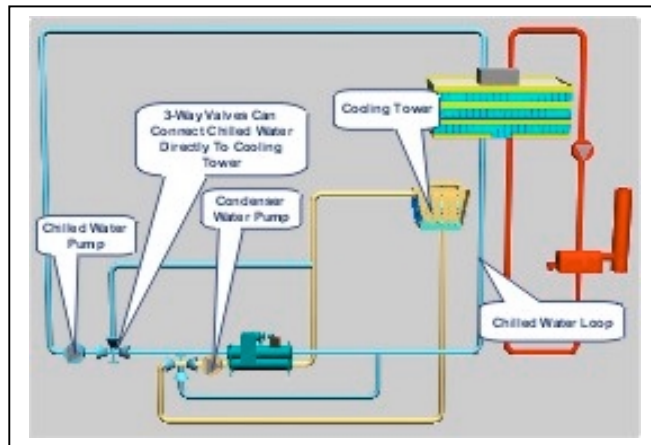
Figure 53 - Direct Water-side Free Cooling
