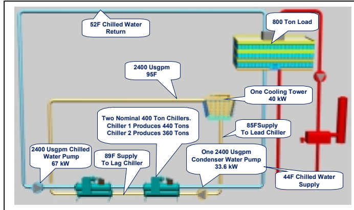
Figure 41 - Series Counterflow System Design
