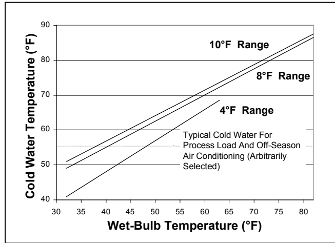
Figure 57 - Cooling Tower Performance Curve at Standard Conditions
