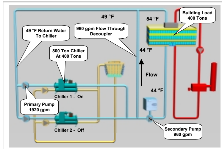
Figure 69 - Primary/Secondary Loop at 50% Load
