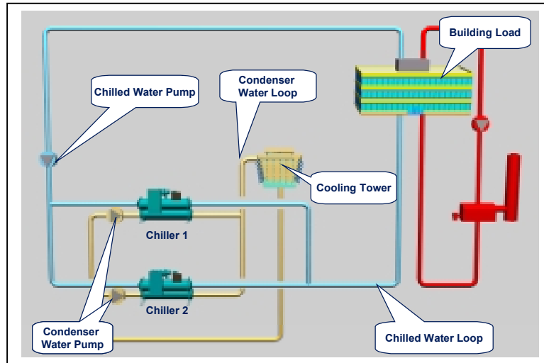
Figure 38 - Typical Parallel Chiller System
