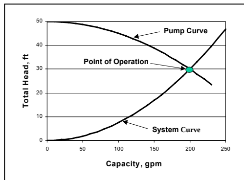
Figure 9 - Basic Pump Curve
