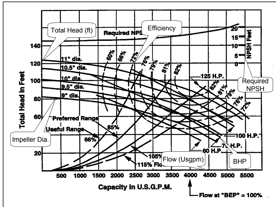
Figure 11 – Typical Centrifugal Pump Curve
