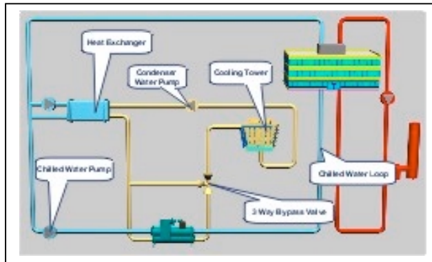
Figure 56 – Free Cooling with Tertiary Loop
