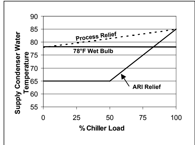
Figure 74 - ARI 550/590 vs. Process Condenser Relief
