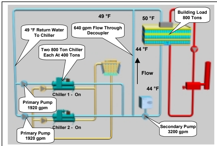
Figure 71 - Primary/Secondary Loop with Low Delta T Reality
