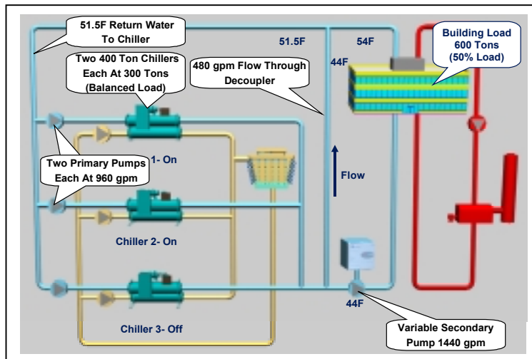
Figure 42 - Basic Primary/Secondary System Operation (50% Load)
