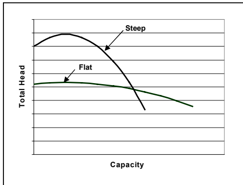
Figure 10 - Pump Curve Profiles
