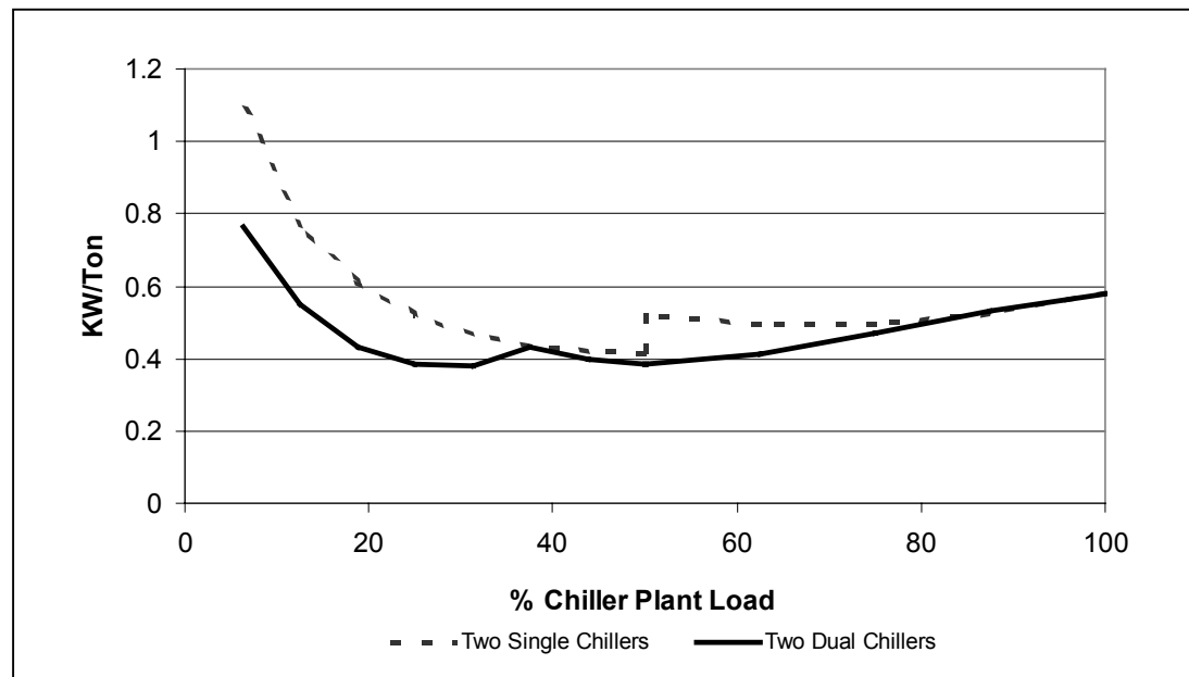
Figure 32 - Chiller Performance Vs. Plant Load
