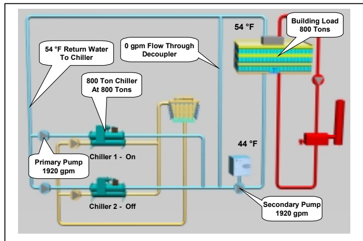
Figure 68 - Primary/Secondary Loop at Full Load
