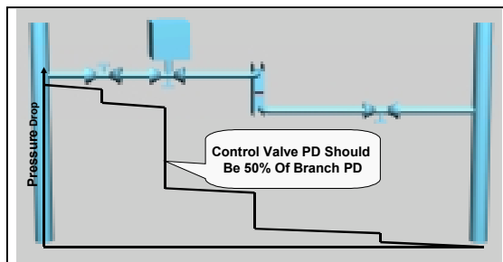
Figure 22 - Pressure Drops and C_v
