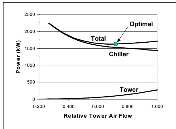
Figure 17 - Chiller Power Vs. Tower Power 4
