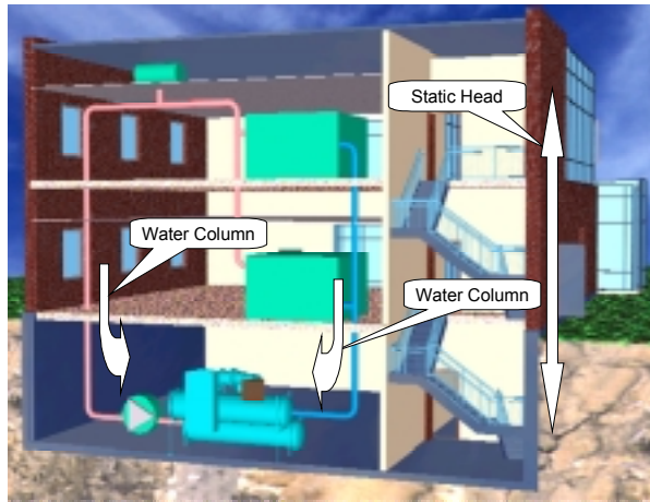
Figure 3 - Closed Loop
