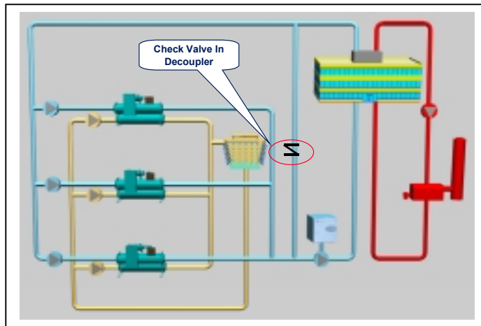
Figure 73 - Check Valve in Decoupler
