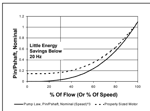
Figure 13 - Pumping Power vs. Flow 3
