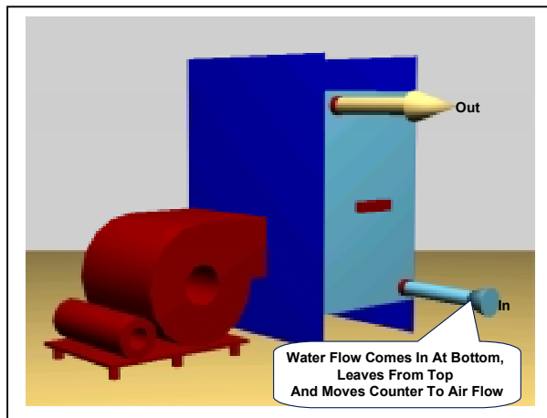
Figure 72 - Proper Coil Connections
