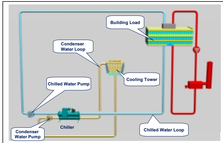
Figure 36 - Typical Single Chiller System
