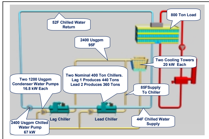
Figure 39 – Basic Series Chiller System Operation
