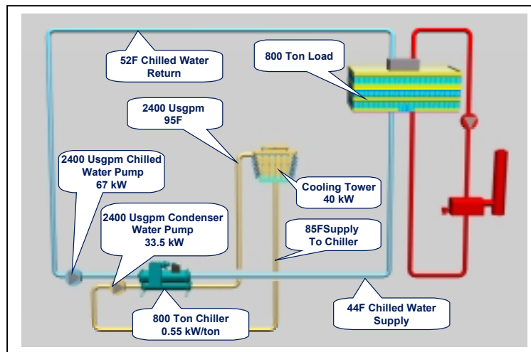
Figure 35 –Basic Single Chiller System Operation
