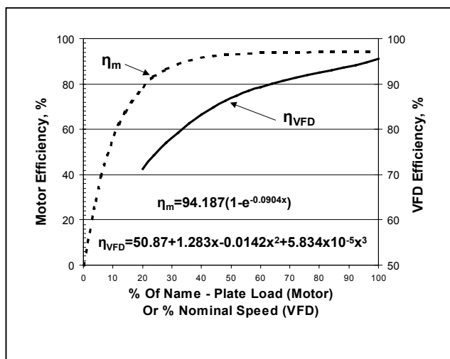
Figure 14 - Motor and VFD Efficiency At Part Load
