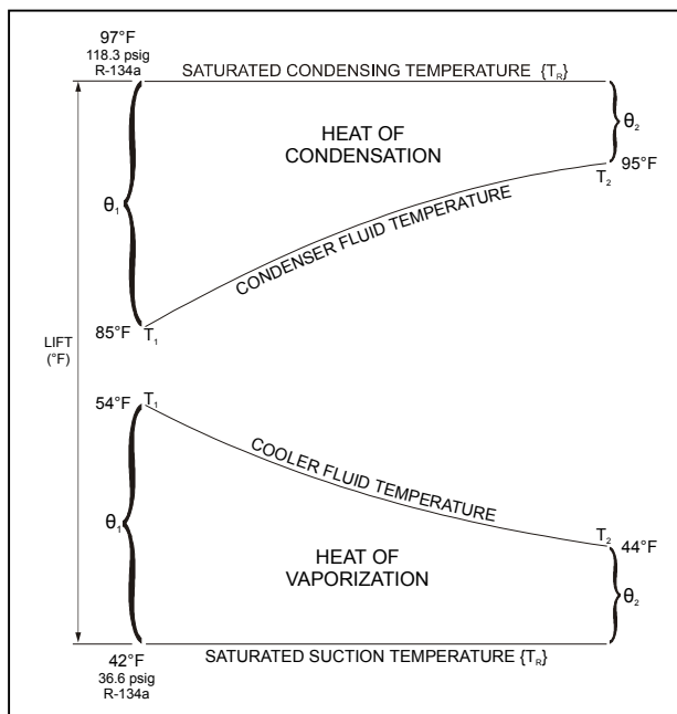
Figure 26 - Chiller Heat Exchanger Conditions
