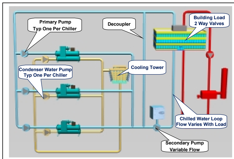
Figure 43 – Typical Primary/Secondary System
