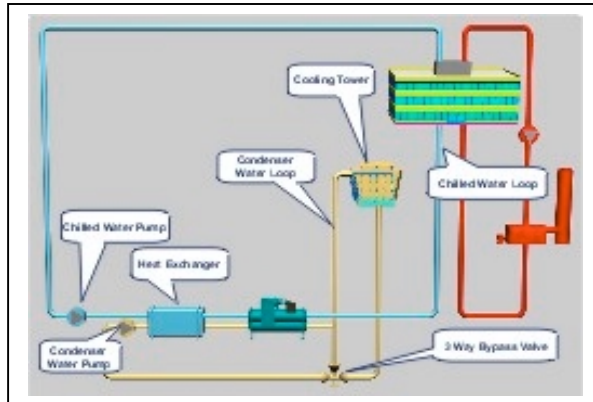
Figure 55, Free Cooling in Series with Chillers
