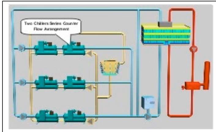
Figure 52 - Series Counterflow Chillers in P/S Arrangement
