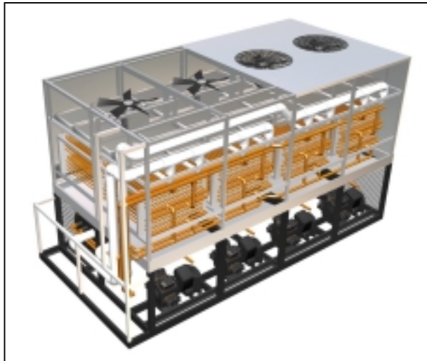
Figure 29 - McQuay EGR Evaporatively Cooled Chiller
