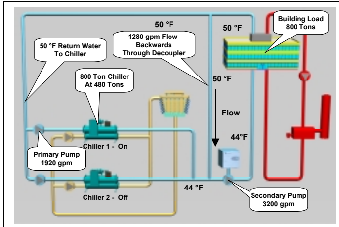
Figure 70 - Primary/Secondary Loop at Low Delta - T
