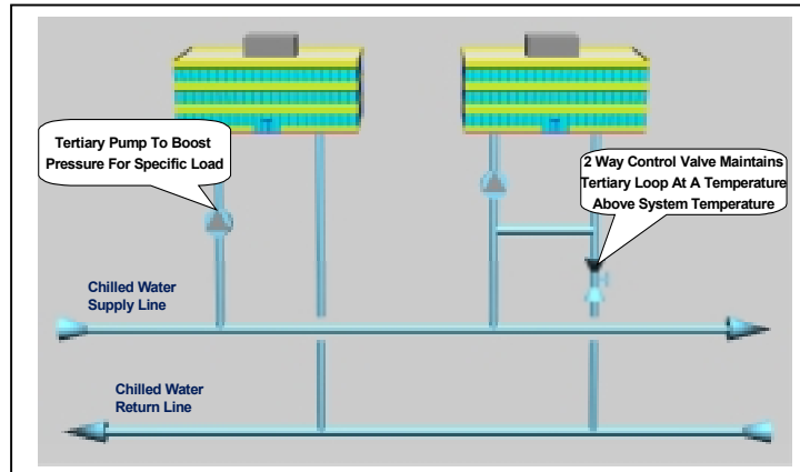
Figure 50 - Tertiary Pumping
