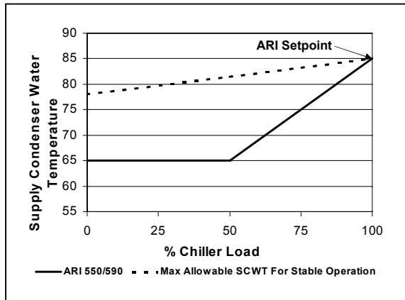
Figure 19 – Chiller Performance with Minimum Setpoint
