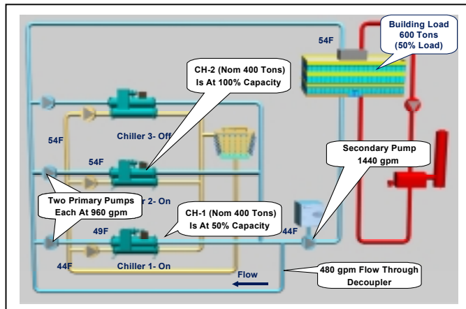
Figure 49 - Backloaded Primary Loop Layout
