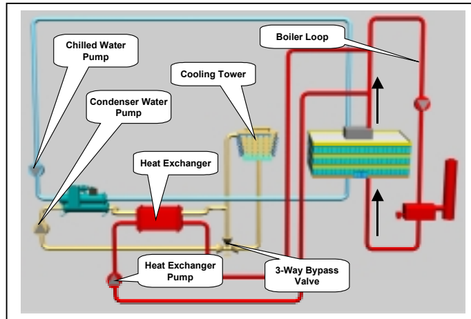
Figure 61 – Single Condenser Heat Recovery
