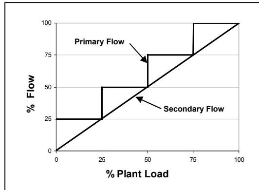
Figure 47 - Primary Vs. Secondary Flow
