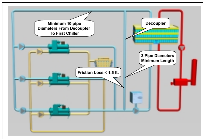
Figure 48 - Decoupler Sizing
