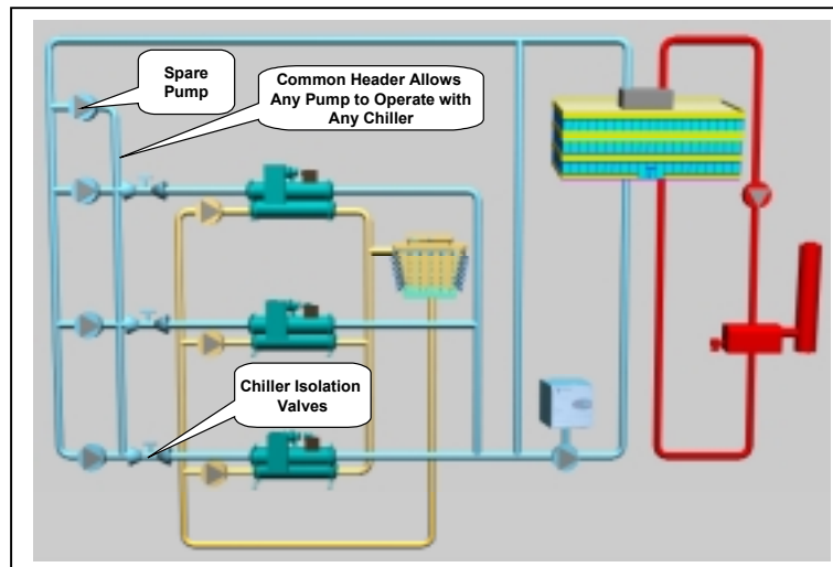
Figure 44 - Alternative Primary Pump Arrangement
