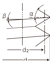
Figure 2-3. Detail drawing
