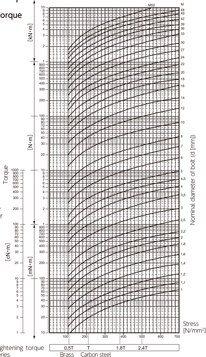
Figure 2-8. Relation between screw and torque
