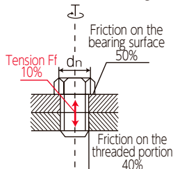
Relational drawing
