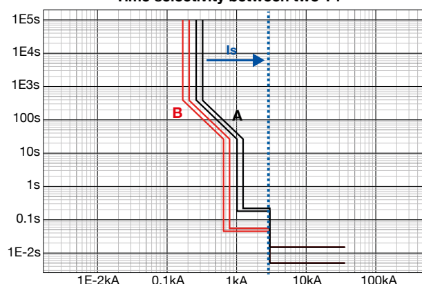
Time selectivity between two T4
