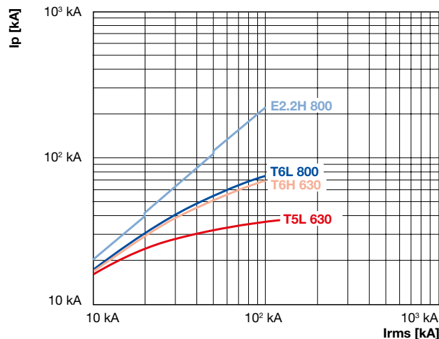
Peak curve
