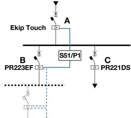
Zone selectivity between Emax 2 and Tmax
