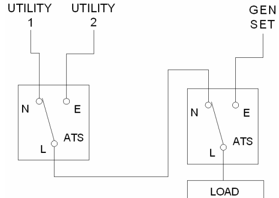
Figure 42 – Multiple Utility – Single Generator Transfer Scheme
