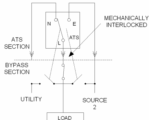
Figure 34 – Make-Before Break
