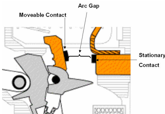
Figure 5 – Arc Gap
