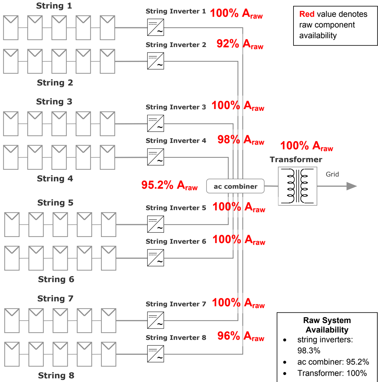
Figure A-2 – String Inverter Availability Comparison
