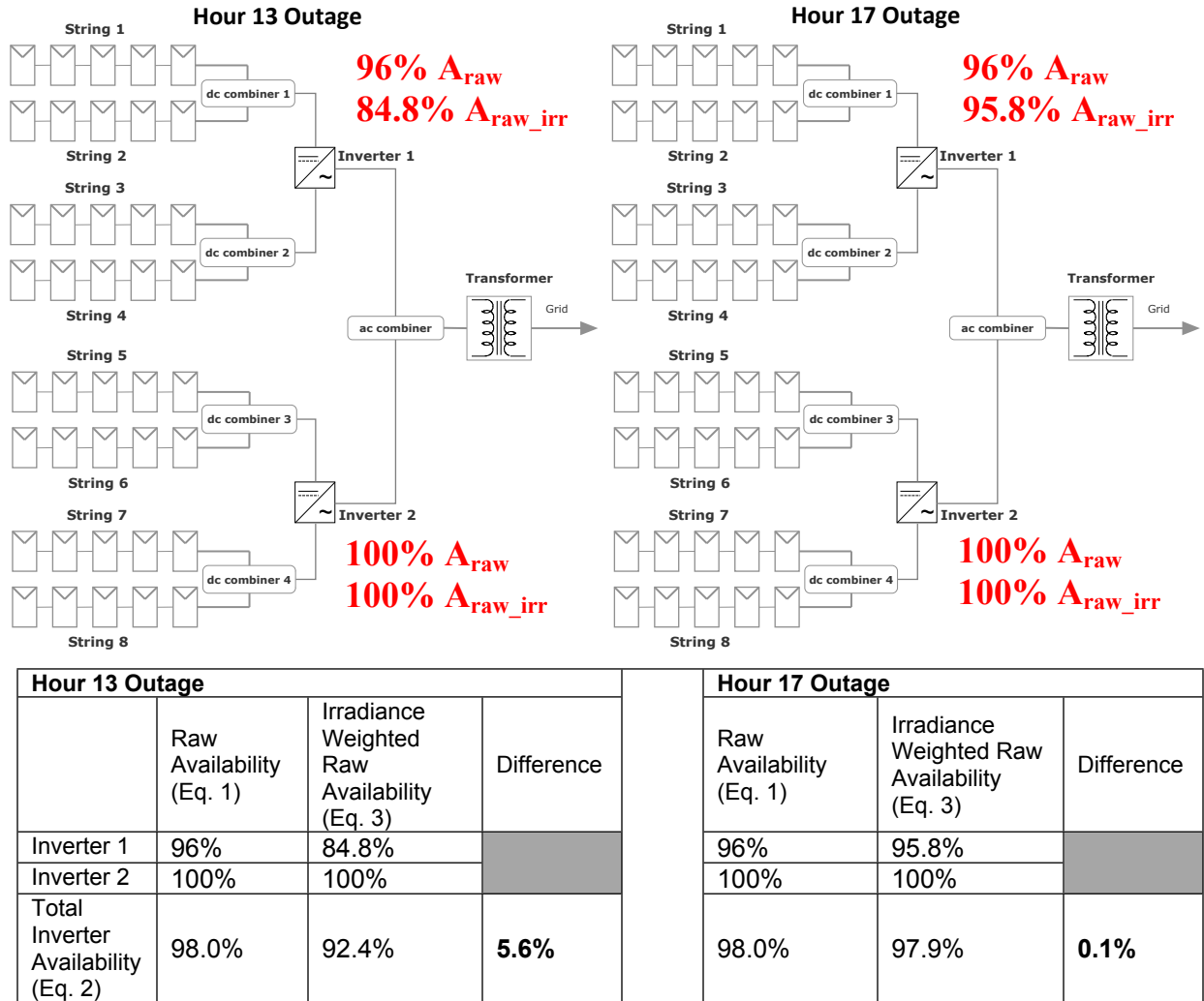
Figure B-2 – Availability Differences for 1-Day Measurement of Irradiance Weighted Availability
