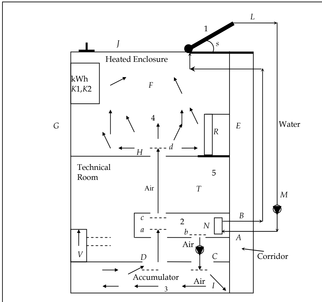
Fig. 13. Simplified chart of the energy system of the Solar House
