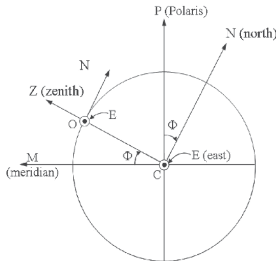
Fig. 3. The coordinate system in the earth-surface frame that consists of OZ, OE and ON axes, in which they point towards zenith, east and north respectively. The transformation of the vector S from earth-centre frame to earth-surface frame can be obtained through a rotation angle that is equivalent to the latitude angle ( \Phi )
