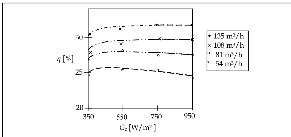
Fig. 7. Efficiency versus irradiation.
