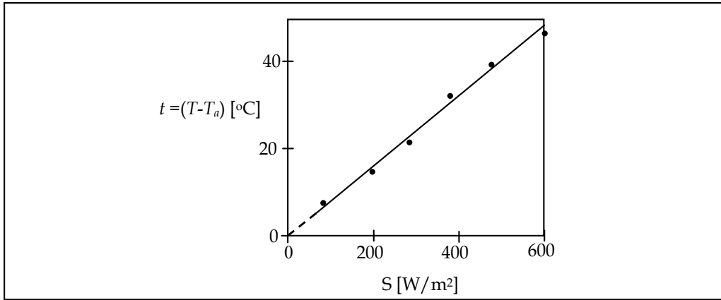
Fig. 5. Temperature rise versus absorbed power density.
