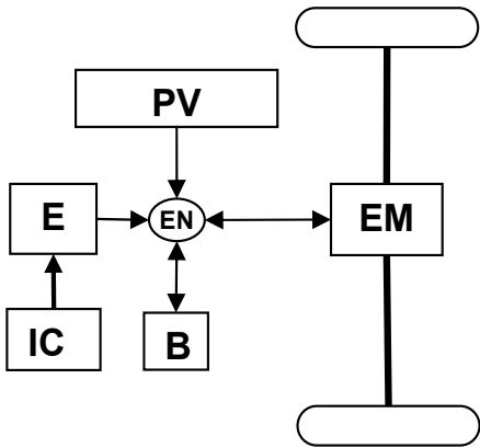
Fig. 11. Scheme of a series Hybrid Solar Vehicle
