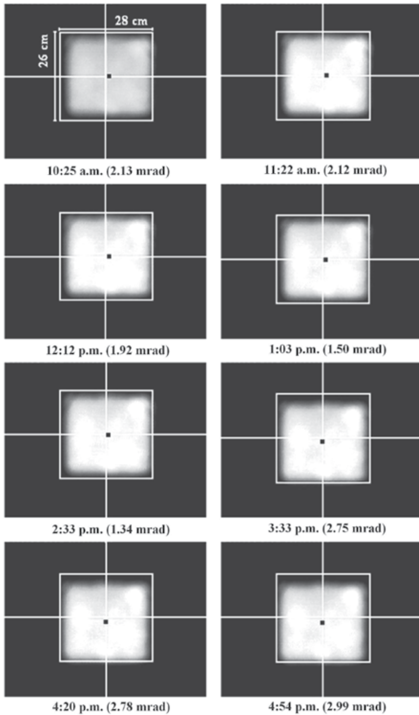
Fig. 15. The recorded solar images on the target of prototype solar concentrator using a CCD camera from 10:25 a.m. to 4:54 p.m. on 16 January 2009 with \phi = -0.1^\circ , \lambda = 0^\circ , and \zeta = -0.5^\circ .
