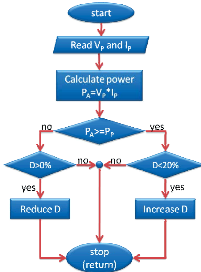
Fig. 22. J.L. Santos algorithm
