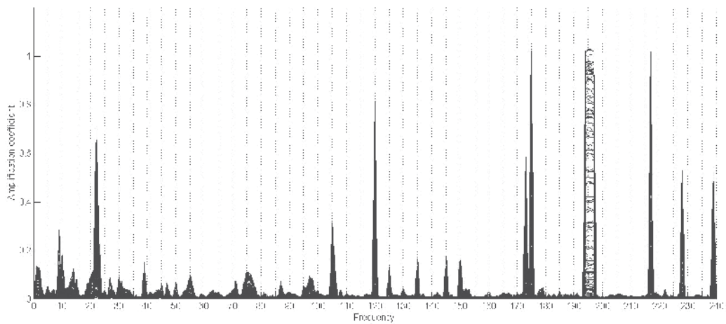
Fig. 13. Fourier spectrum of the sensitivity analysis for the inside air temperature of the building
