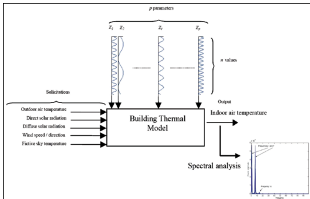
Fig. 12. Procedure of sensitivity analysis.
