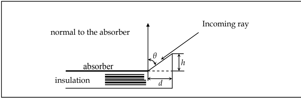
Fig. 3. Shadowing of the surface.
