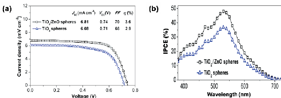
Fig. 19. (a) Photocurrent density-voltage curves, (b) action spectra of the DSCs with anodes made of TiO 2 /ZnO spheres and TiO 2 hollow spheres
