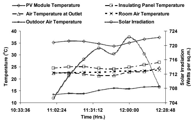
Fig. 7. Variation of mean temperatures of PV module, air and insulating panel with solar irradiation under fan-induced hybrid ventilation
