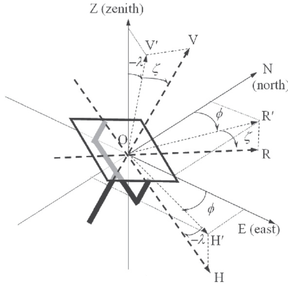
Fig. 7. The combination of the three rotations in 3D view from collector-centre frame to the earth-surface frame, where the change of coordinate system for each axis follows the order: Z \rightarrow V' \rightarrow V , E \rightarrow H' \rightarrow H and N \rightarrow R' \rightarrow R
