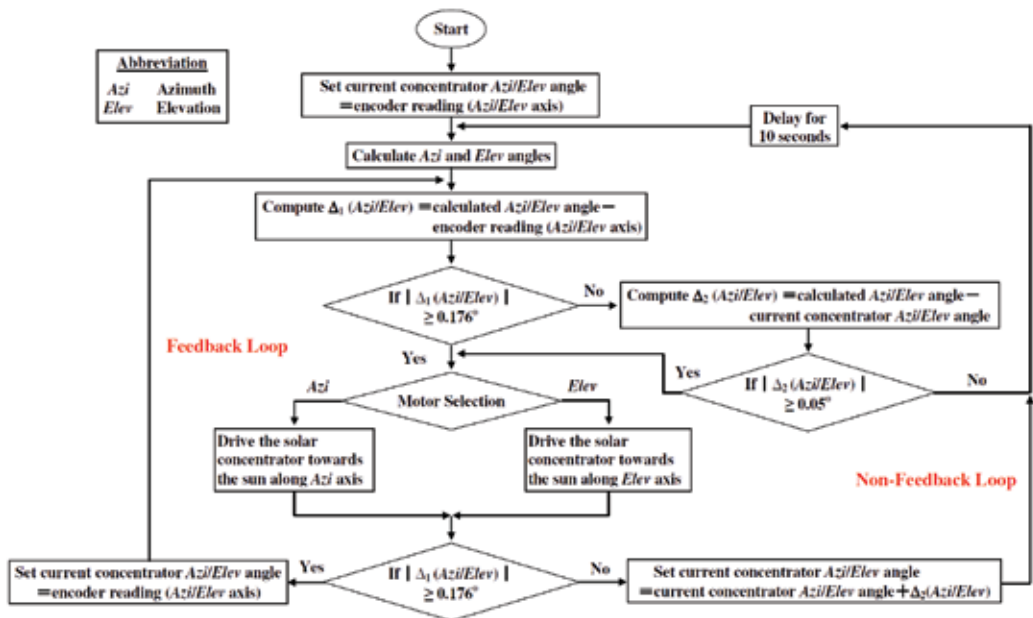
Fig. 16. The algorithm flow of the sun-tracking control program that including motor step count, 1.64 \times 10^{-4} \text{ }^\circ/\text{step} , in fine-tuning the position of solar concentrator prototype and improving the sun tracking accuracy beyond the resolution of the optical encoder.
