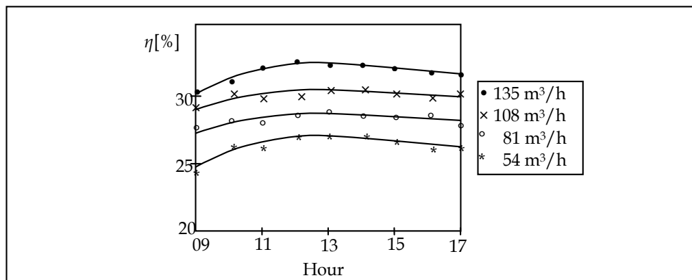
Fig. 8. Hourly variation of the average efficiency.
