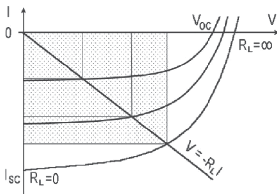
Fig. 1. Some I(V) characteristics of a photovoltaic panel under different work conditions
