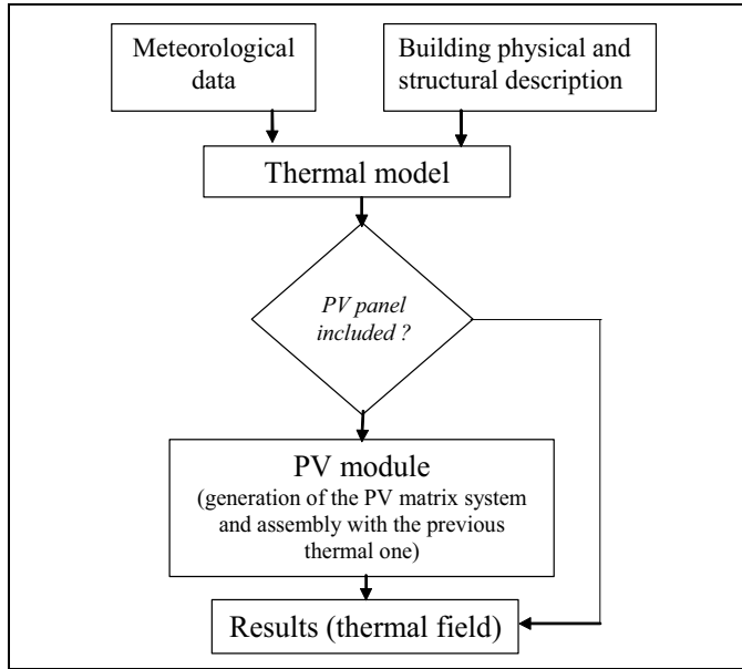
Fig. 5. Integration of the PV calculation module to the existing ISOLAB code.
