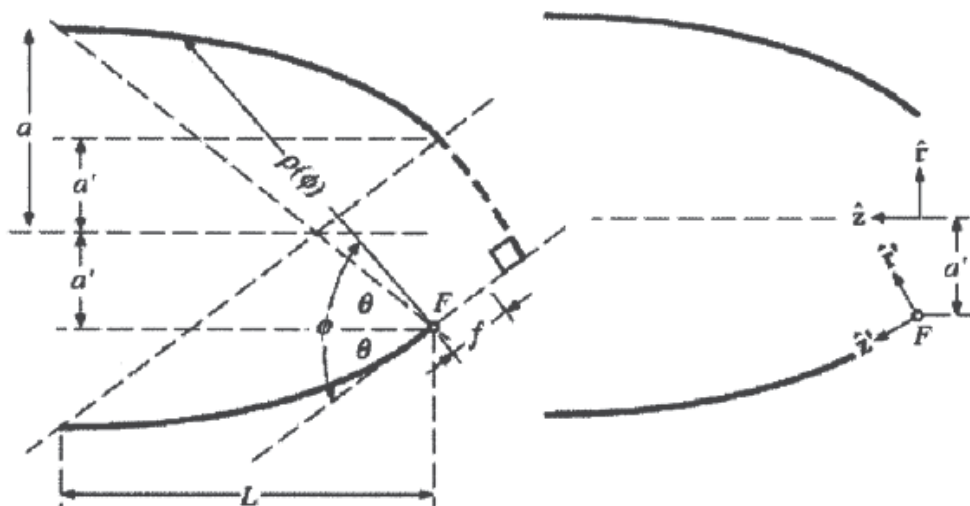
Fig. 4.3. Winston cone concentrator.
