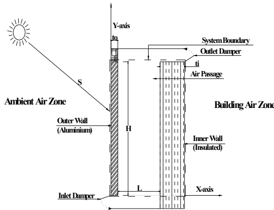
Fig. 1. Schematic of a solar thermosyphon integrated to building air zone
