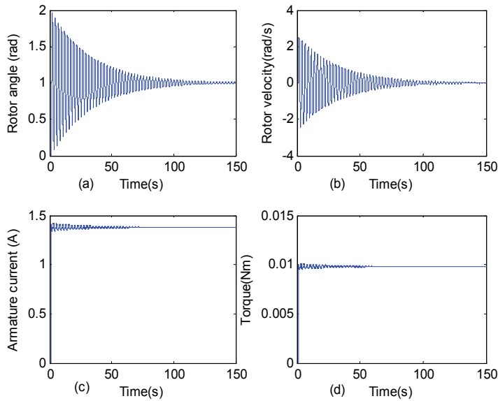
Fig. 11. Dynamics of open-loop platform
