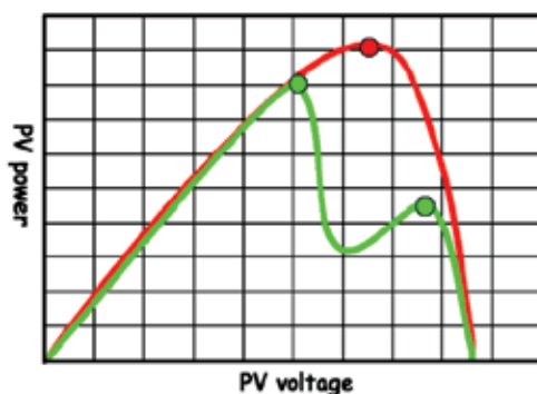
Fig. 9. Power vs. voltage characteristic of a PV field under uniform conditions (red) and with mismatching (green).
