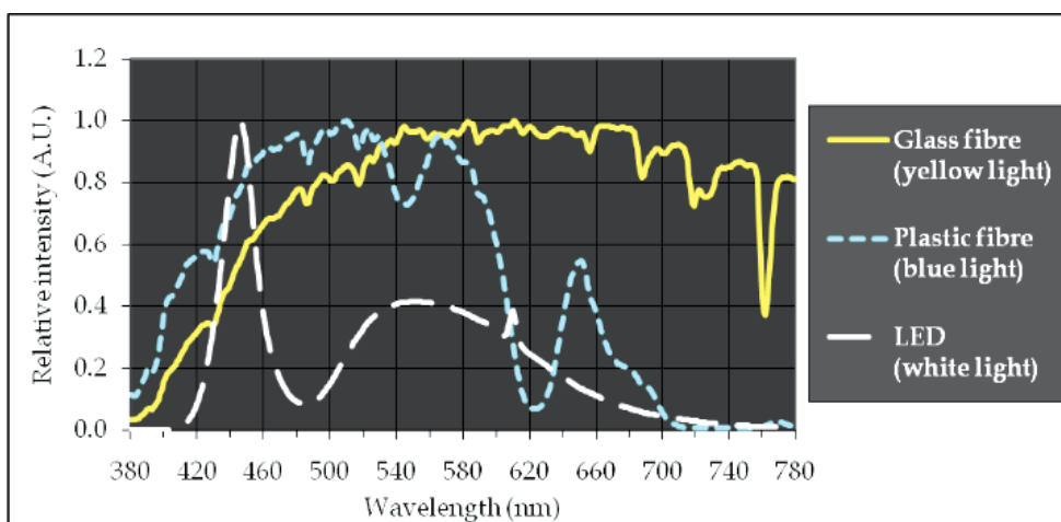
Fig. 18. Spectral comparison of the lighting using white LED, plastic and glass fibres.
