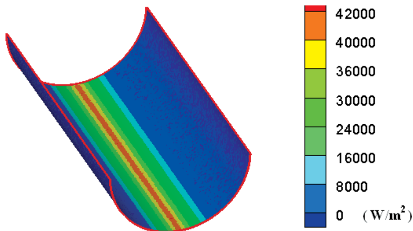
Fig. 2. Concentrated solar irradiation heat flux distribution on the bottom surface of tube receiver.
