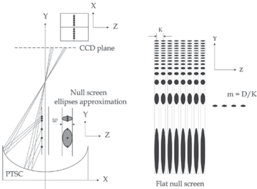
Fig. 13 Inverse ray tracing on the X-Y plane, the elliptical approximation in the Y-Z screen plane, and the flat null screen for testing the PTSC component.
