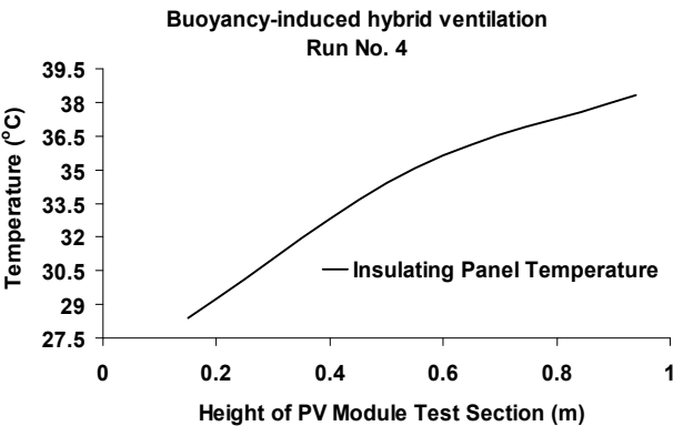
Fig. 6.(b) Temperature plot of insulating panel for buoyancy-induced hybrid ventilation with height of PV module test section
