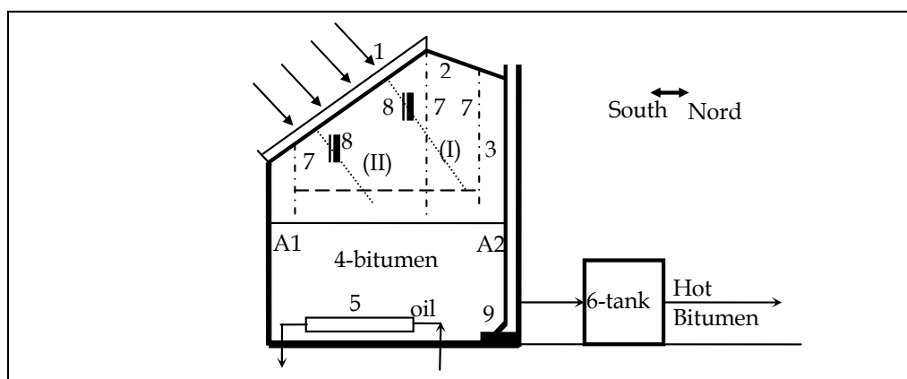
Fig. 19. Diagram of the industrial installation for bitumen preheating.
