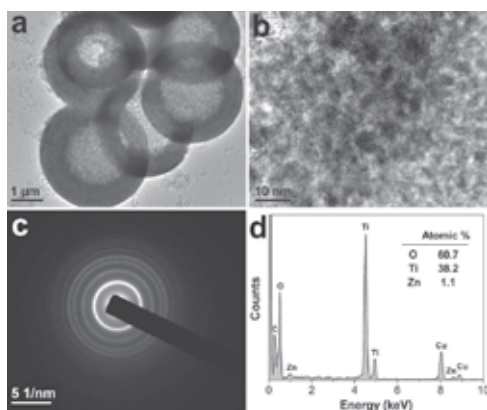
Fig. 16. (a, b) TEM images, (c) selected area electron diffraction (SAED) image, and (d) energy-dispersive X-ray spectroscopy (EDS) of the \text{TiO}_2/\text{ZnO} spheres
