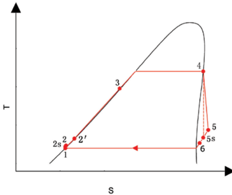
Fig. 2. Thermodynamic cycle of a typical dry fluid
