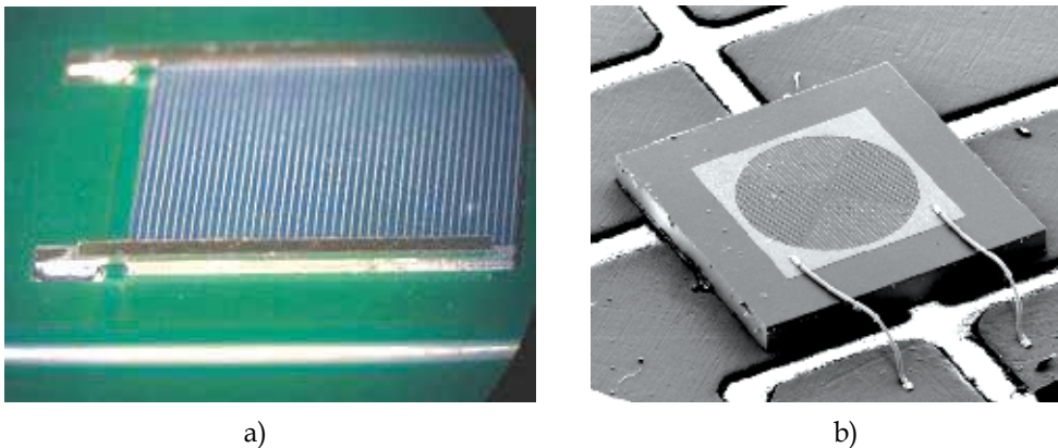
Fig. 12. CPV solar cells assembled on substrates: a) soldered silicon solar cell (Courtesy of CPower Srl); b) solar cell of 1mm 2 assembled with chip on board technology (Courtesy of CRP – Centro Ricerche Plast-ottica)
