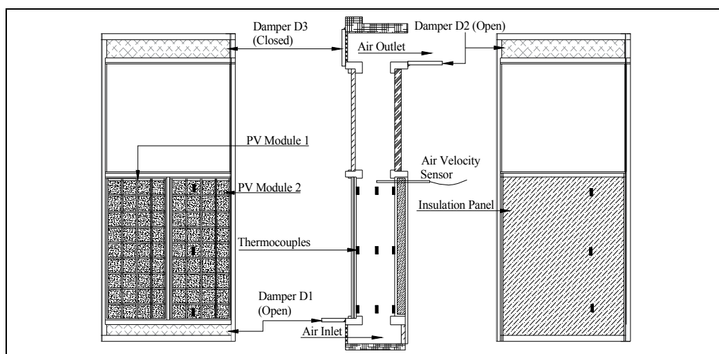
Fig. 4. Schematic of the Experimental Setup
