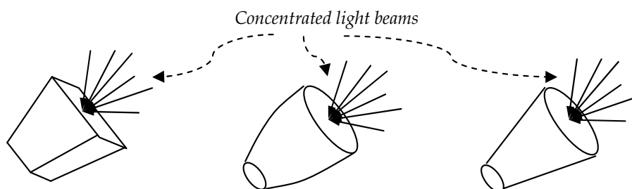
Fig. 5. Examples of geometries for simple secondary concentrators
