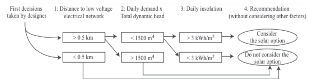
Fig. 3. Diagram for making a decision to use a PV system for pumping water.
