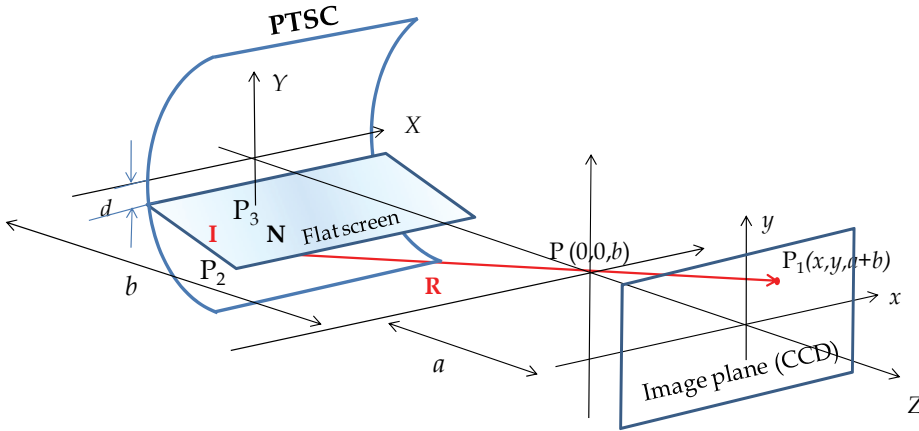
Fig. 8. Setup for the testing for a PTSC with null screens.
