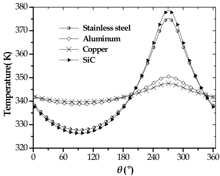
Fig. 8. Temperature profiles across the circumference on the tube inner surface at the tube outlet section
