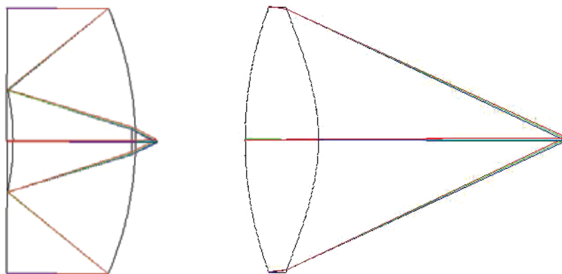
Fig. 17. Comparison of the optical designs: Cassegrain in PMMA (left) and aspherical lens in PMMA (right).
