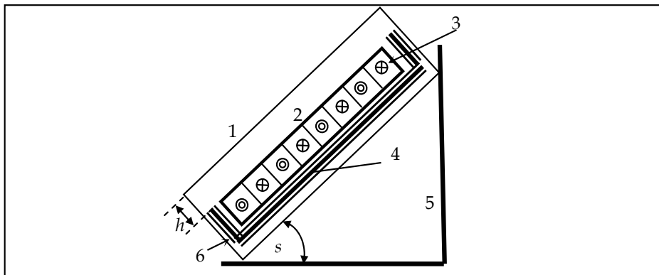
Fig. 1. Air solar collector
