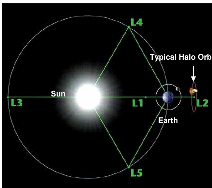
Fig. 19. Lagrange Points of the Earth-Sun system (not to scale). The Earth-sun L2 point distance is 1.5M km from Earth. Also shown an example of a typical halo orbit around L2 (2004), with some concepts of Earth-Sun L2 Design details are exhibited in Table 3. Three new concepts for solar power satellites were invented and analyzed:
