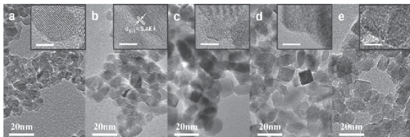
Fig. 10. TEM images of the as-prepared \text{TiO}_2 nanoparticles with different Nb contents (a) 0 mol%, (b) 2.5 mol%, (c) 5.0 mol%, (d) 7.5 mol%, and (e) 10.0 mol%. Inset shows the corresponding HRTEM image of each sample (Scale bar 5 nm)
