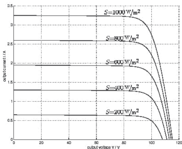
Fig. 1. I-V characteristics of a photovoltaic panel for different values of irradiance S at a temperature of 25 °C.
