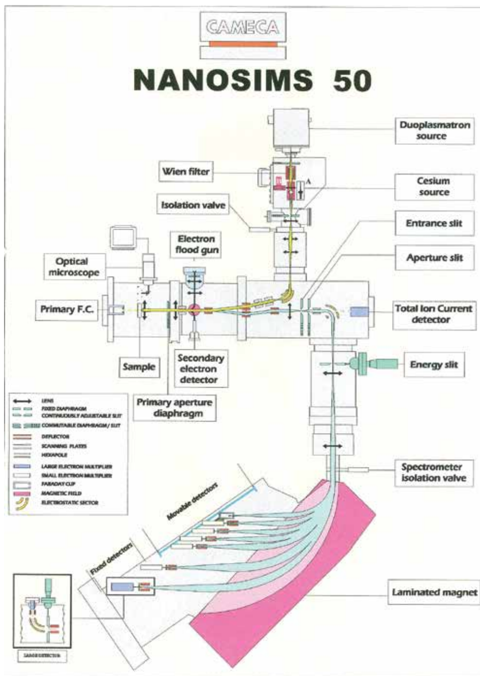
Fig. 4a. The NanoSIMS 50 of CAMECA (Courtesy of CAMECA, Paris)
