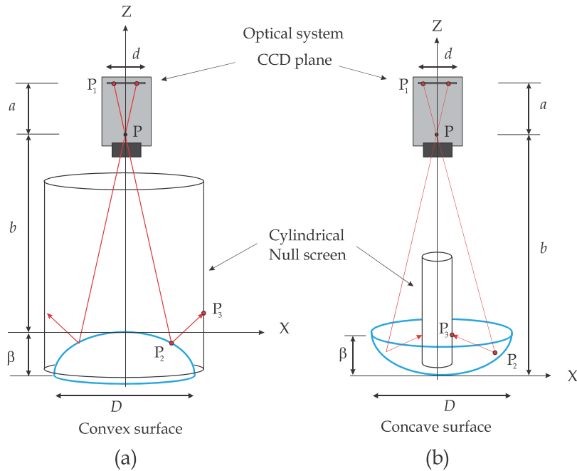
Fig. 1. Setup for testing a) a convex and b) a concave
