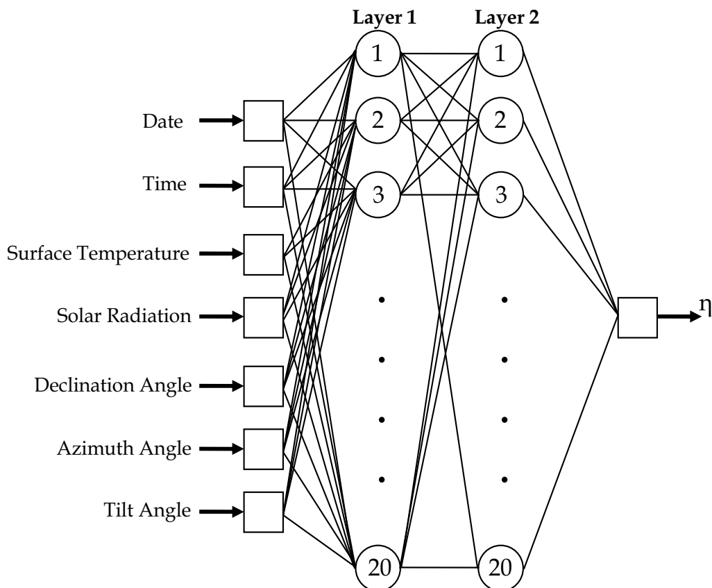
Fig. 9. ANN structure used by Sözen et al. (2008)
