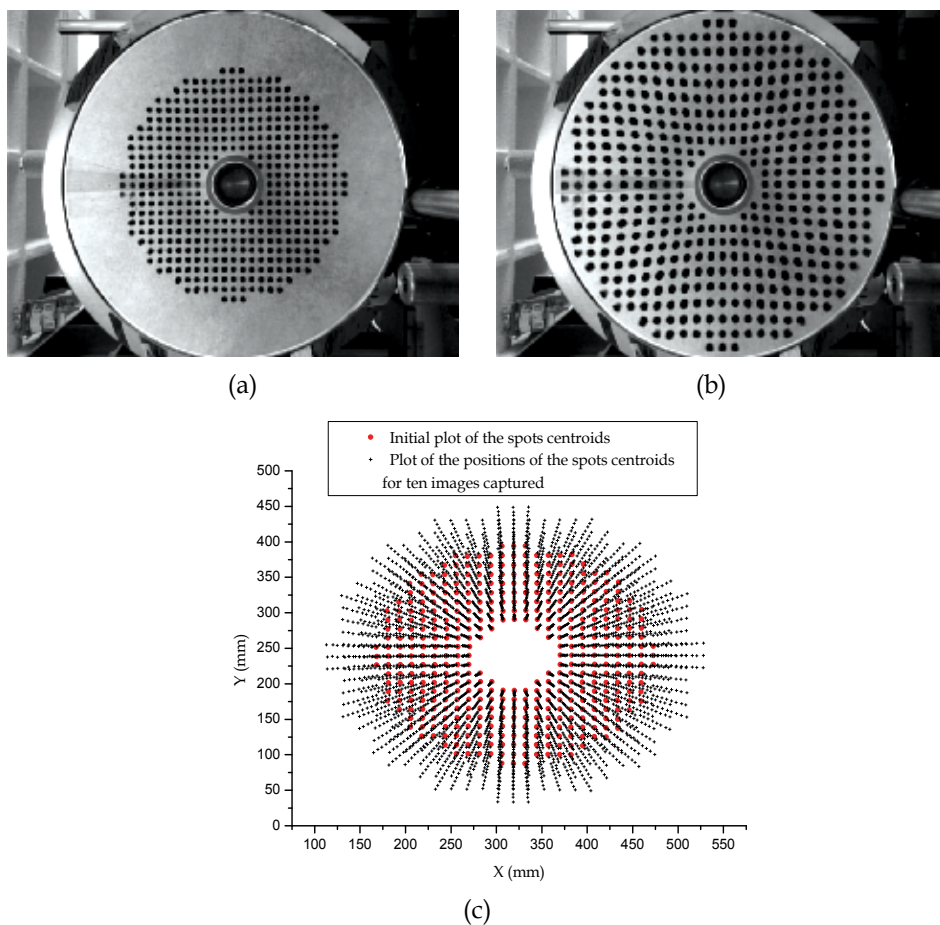
Fig. 5. a) Image of the screen at the initial position, b) Image of the screen at the final position, c) Plot of the centroid positions of the spots for ten images captured by using the point shifting method.
