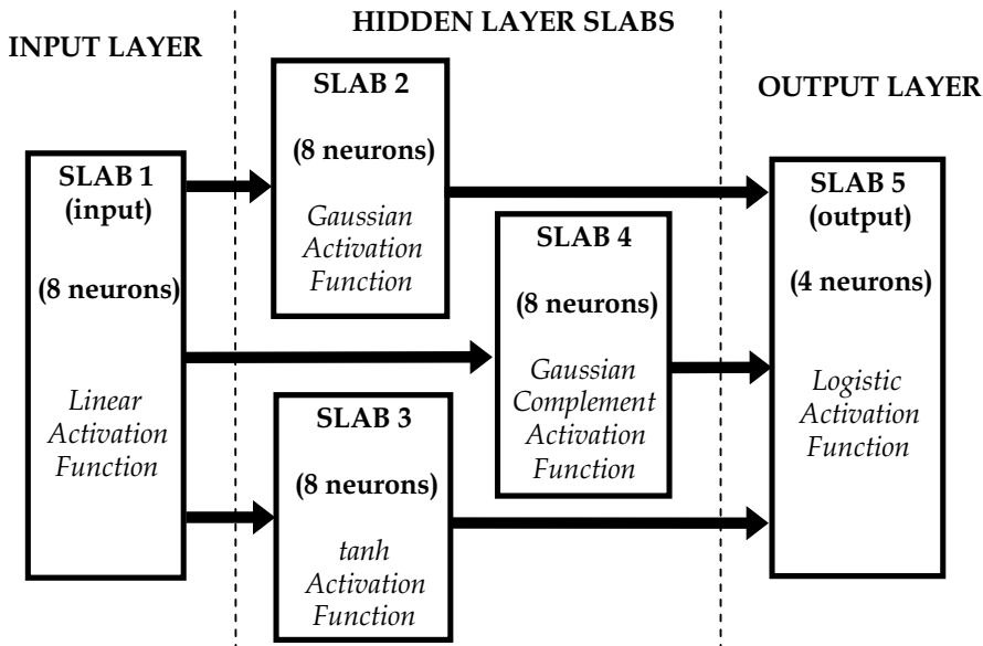
Fig. 7. The selected neural network architecture for modelling the transient heat-up response of a solar steam-generation system (Kalogirou et al., 1998)
