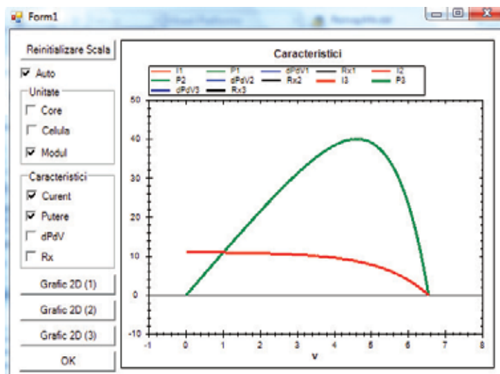
Fig. 16. The characteristic I(V) and P(V)
