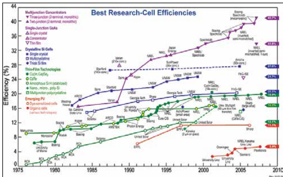
Fig. 6. Trends for efficiency of photovoltaic cells.
