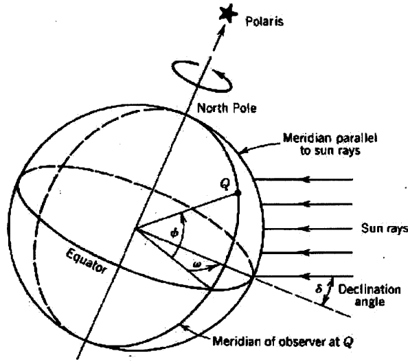
Fig. 4. Measurement of direction of sunrays, in the earth-centred coordinate systems
