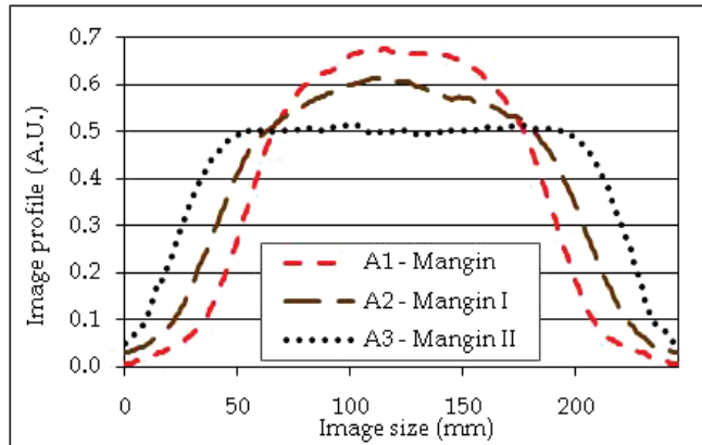
Fig. 4. Profiles of images for A1, A2, A3.
