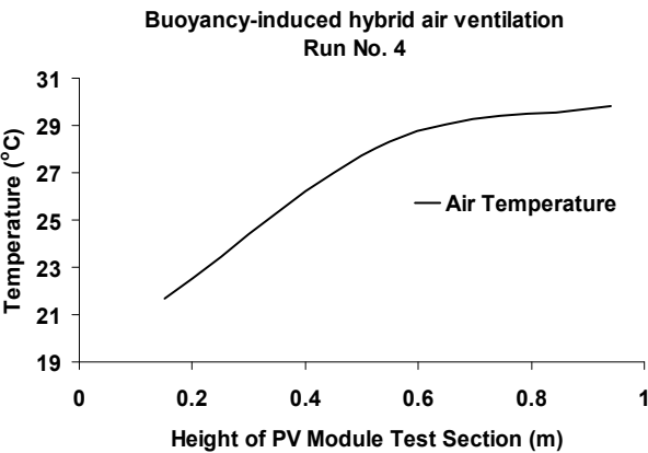
Fig. 6.(c) Temperature plot of air for buoyancy-induced hybrid ventilation with height of PV module test section
