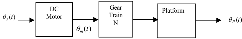
Fig. 3. Block diagram of the open-loop 3KW solar power platform
