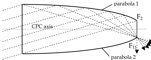
Fig. 3. Scheme of the edge ray method applied to a compound parabolic concentrator (CPC); the dotted arrows represents the incoming rays
