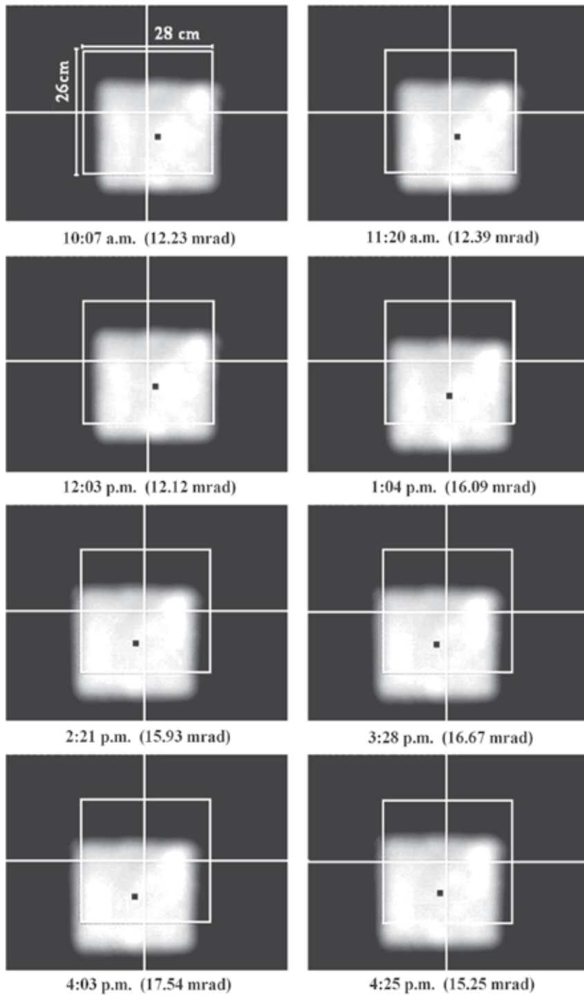
Fig. 13. The recorded solar images cast on the target of prototype solar concentrator using a CCD camera from 10:07 a.m. to 4:25 p.m. on 13 January 2009 with \phi = \lambda = \zeta = 0^\circ
