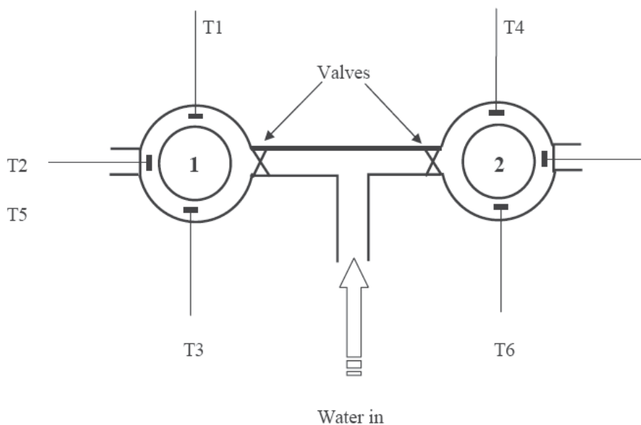
Fig. 5.2. Arrangement of the rings and thermocouples for solar water heater experiment.
