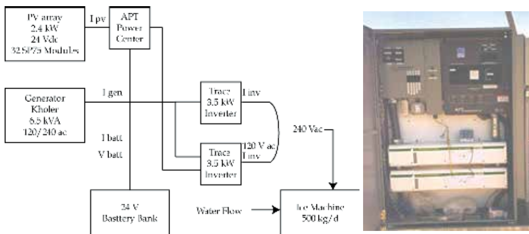
Fig. 10. Icemaker diagram and system Trace DR series inverters and APT power center with disconnects.
