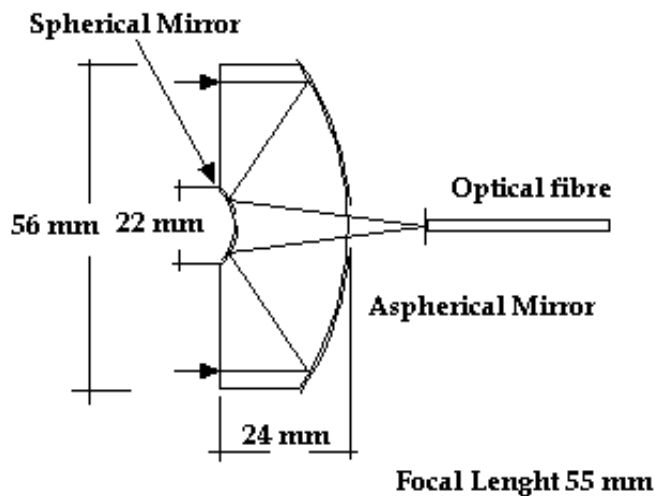
Fig. 9. Layout of CCM: collector C1.
