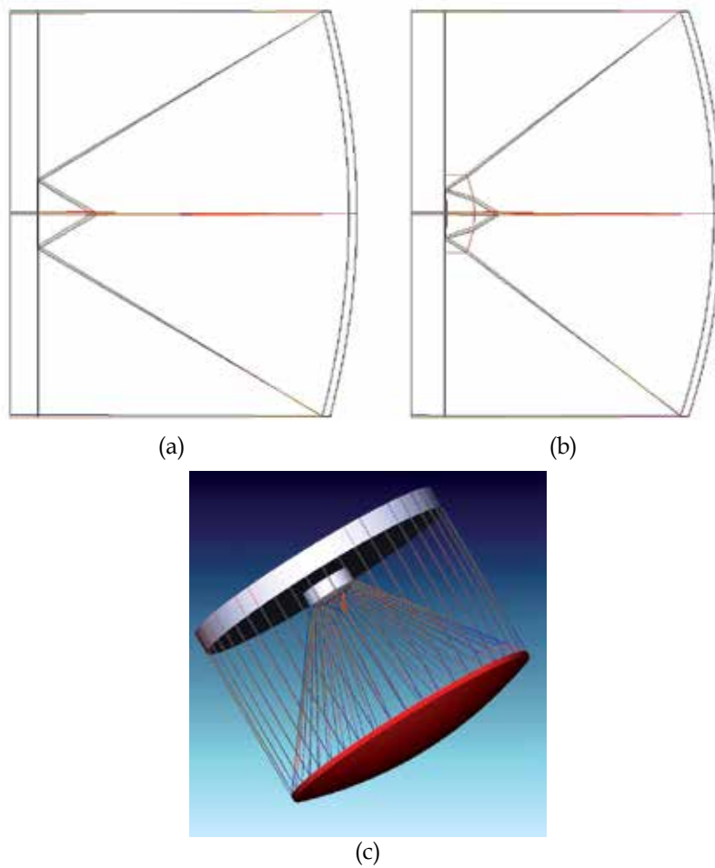
Fig. 7. (a) Zemax optical design of Parabolic B1. (b) Zemax optical design of Parabolic B2. (c) Zemax 3D model of Parabolic B2.
