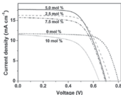
Fig. 12. Current - voltage curves of dye-sensitized solar cells based on the undoped and Nb-doped \text{TiO}_2 electrodes
