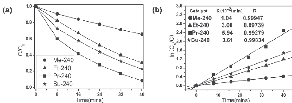
Fig. 4. MO photodegradation over samples under UV-light irradiation
