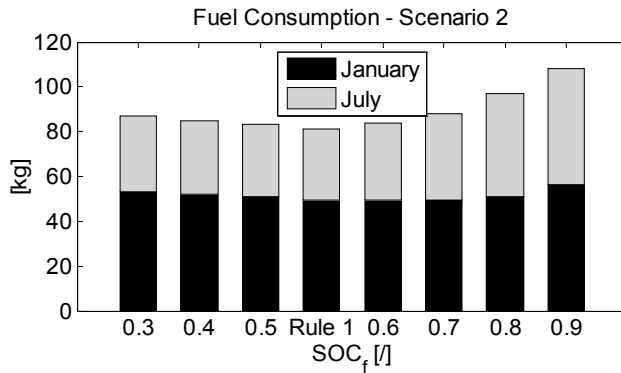
Fig. 13. Effects of optimized (Rule 1) and parametric choice of SOC on Fuel Consumption for a Hybrid Solar Vehicles (Los Angeles, January and July, 1988). \eta_{PV} = 0.19
