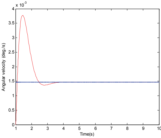
Fig. 14. Velocity response of tracker
