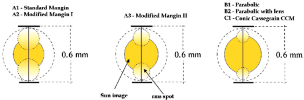
Fig. 1. Schematic view of images formed by the six collectors.
