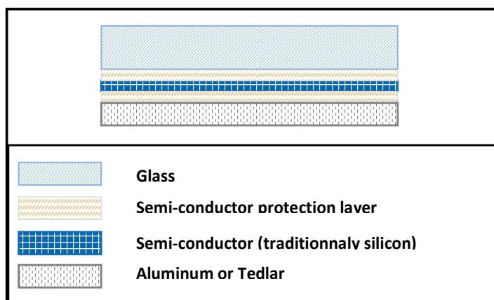
Fig. 3. Cross section of a typical photovoltaic panel
