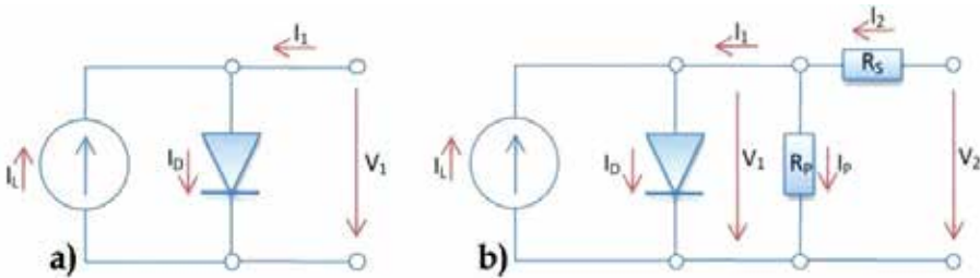
Fig. 3. Two equivalent circuits of PV cell: a) an ideal circuit, b) an equivalent circuit with serial and parallel resistive losses
