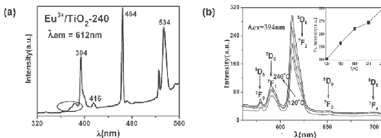
Fig. 8. (a) The excitation spectrum of \text{Eu}^{3+}/\text{TiO}_2 -240 ( \lambda_{\text{em}} = 612 \text{ nm} ), (b) the emission spectra ( \lambda_{\text{ex}} = 394 \text{ nm} ) of the \text{TiO}_2:\text{Eu}^{3+} samples, where their maximum emission ( \lambda_{\text{em}} = 612 \text{ nm} ) intensities at 612 nm in the inset
