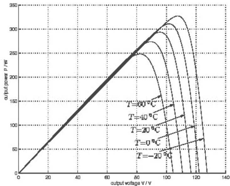
Fig. 3. P-V characteristics of a photovoltaic panel for different values of temperature T at irradiance of 1000 \text{W/m}^2 .
