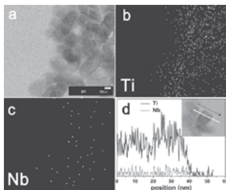
Fig. 11. (a) Bright-field STEM image of 5.0 mol% Nb-doped \text{TiO}_2 ; (b, c) the corresponding elemental mapping of Ti (b) and Nb (c); (d) line-scanning analysis across the nanoparticles indicated by the line as shown in the inset
