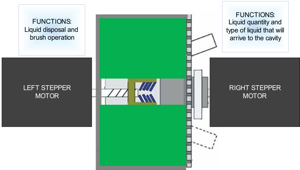
Fig. 2. Sensor simplest diagram design and motor functions
