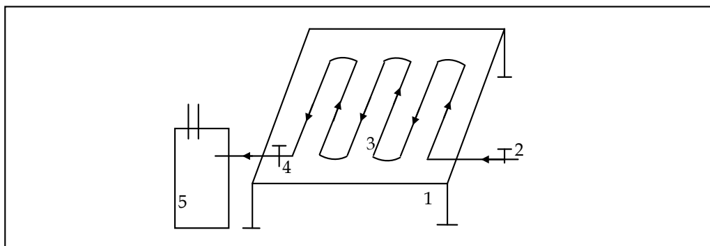
Fig. 12. Collector with pipes from an old refrigerator.
