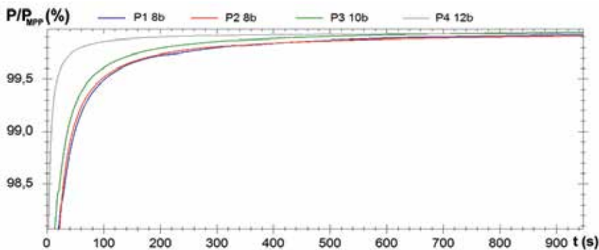
Fig. 17. The algorithm behavior: energy output (Algorithm result for MPP calculation using dP/dV=0 relation)
