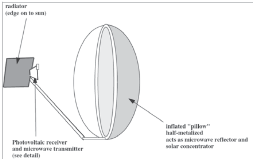
Fig. 20. Individual concentrator/PV/solid-state-transmitter/parabolic reflector element (Landis, 2004)
