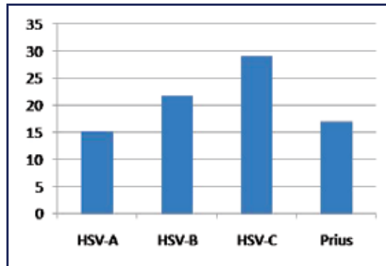
Fig. 12. Fuel Economy (km/l) on ECE Cycle - HSV vs. Toyota Prius. A – actual prototype. B – PV eff.=18% - Batt.=75 Ah. C – B+ 20% weight off – Lithium-Ion Batt.
