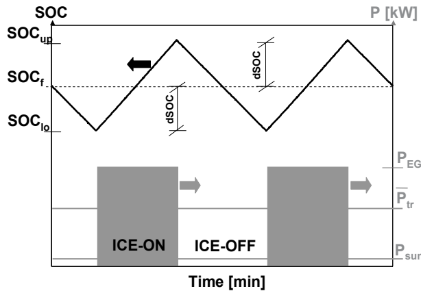
Fig. 14. Schematic representation of the rule-based control strategy for quasi-optimal energy management of a series HSV powertrain.
