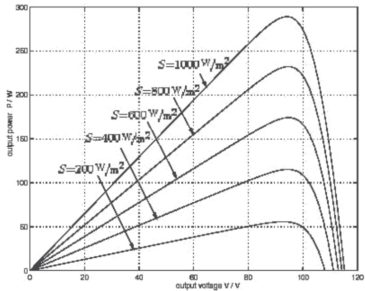
Fig. 2. P-V characteristics of a photovoltaic panel for different values of irradiance S at a temperature of 25 °C.
