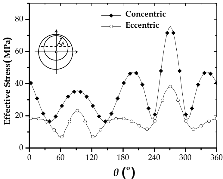
Fig. 13. Thermal stress profiles along the internal circumference at the outlet section for both the concentric and eccentric tube receivers.
