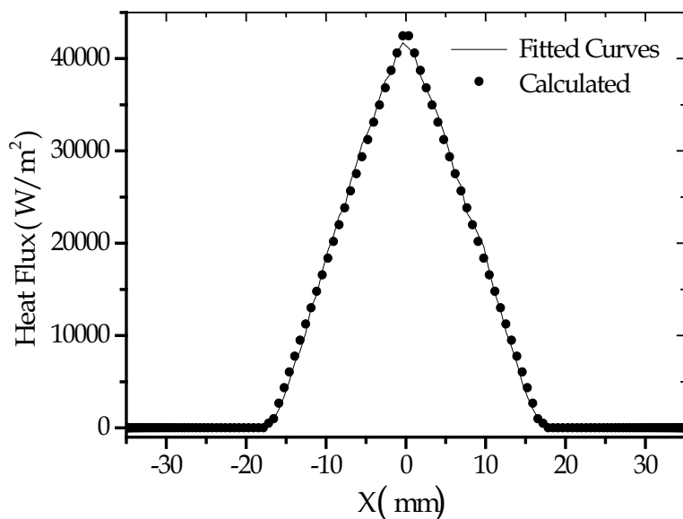
Fig. 3. Calculated heat flux distribution on the bottom half periphery of tube receiver and the fitted function curves.
