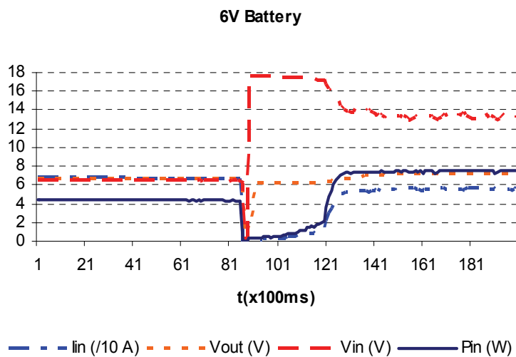
Fig. 11. Experimental results of the P&O MPPT algorithm power with four 6V batteries (first phase direct connection and second phase using the developed board).
