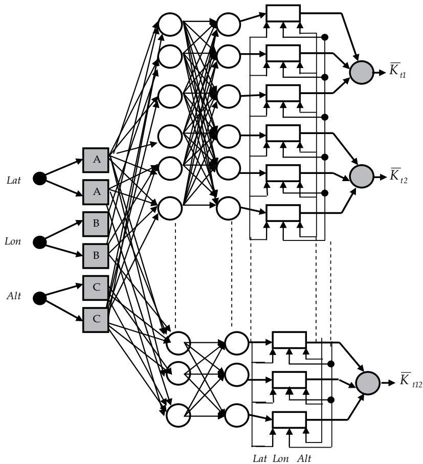
Fig. 11. The proposed ANFIS-based prediction for monthly clearness index proposed by Mellit et al. (2008)
