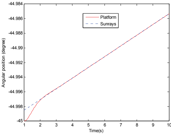
Fig. 13. Polar axis tracking of angle of sunrays
