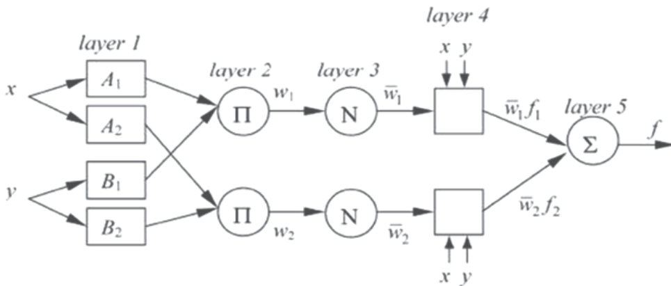
Fig. 3. ANFIS architecture
