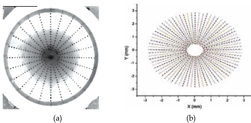
Fig. 6. a) Image of the screen at the initial position, b) Plot of the position of the centroids for the spots at each rotation step of the test surface.
