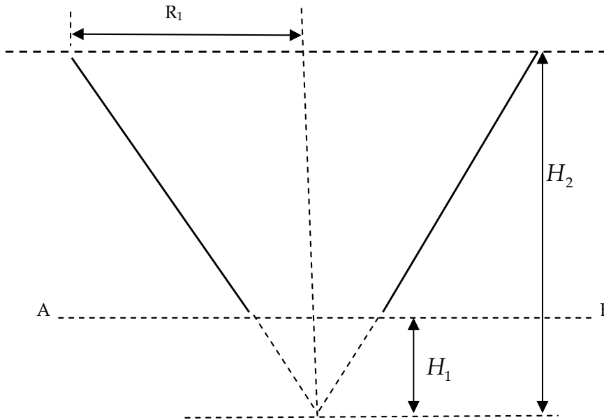
Fig. 3.1. Schematic diagram of a cone showing the distance H_1 from the apex to the cross section AB (absorber area) and the distance H_2 from the apex to the collector area
