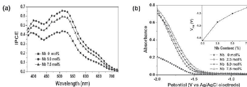
Fig. 13. (a) Action spectra of the dye-sensitized solar cells based on the undoped and Nb-doped \text{TiO}_2 electrodes. (b) Optical absorbance at 870 nm of undoped and Nb-doped \text{TiO}_2 films measured as a function of applied potential. Inset shows the flat-band potential of the samples as a function of the Nb contents
