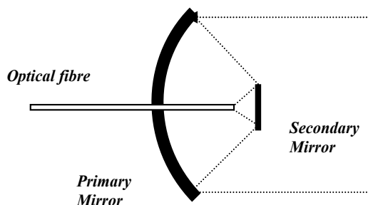
Fig. 6. Fibre position for Mangin and Parabolic collectors.
