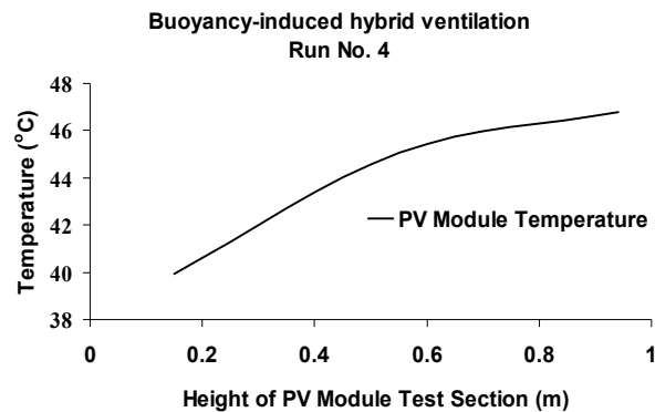
Fig. 6.(a) Temperature plot of PV module for buoyancy-induced hybrid ventilation with height of PV module test section
