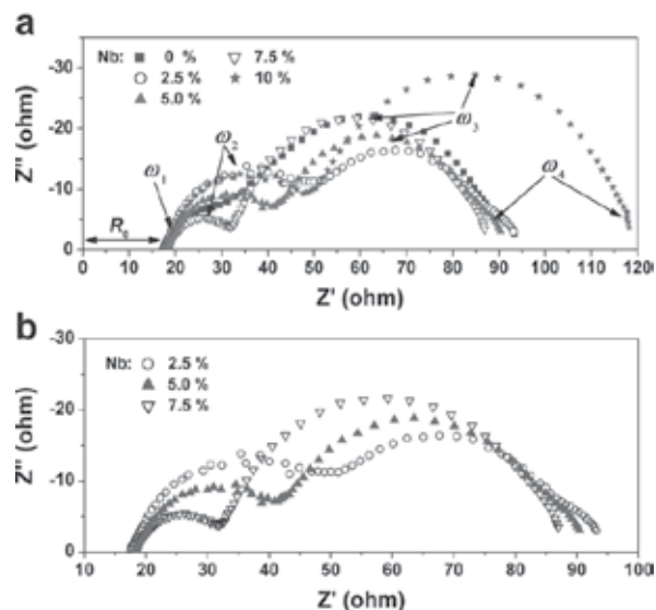
Fig. 15. Electrochemical impedance spectra of dye-sensitized solar cells based on the undoped and Nb-doped \text{TiO}_2 electrodes
