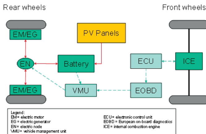
Fig. 19. Scheme of a system to upgrade a conventional car to Mild Hybrid Solar Vehicle.
