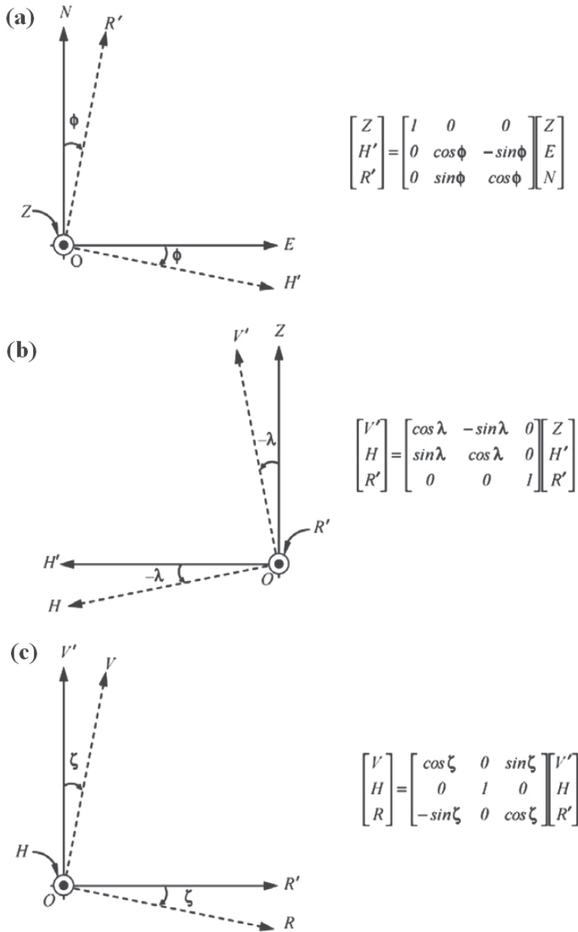
Fig. 6. The diagram shows the process of how the collector-centre frame is tilted step-by-step relative to the earth-surface frame, where OV' , OH' and OR' axes represent the intermediate position for OV , OH and OR axes, respectively. (a) The first tilted angle, +\phi , is a rotational angle about OZ -axis in clockwise direction in the first step of coordinate transformation
