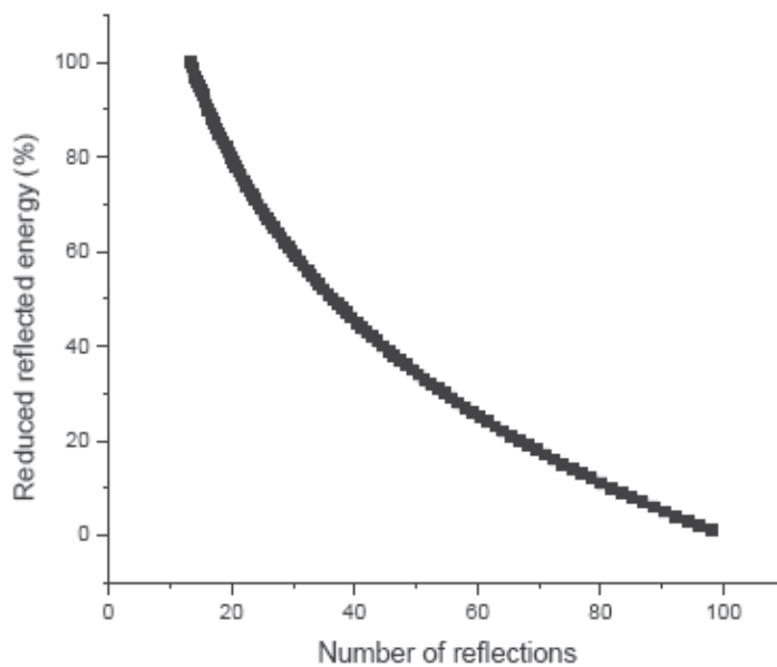
Fig. 5.3. Reflected energy versus the number of reflections.
