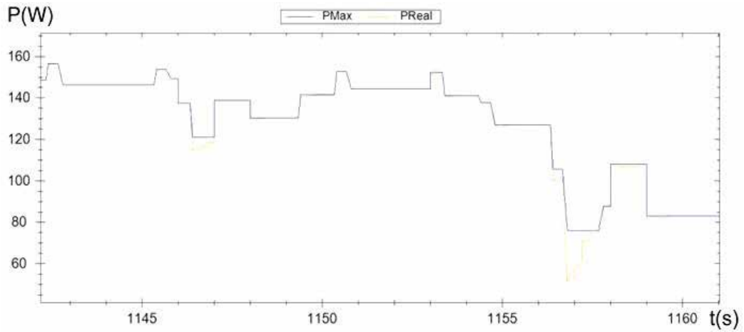
Fig. 20. Algorithm result for MPP's calculation with three points
