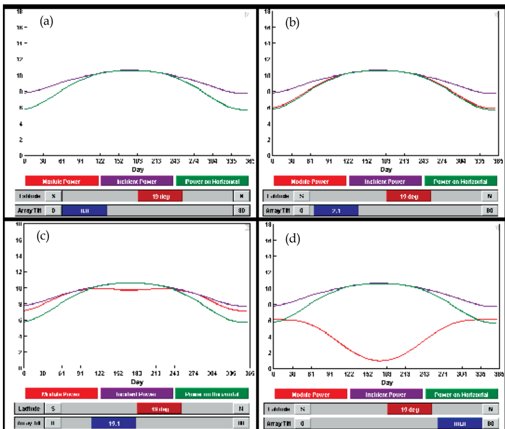
Fig. 5. Tilting in power production at (a) 0°, (b) 2.1°, (c) 19.1° and (d) 80° throughout all the year ( http://energyworksus.com/solar_power_incident_angle.html ).
