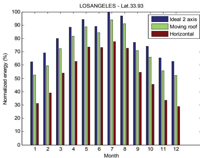
Fig. 18. Energy collected with various options of solar roof (Los Angeles, 1988)
