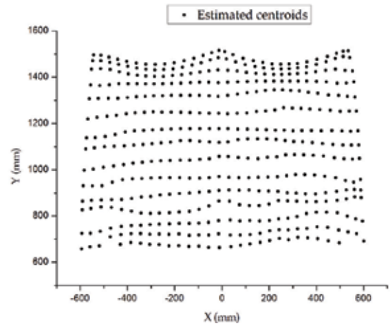
Fig. 10. Plot of the centroid positions for some spots of the flat null screen.
