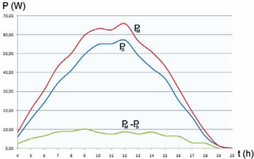
Fig. 24. Power transferred into batteries in a clear summer day
