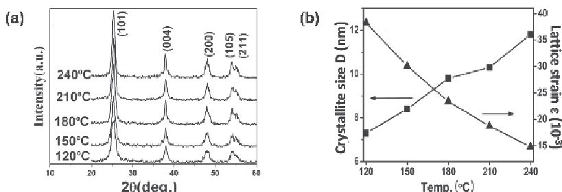
Fig. 6. (a) XRD patterns and (b) the corresponding crystallite size D and lattice strain \epsilon for the \text{TiO}_2:\text{Eu} nanoparticles on the hydrothermal temperature
