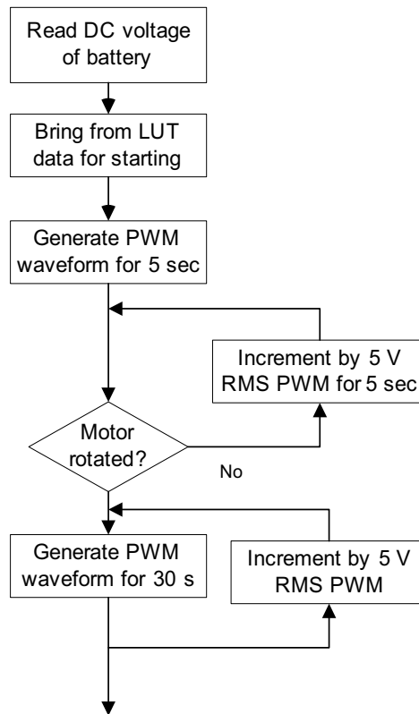
Fig. 11. Block diagram of the motor starter
