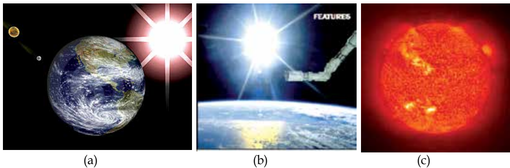
Fig. 16. Impressive views of the Sun: (a) The Sun, the Earth and the Moon, (b) The Sun as seen from Space Shuttle Endeavour (c) and the Sun observed surface, all of which emphasize its tremendous potential as an inexhaustible source of energy ( http://www.google.com.my/imglanding ).
