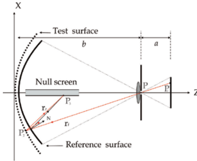
Fig. 4. Approximated normals.
