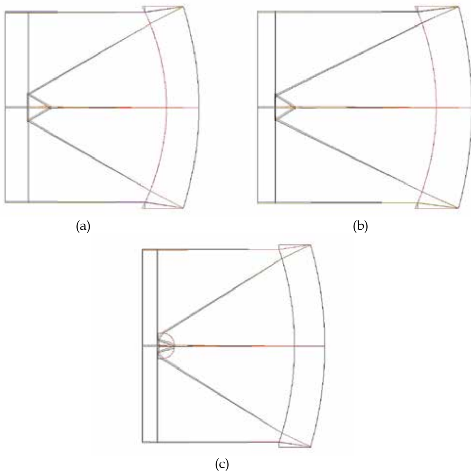
Fig. 3. (a) Zemax optical design of Mangin A1 (b) Zemax optical design of Mangin A2 (c) Zemax optical design of Mangin A3
