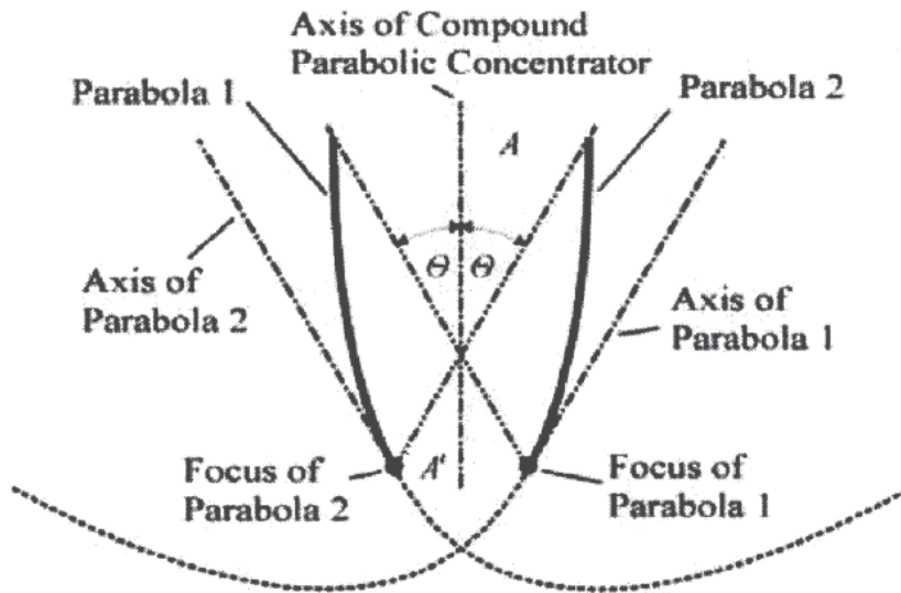
Fig. 4.1. Compound parabolic concentrator (CPC).
