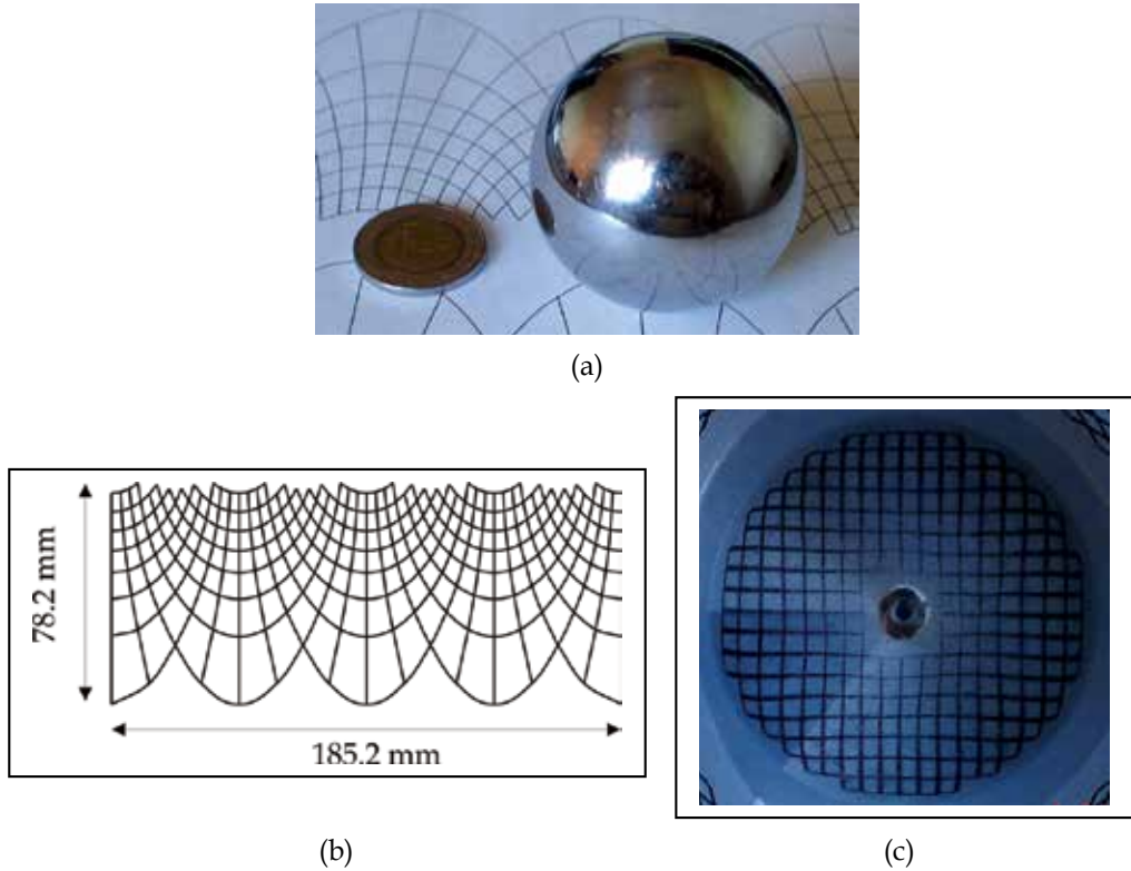
Fig. 3. a) Spherical surface (steel ball), b) flat printed null screen with grid lines for qualitative testing, and c) the resultant image of the screen after reflection on the test surface.
