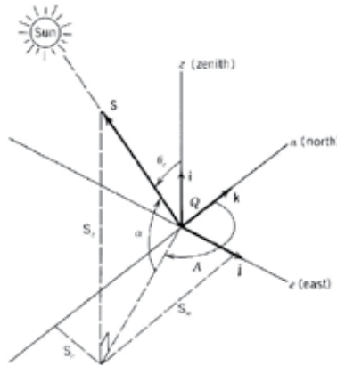
Fig. 7. Collector-centred coordinate systems and its relationship to the earth-centred coordinates at the observer location
