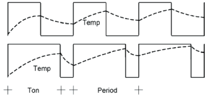
Fig. 12. Duty cycle and its effect on temperature increase.
