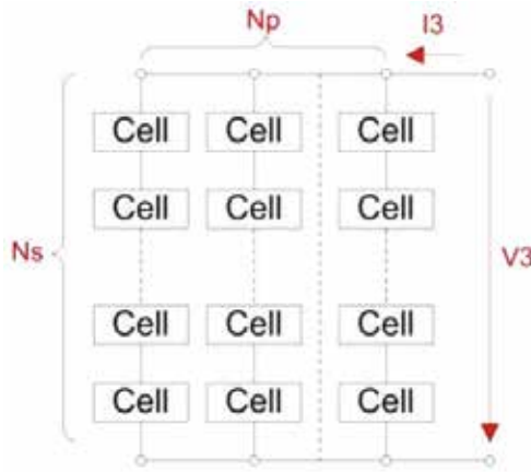
Fig. 4. A photovoltaic panel, as a matrix of N_S \times N_P cells
