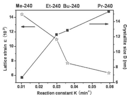
Fig. 5. The effect of the crystallinity on the reaction constant K
