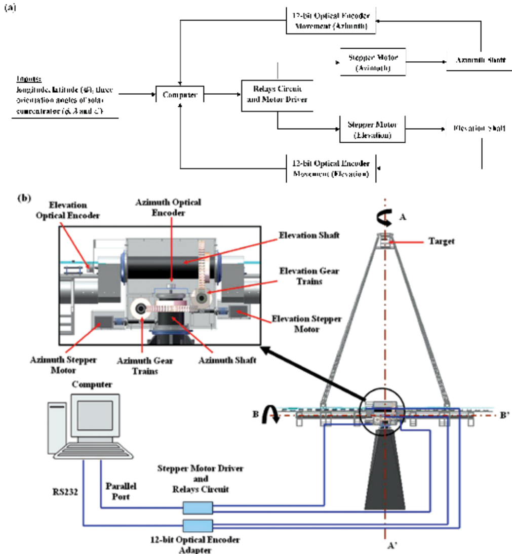
Fig. 11. (a) Block diagram to show the complete open-loop feedback system of the solar concentrator. (b) Schematic diagram to show the detail of the open-loop sun-tracking system of the prototype planar concentrator where AA' is azimuth-axis and BB' is elevation-axis.
