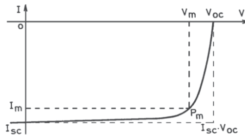
Fig. 2. The parameters of I - V cell illumination characteristic
