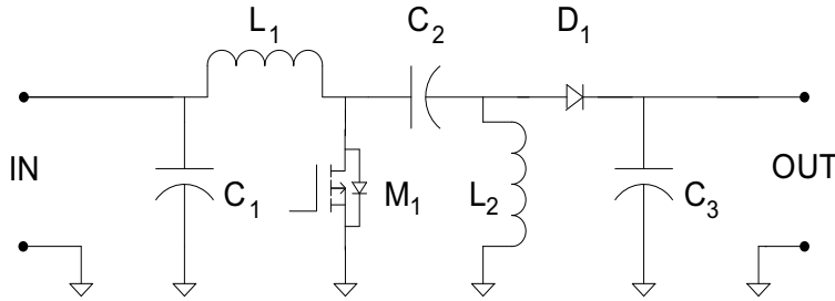
Fig. 4. SEPIC DC/DC converter circuit.
