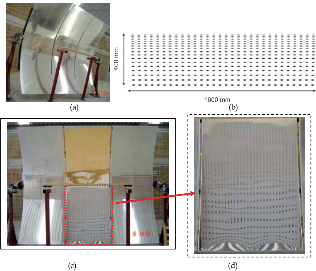
Fig. 9. a) PTSC component, b) flat printed null screen with drop shaped spots for quantitative testing (400x1600 mm), c) image of the screen after reflection on the test area surface, and d) detail of the image.
