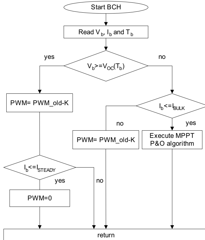
Fig. 8. Battery charging algorithm with two main stages.
