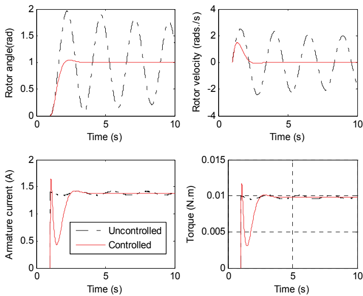
Fig. 12. Comparison of dynamics for controlled and uncontrolled platform
