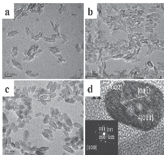
Fig. 7. The TEM images of (a) \text{Eu}^{3+}/\text{TiO}_2 -120, (b) \text{Eu}^{3+}/\text{TiO}_2 -180, (c) \text{Eu}^{3+}/\text{TiO}_2 -240, (d) HRTEM of \text{Eu}^{3+}/\text{TiO}_2 -240, Fast-Fourier Transformed diffractogram of \text{Eu}^{3+}/\text{TiO}_2 -240 (inset)
