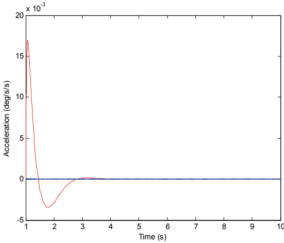
Fig. 15. Comparison of acceleration
