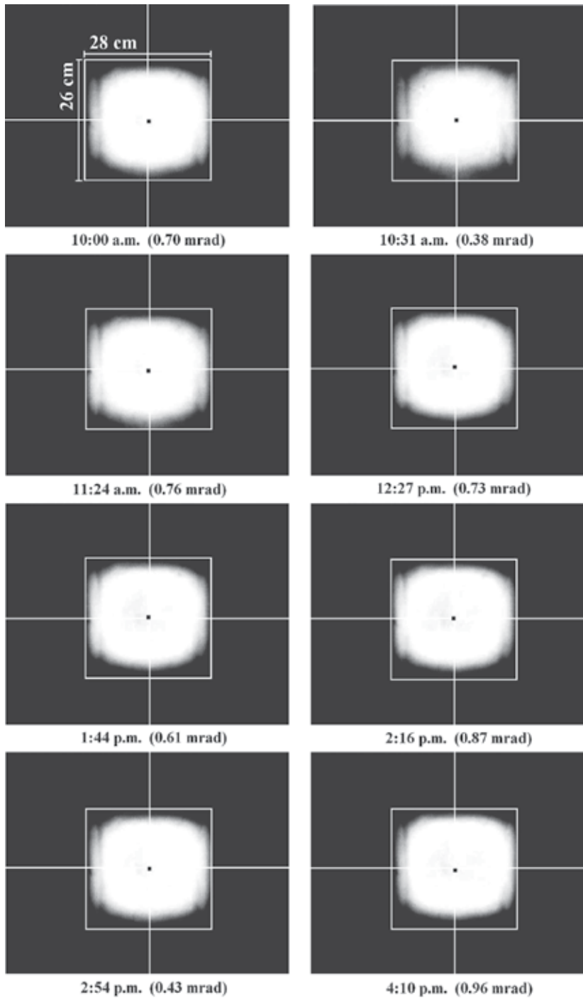
Fig. 17. The recorded solar images on the target of prototype solar concentrator using a CCD camera from 10:00 a.m. to 4:10 p.m. on 6 August 2009 with \phi = -0.1^\circ , \lambda = 0^\circ , and \zeta = -0.5^\circ and including the step count of stepper motor, 1.64 \times 10^{-4}^\circ/\text{step}
