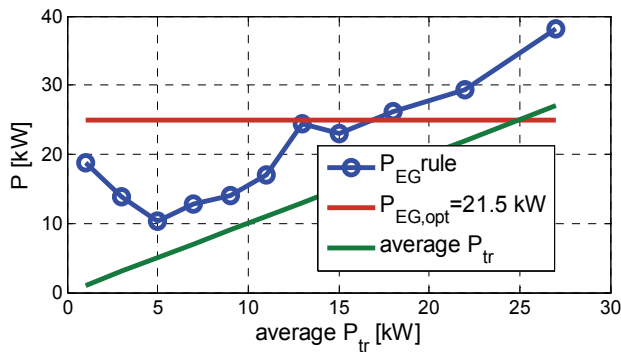
Fig. 16. Optimal generator power vs. average vehicle power for a hybrid electric vehicles with series structure.
