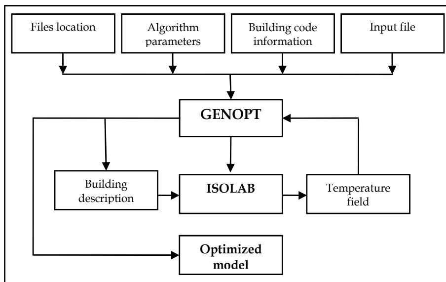
Fig. 14. Synoptic of the coupling of the building simulation code ISOLAB with GENOPT.
