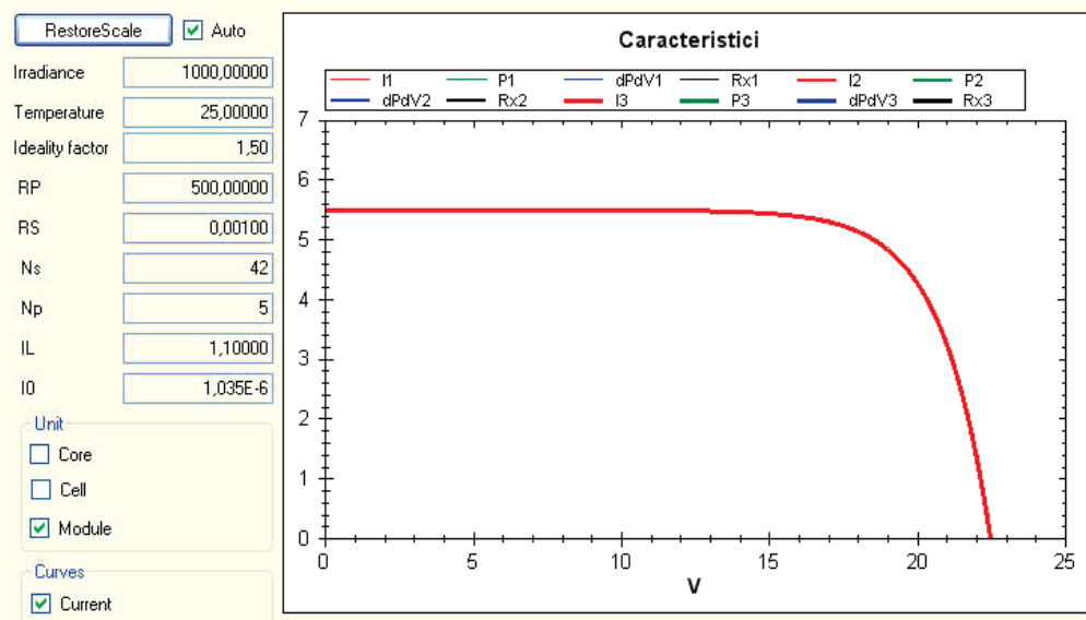
Fig. 26. The I(V) characteristic and model parameters of photovoltaic panel
