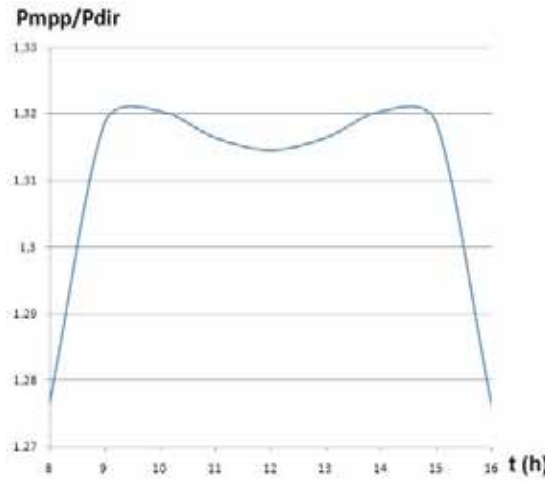
Fig. 8. Power ratio under winter conditions
