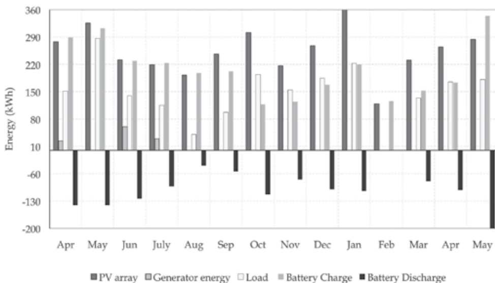
Fig. 11. First year system energy performance.
