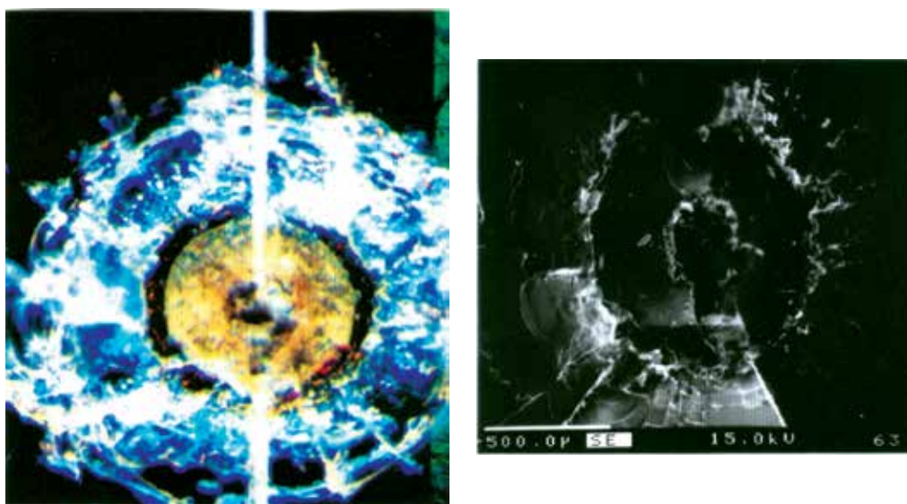
Fig. 8. shows a photo and a secondary electron image (of a scanning electron microscope) of a particle impact on a solar cell sample of the Hubble Space Telescope (Heiss & Stadermann, 1997)
