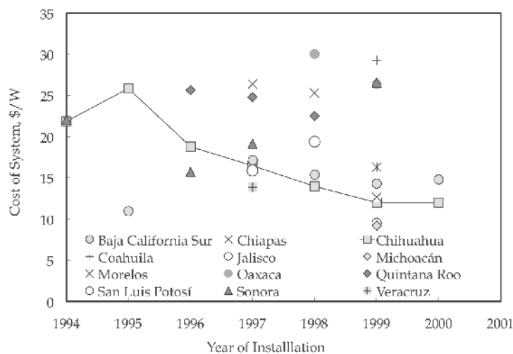
Fig. 7. Average cost of PV water systems by year and by state.
