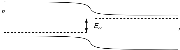
Fig. 8. Schematic band diagram of an illuminated p-n junction of a cell in open circuit conditions
