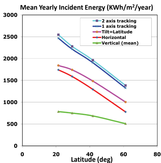
Fig. 17. Effects of panel position and latitude on incident energy
