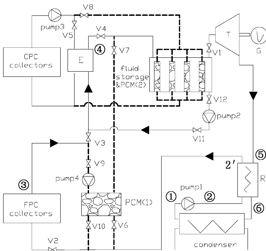
Fig. 1. Low-temperature solar thermal electric generation with two-stage collectors and heat storage units
