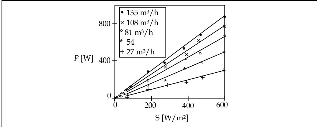
Fig. 6. Collector power versus absorbed radiation, parameterized by the flow rate
