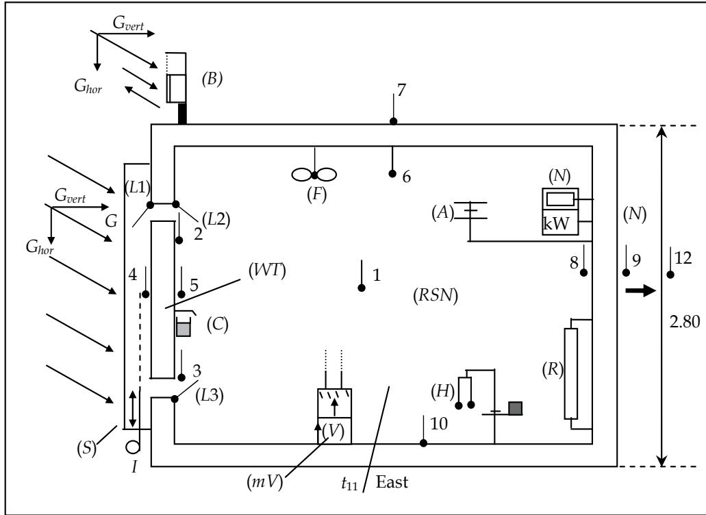
Fig. 9. Room with Trombe wall and measuring points.
