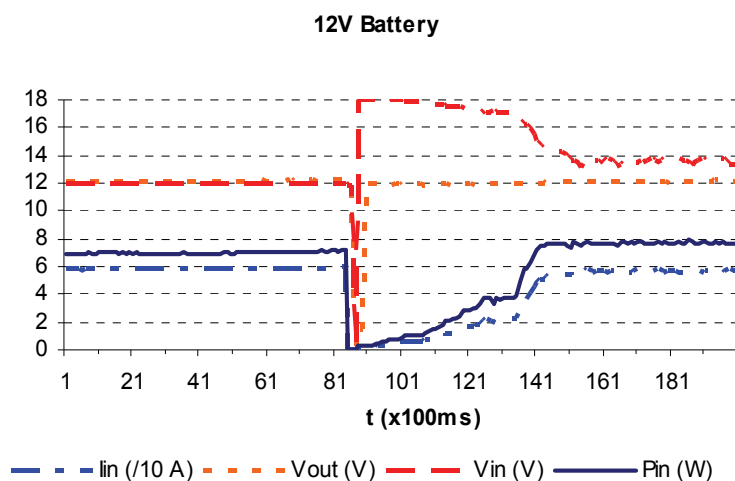
Fig. 10. Experimental results of the P&O MPPT algorithm power with a 12V battery (first phase direct connection and second phase using the developed board).
