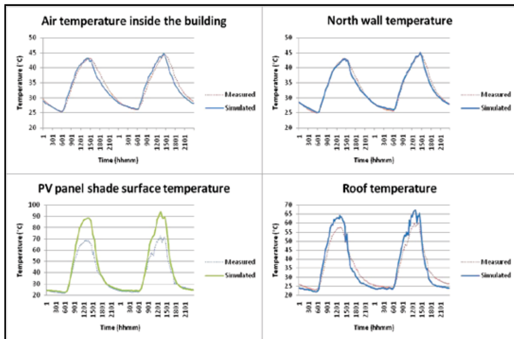
Fig. 11. Temperatures of the PV installation with a confined air layer.
