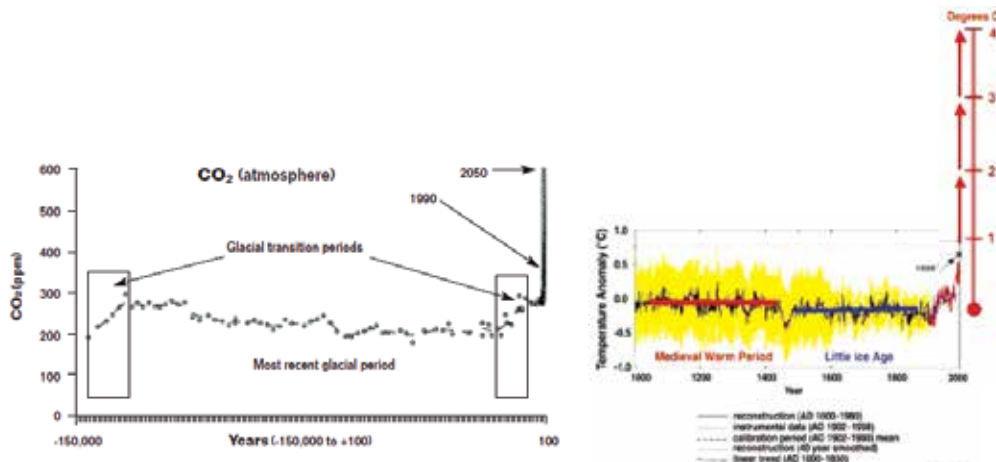
Fig. 6. Estimates of CO 2 concentrations for the last 150,000 years with a projection to A.D. 2050 based on present-day rates of emission. The corresponding temperature anomaly is shown on the right hand side (From Walker, Keim and Arndt, 2010).
