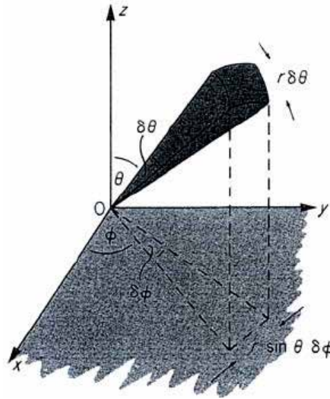
Fig. 3.2. The cone subtends angles \delta\theta and \delta\phi at the origin, and its cross sectional area at a distance r from the apex is r^2 \sin \theta \delta\theta \delta\phi . [1].
