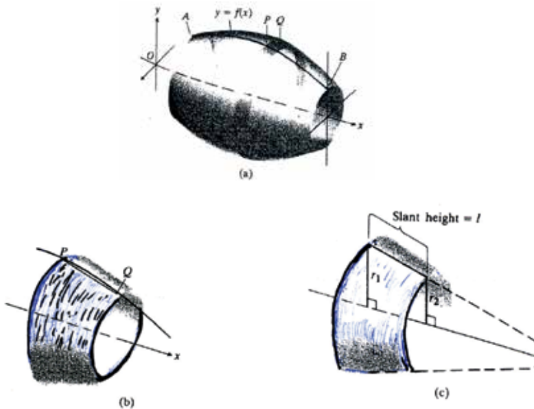
Fig. 3.3. Generation of a cone from a curve AB by using frustrums as parts of the cone.
