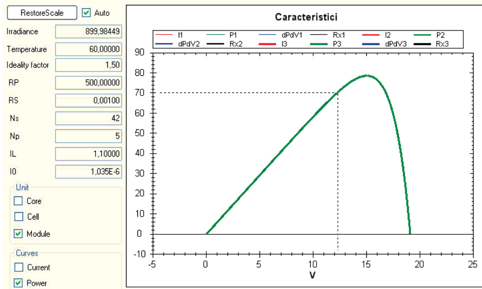
Fig. 27. The P(V) characteristic of the panel model, at T=60^{\circ}\text{C} and G=900\text{W}/\text{m}^2
