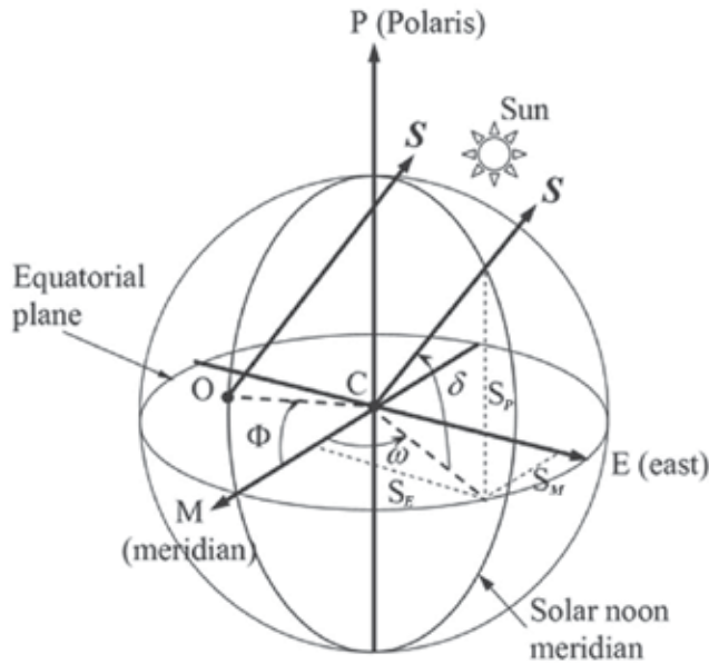
Fig. 2. The sun's position vector relative to the earth-centre frame. In the earth-centre frame, CM, CE and CP represent three orthogonal axes from the centre of the earth pointing towards meridian, east and Polaris, respectively
