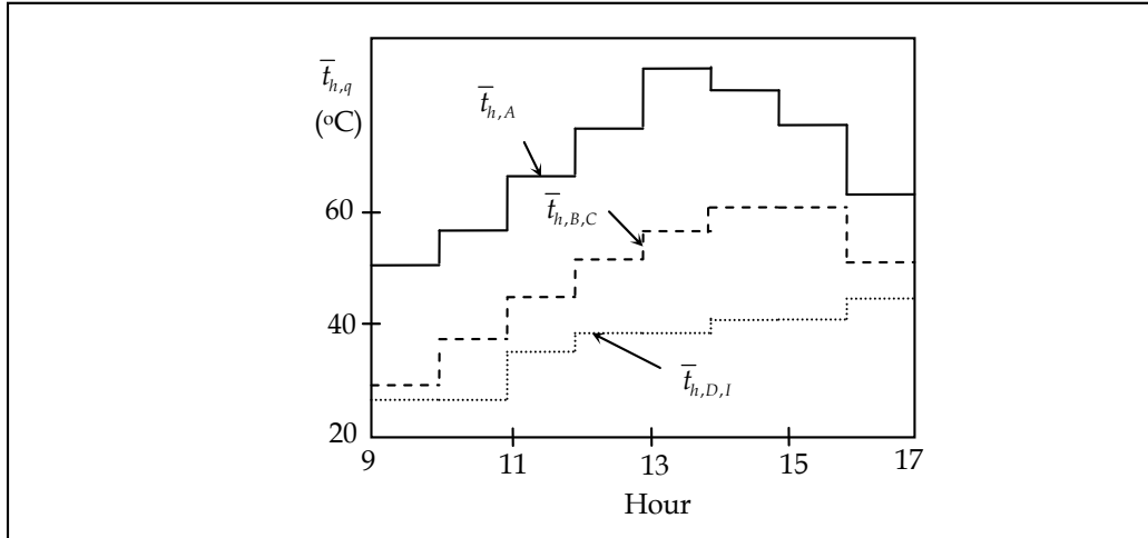
Fig. 15. Hourly averaged temperatures at points A, B, C, D and I.
