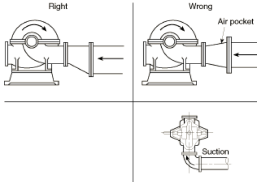
fig-20. Right and wrong pump suctions.
