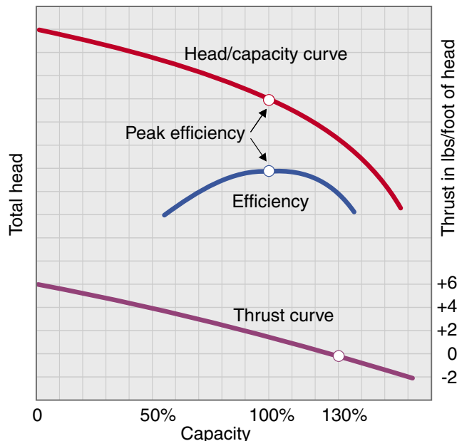
Figure 2 – Typical thrust curve.
