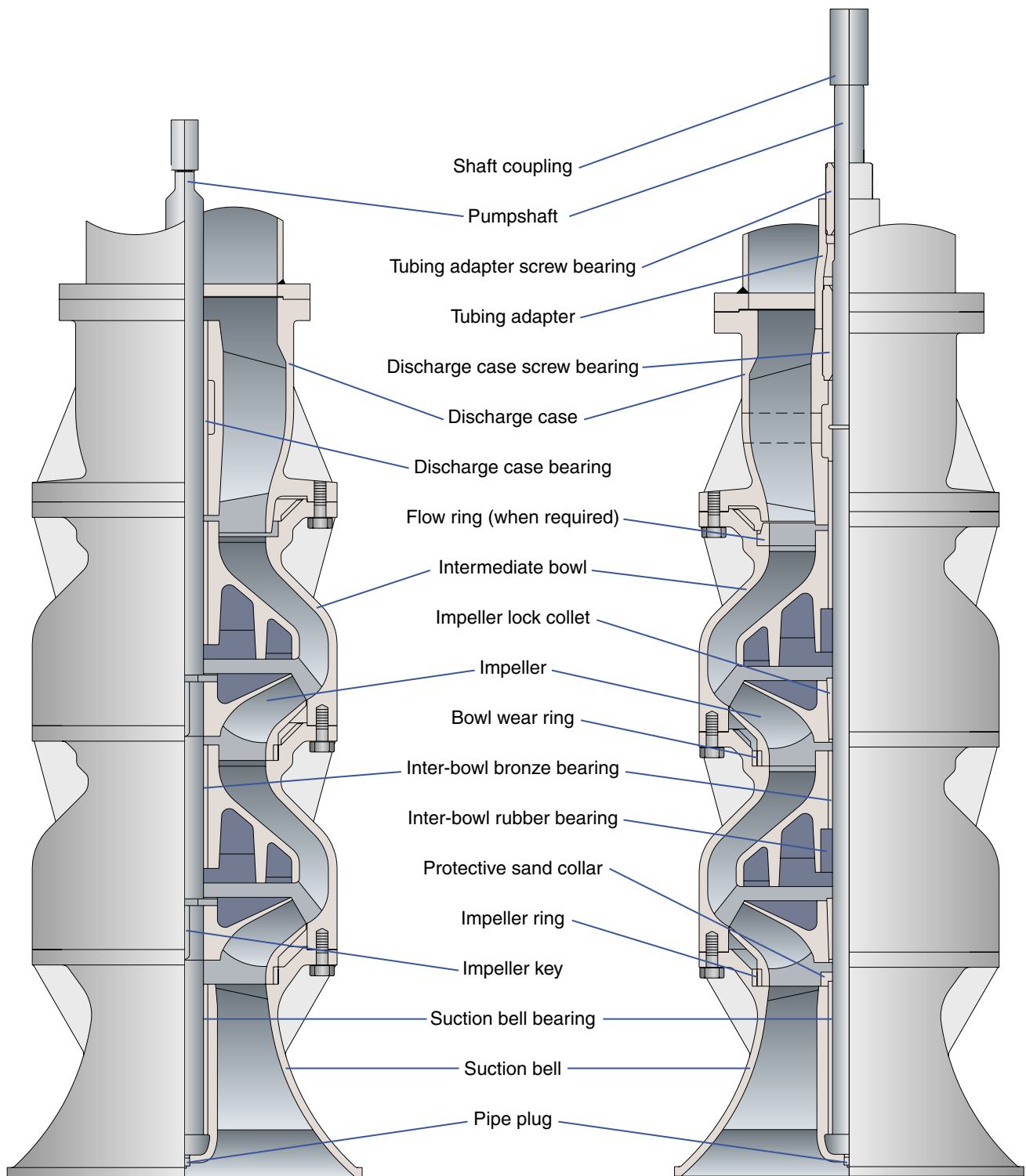
Product lubricated model with closed impellers, single bearings and keyed impeller construction
