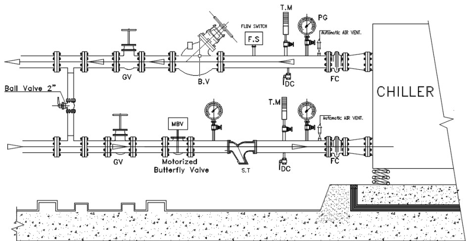
TYP. CHILLER CONNECTION DETAIL
