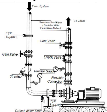
Chilled Water Pump Hook Up Details ( N.T.S. )
