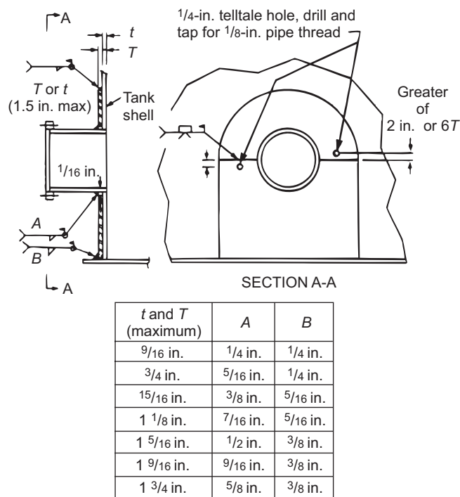
Figure 9.8—Typical Details for Addition of “Tombstone” Shape Reinforcing Plate to Existing Shell Penetration
