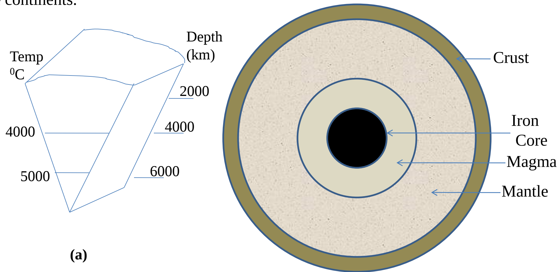
Fig: (a) Temperature distribution along depth of earth and (b) different layers of earth along depth
