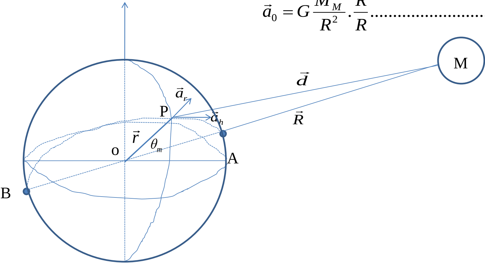
Fig: Moon and Earth system
