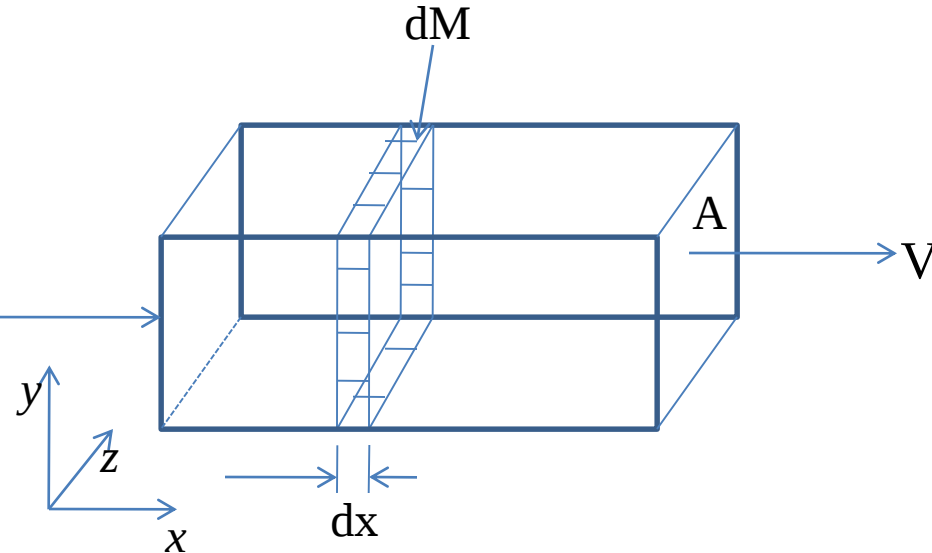
Fig: Derivation of power density
