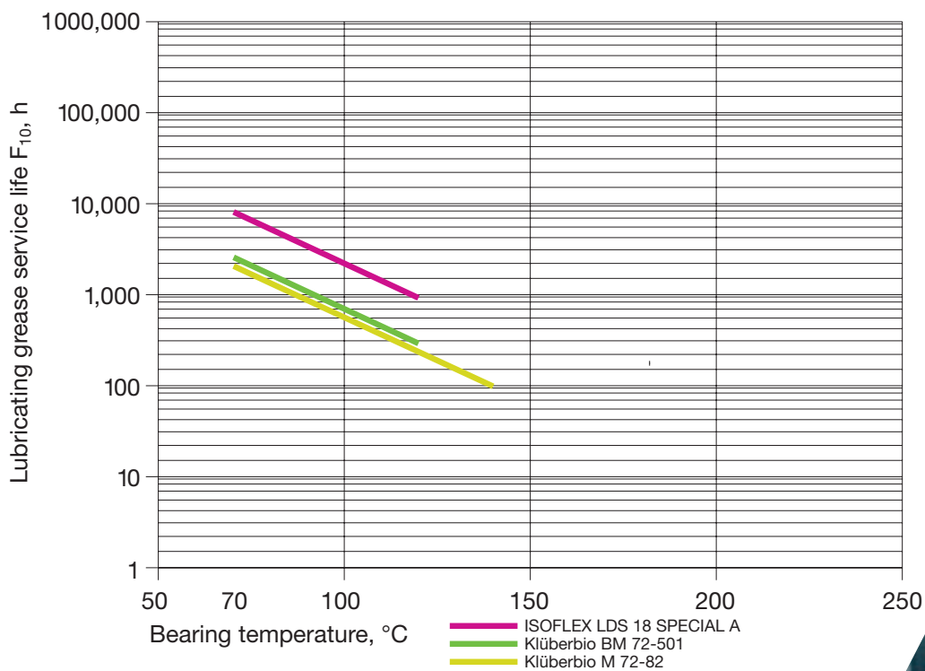
Lubricating grease service life as a function of temperature
