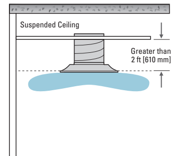
Figure 25: Ceiling diffuser free space mounting
