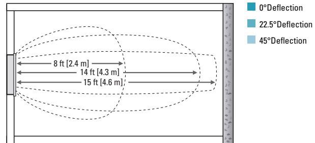
Figure 27: Plan view of spread vs. throw
