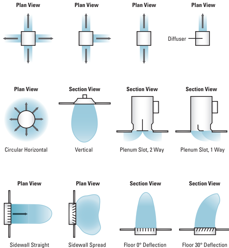
Figure 4: Air patterns
