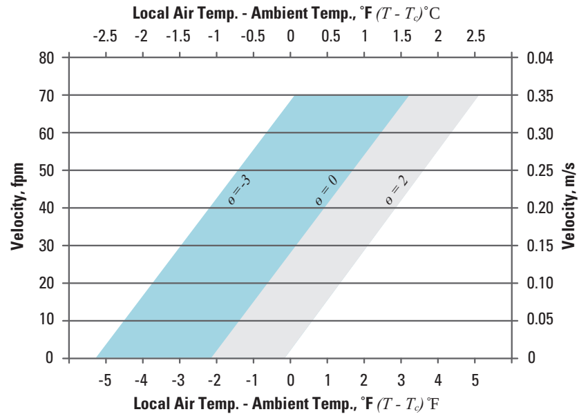
Figure 30: Comfort criteria - draft temperature
