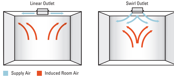
Figure 34: Low temperature air outlets
