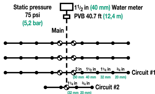
Figure 65: Piping plan
