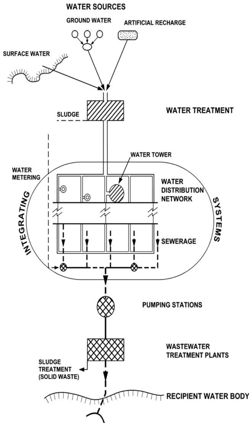
Figure 3.1 Schematic of integrated water supply and sewage systems.
