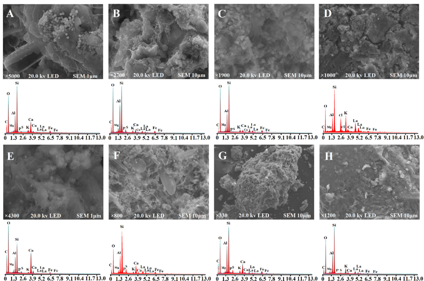
Figure 3. SEM images and spectra of chemical composition of Control (A), LAA (B), LAA+M (C), Original LAA (D), M (E), LMB (F), LMB+M (G) and Original LMB (H). Original LAA and Original LMB are substances that are not mixed with sediments respectively.
