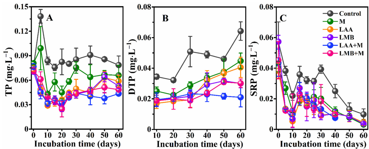
Figure 1. The changes of TP, DTP, and SRP concentrations in the overlying water of the six treatments during the experiment. Vertical bars indicate standard deviation. (A–C) represent TP, DTP, and SRP in the overlying water, respectively.
