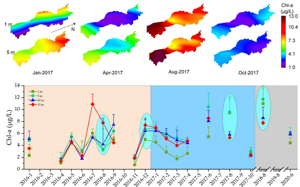
Figure 6. Spatiotemporal changes in Chl-a.
