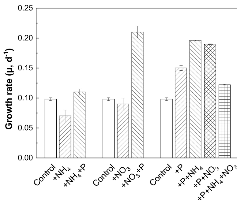
Figure 5. Comprehensive effects of NH 4 -N, NO 3 -N, and SRP on phytoplankton growth.
