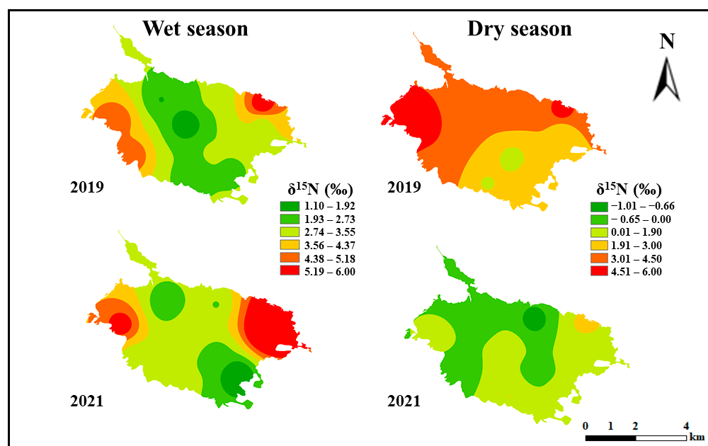
Figure 6. Temporal and spatial variation of nitrogen stable isotope in wet season and dry season of Caohai Lake.
