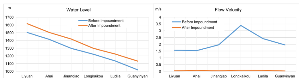
Figure 6. Changes in water level in front of dams and velocity in reservoirs after cascade hydropower development on the middle reaches of the Jinsha River.
