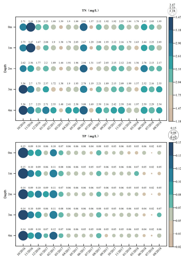
Figure 7. The change in TN and TP concentration in Lake Yilong from October 2016 to August 2018.
