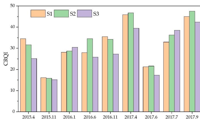
Figure 8. Cyanophyte relative quantity index from 2015–2017 in Lake Yangzong. Note: The ordinate value in the figure was calculated using the formula CRQI = [PC]/[Chl-a] , and its unit is cells/ \mu g .
