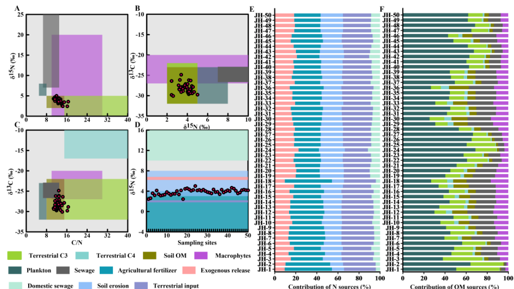
Figure 3. Scatterplots of \delta^{15}\text{N}/\text{C/N} ratios (A), \delta^{15}\text{N}/\delta^{13}\text{C} (B) and \delta^{13}\text{C}/\text{C/N} ratios (C), site-special range of \delta^{15}\text{N} (D) (isotopes boundary data from [25,26]), as well as the contribution of N (E) and organic matter sources (F).
