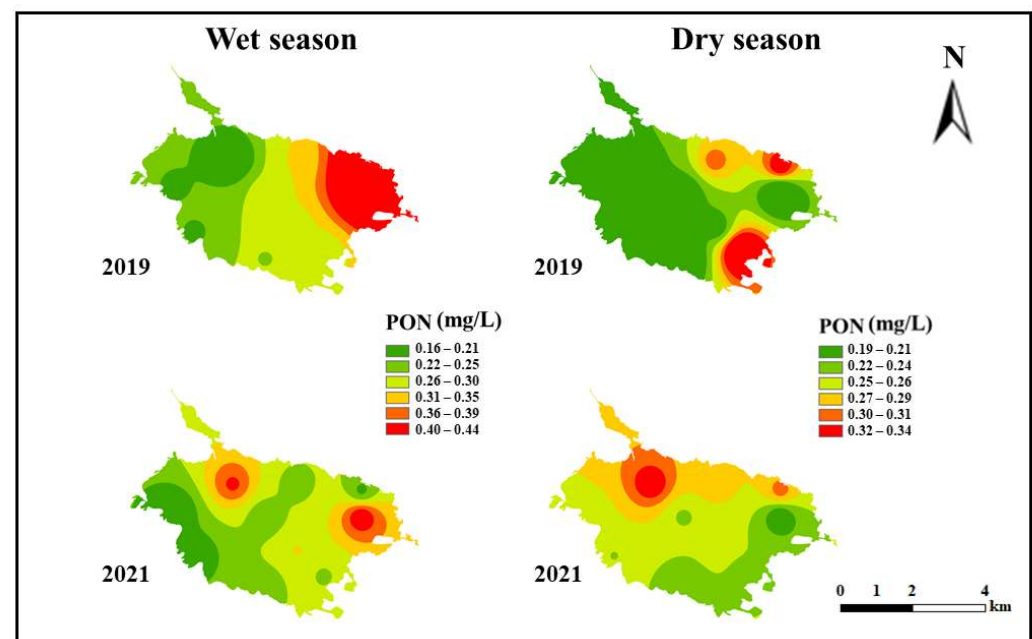
Figure 4. The temporal and spatial distribution of the concentrations of PON in wet season and dry seasons of Caohai Lake.
