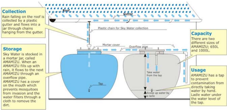
Figure 7.9 AMAMIZU systems. (Source: Author's own).
