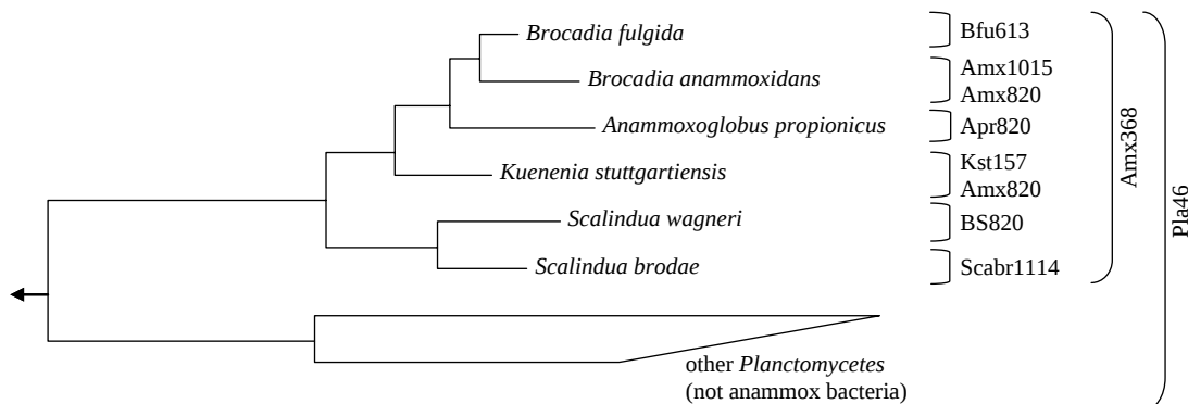
Figure 2.3. 16S rRNA-based phylogenetic tree showing main lineages of known anammox organisms. Brackets indicate the coverage of the probes listed in Table 2.3.
