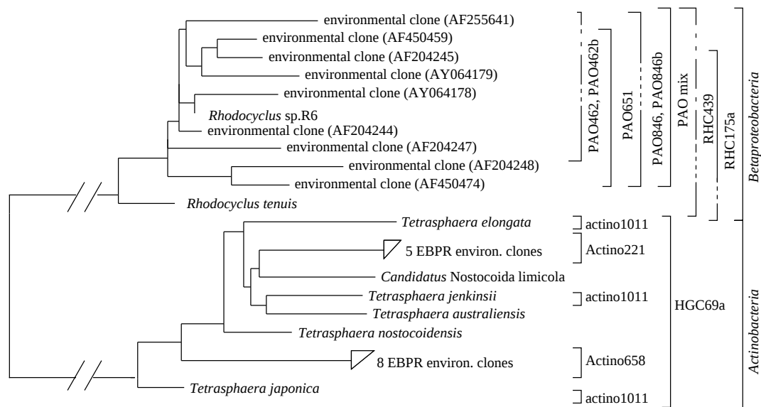
Figure 4.1. 16S rRNA-based phylogenetic tree showing main lineages of known or putative PAOs. Brackets indicate the coverage of the probes listed in Table 4.1.
