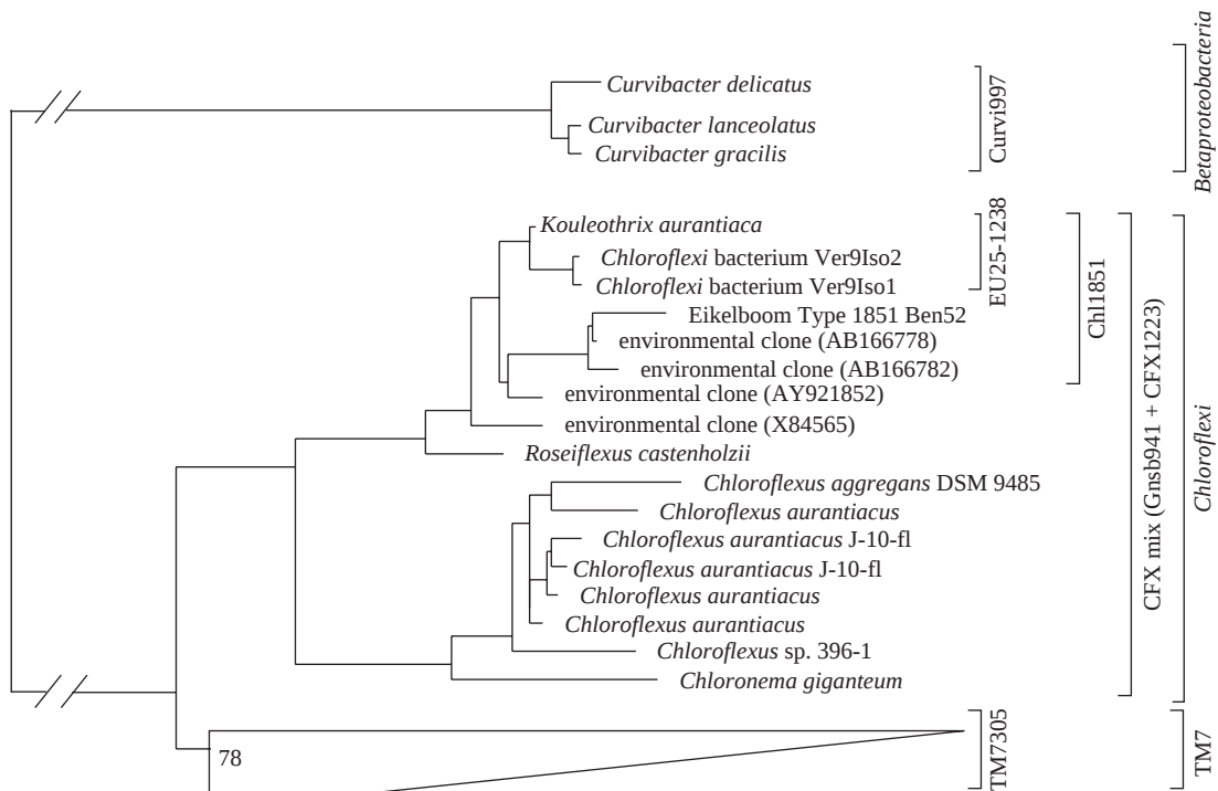
Figure 5.8. 16S rRNA-based phylogenetic tree showing main lineages of known bacteria with attached growth. Brackets indicate the coverage of the probes listed in Tables 5.11 and 5.13–5.14. The exact branching order of the bacteria with attached growth lineages cannot yet be determined due to a limited phylogenetic resolution of the 16S rRNA marker gene. Therefore, unclear tree topology is depicted as multifurcation.
