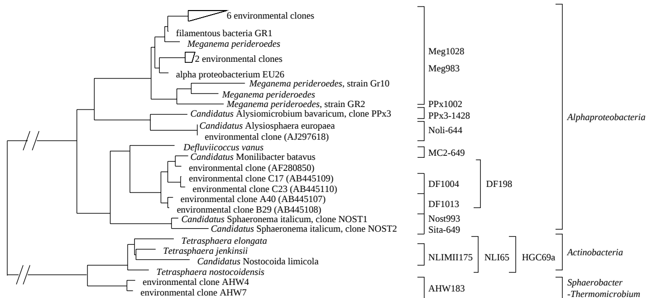
Figure 5.5. 16S rRNA-based phylogenetic tree showing main lineages of Nostocoida limicola morphotypes. Brackets indicate the coverage of the probes listed in Table 5.8. The exact branching order of the Nostocoida limicola morphotypes lineages cannot yet be determined due to a limited phylogenetic resolution of the 16S rRNA marker gene. Therefore, unclear tree topology is depicted as multifurcation.
