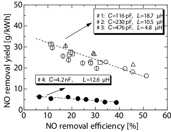
Fig. 9. Dependence of NO removal energy efficiency on NO removal for various circuit conditions.
