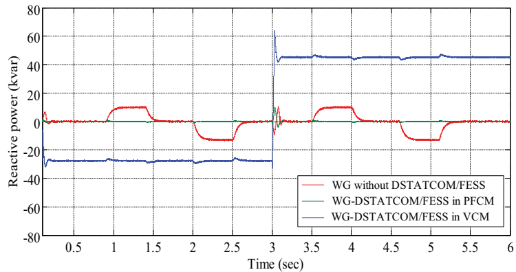
Fig. 8. Reactive power of the WG-DSTATCOM/FESS system
