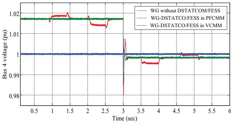
Fig. 9. Voltage at bus 4
