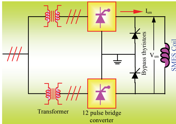
Fig. 2. Schematic diagram of the SMES unit
