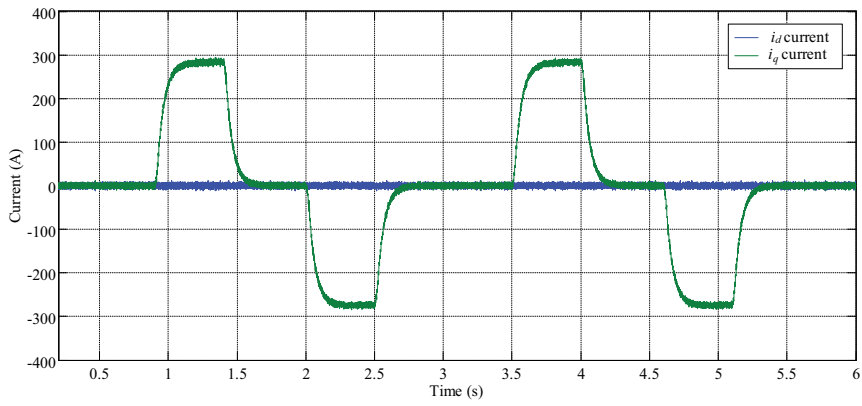
Fig. 14. PMSM i_d and i_q currents
