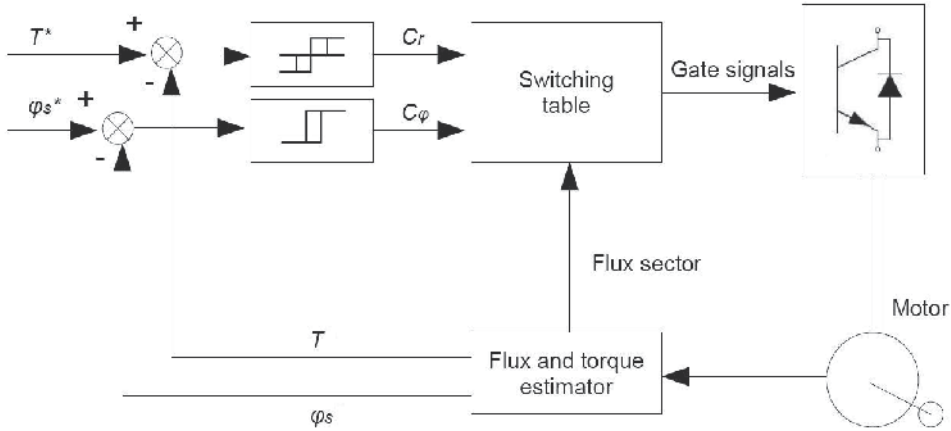
Fig. 10. Basic Direct Torque Control scheme.
