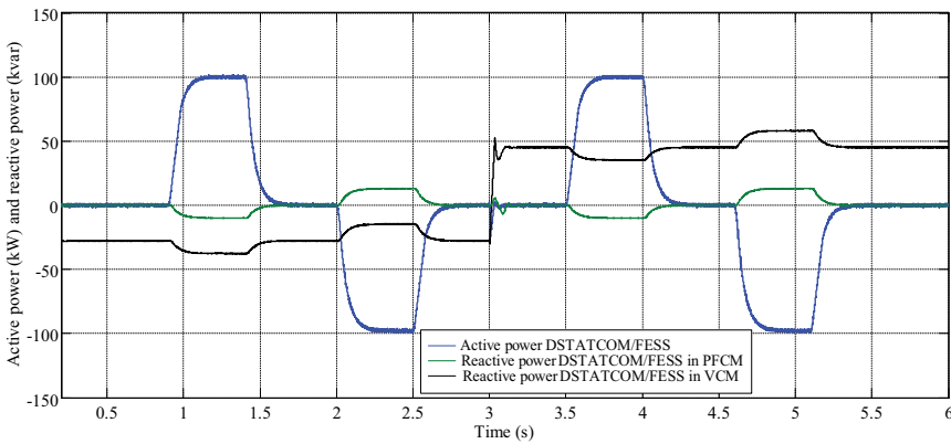
Fig. 10. Input/output active and reactive power of the DSTATCOM/FESS
