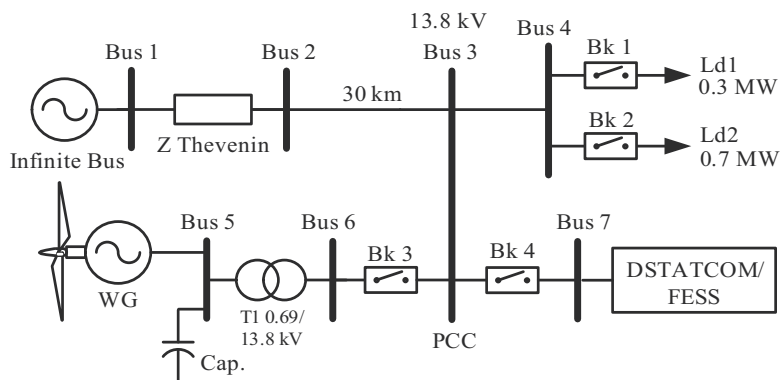
Fig. 5. Test power system
