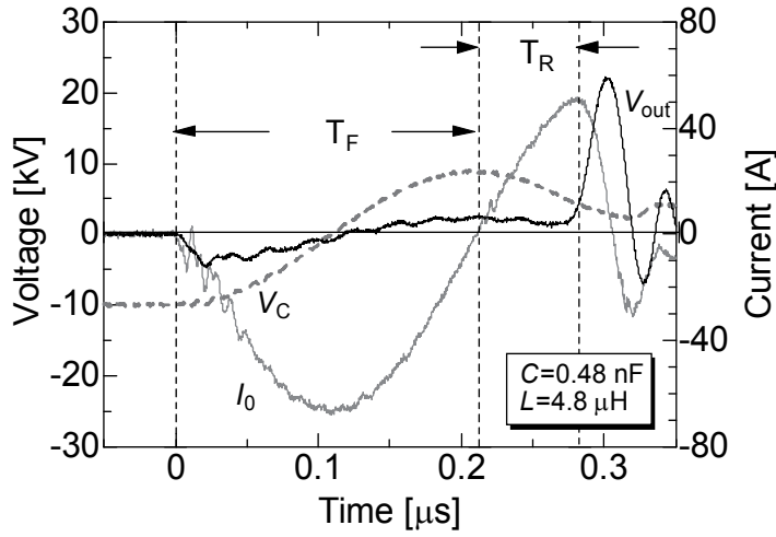
Fig. 3. Typical waveforms of circuit current I_0 , capacitor voltage V_C , and output voltage V_{out} without connection to the load at C=0.48 nF, L=4.8 \mu H and V_0=-10 kV.
