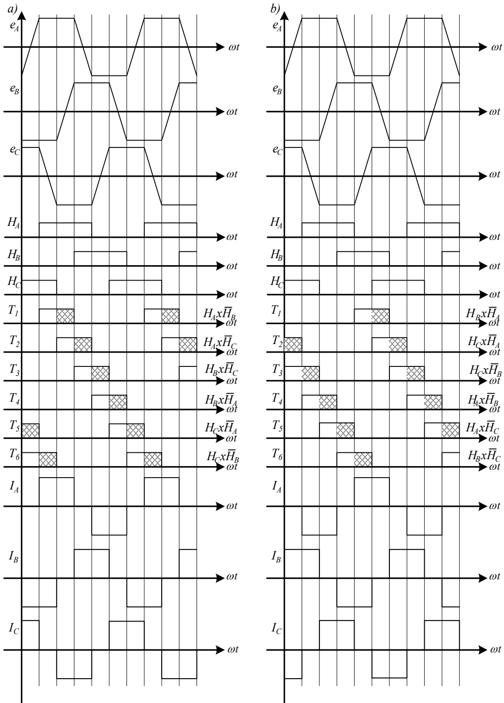
Fig. 30. Time relations between the motor back emf, phase currents, Hall sensors signals and the inverter switches control pulses; a) motor mode operation, b) generator mode operation
