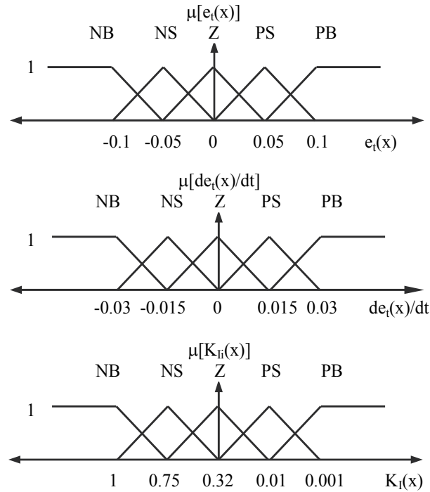
Fig. 9. Membership functions for the fuzzy variables
