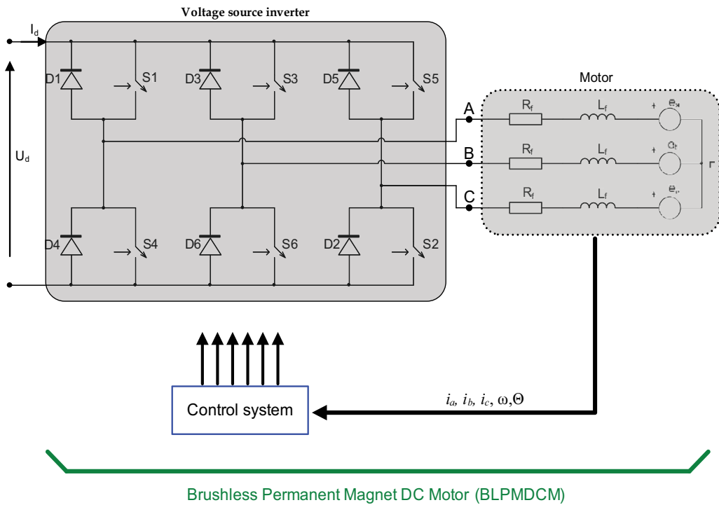
Fig. 6. A brushless permanent magnet DC motor supplied from a voltage source inverter with control system
