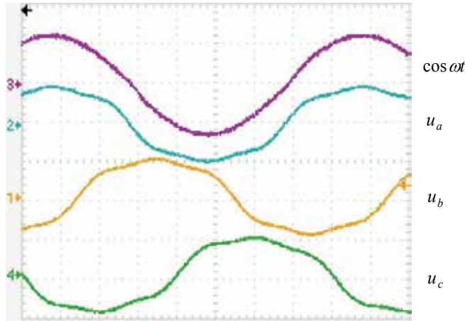
Fig. 17. The synchronizing voltage waveforms and the generated function \cos \omega t
