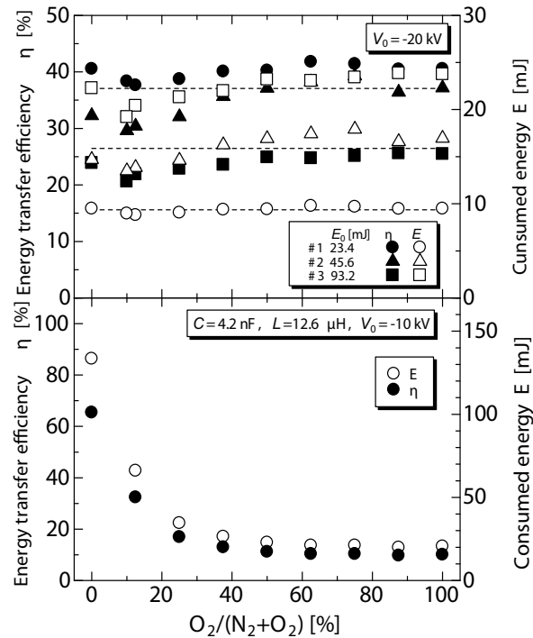
Fig. 12. Energy consumed in the reactor and the energy transfer efficiency from the primary capacitor to the reactor as a function of oxygen concentration for various circuit conditions.
