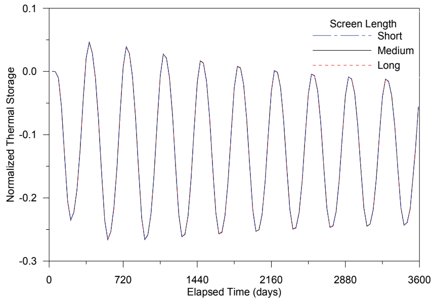
Fig. 11. History of balance of thermal energy obtained from simulations with different screen length
