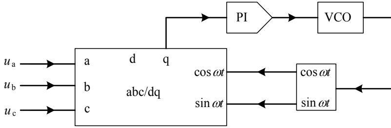
Fig. 16. Block diagram of the synchronization circuit
