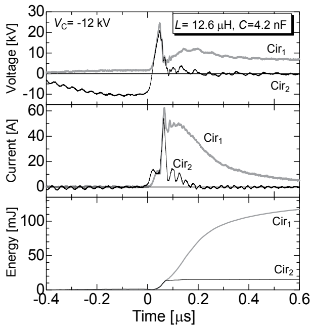
Fig. 16. Waveforms of applied voltage, discharge current, and energy consumed in the reactor for two different circuits.
