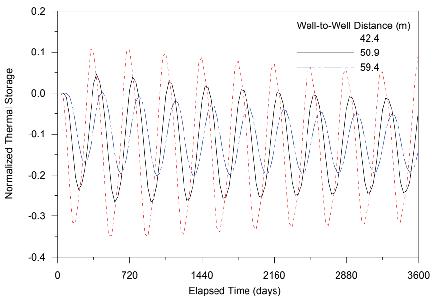
Fig. 9. History of balance of thermal energy obtained from simulations with different interwell distances
