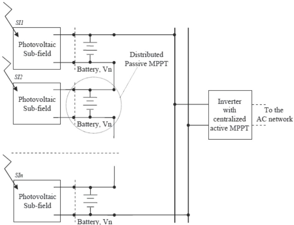
Fig. 3. Grid-connected photovoltaic system with distributed use of batteries as distributed passive MPPTs and centralized inverter with active MMPT function.
