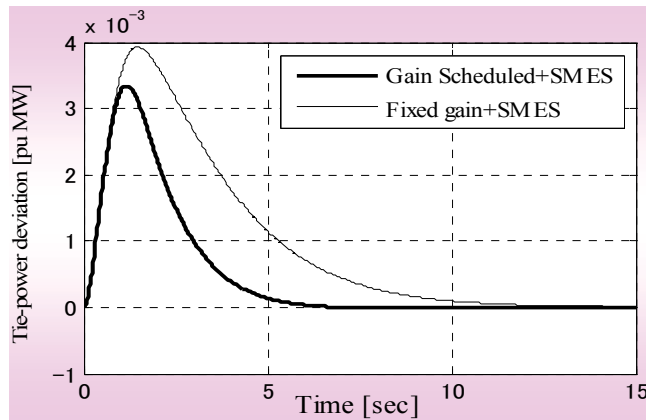
Fig. 11. Performances of the tie power deviation for a step load increase \Delta P_{L2}=0.01 pu in area2 only
