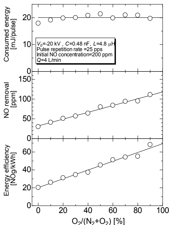
Fig. 13. Consumed energy, NO removal and its energy efficiency as a function of oxygen concentration in the NO contained gas mixture for the circuit condition 3; C=0.48 nF and L=4.8 \mu H at V_0 = -20 kV, 25 pps in pulse repetition rate and 4 L/min in gas flow rate.
