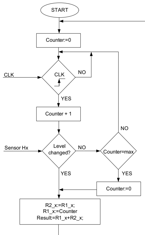
Fig. 32. Flowchart of the algorithm determining the frequency of a single Hall sensor signal
