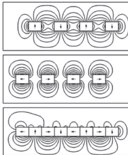
Fig. 6. Halbach array configuration. Magnetic potential in a radial magnet array (top), azimuthal magnet array (middle) and composition of both in a Halbach array (bottom).
