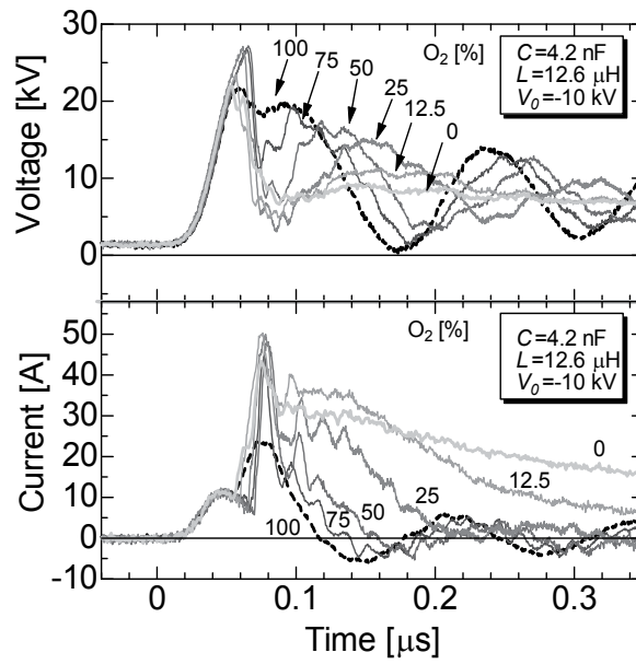
Fig. 11. Time-dependences of applied voltage and discharge current for various oxygen concentrations in the gas mixture at C=4.2 \text{ nF} , L=12.6 \text{ } \mu\text{H} and V_0=-10 \text{ kV} .
