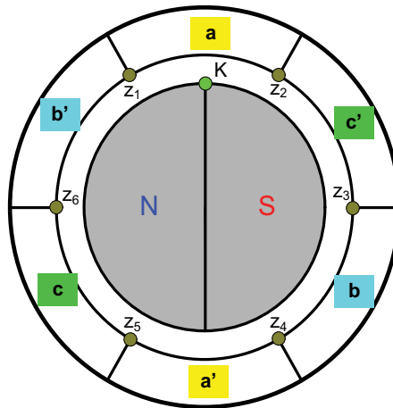
Fig. 12. The cross section of a BLDCM motor
