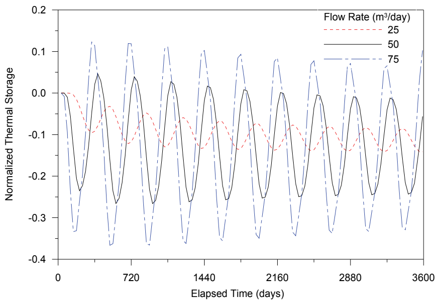
Fig. 8. History of balance of thermal energy obtained from simulations with different injection/production flow rates
