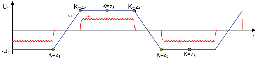
Fig. 13. Waveforms of the current and back electromotive force in one phase depending on the permanent magnet poles position
