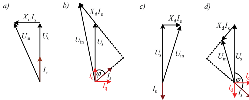
Fig. 22. Phasor diagrams for several selected parameters of the input voltage U_{in} vector
