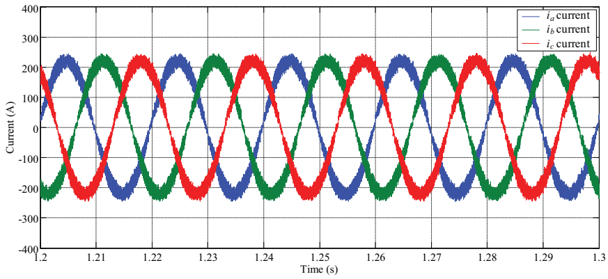
Fig. 15. DSTATCOM i_a , i_b and i_c currents
