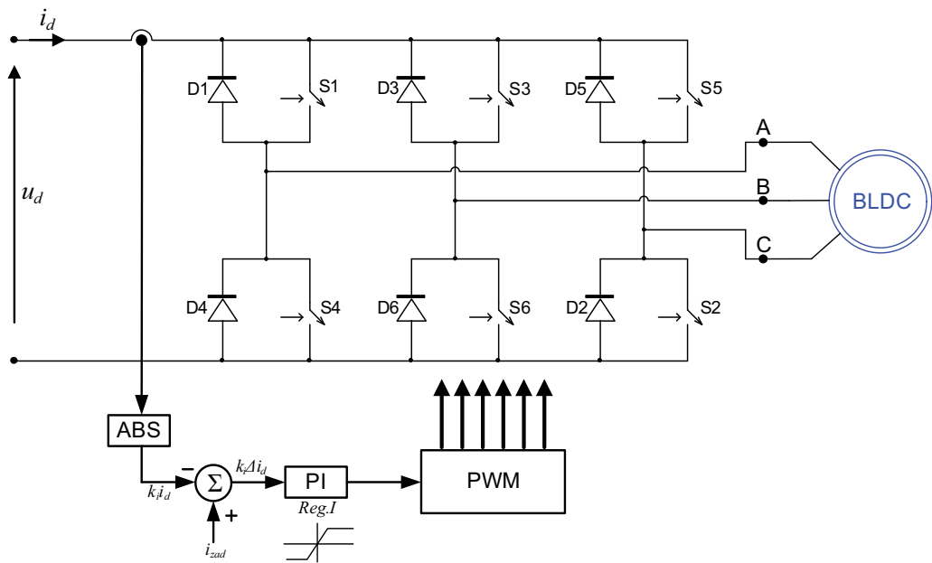
Fig. 10. Measurement of the inverter input current
