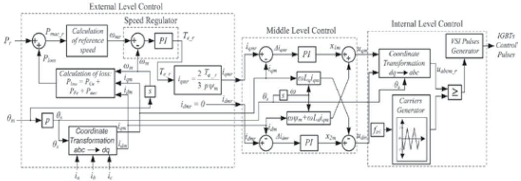
Fig. 4. Multi-level control scheme of the FESS
