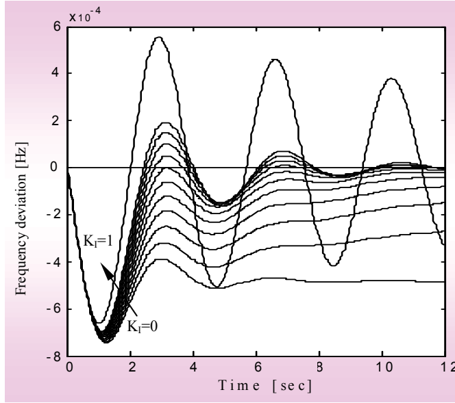
Fig. 7. Frequency deviation step response for different values of K_I
