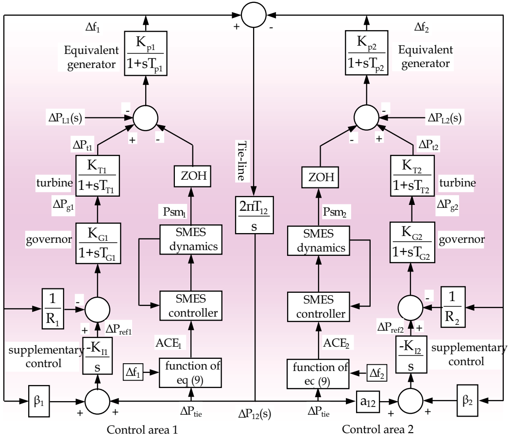
Fig. 6. Digital simulation model for the two-area power system
