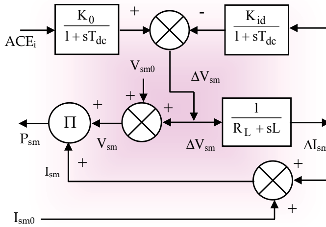
Fig. 10. Superconducting magnetic energy storage unit control system
