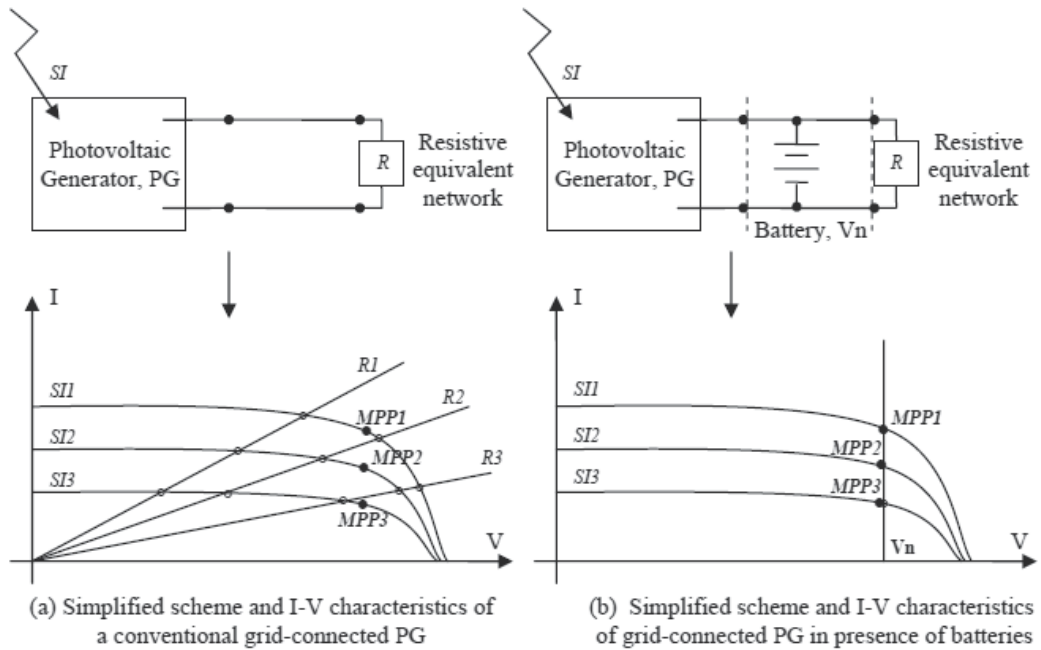
Fig. 1. Working points analysis of grid-connected photovoltaic systems, without (a) and with (b) the use of batteries.
