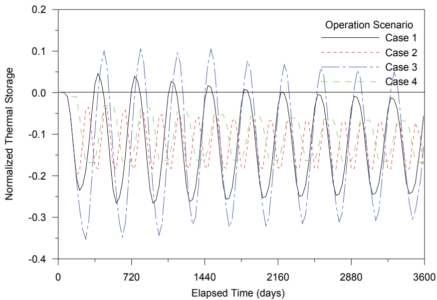
Fig. 4. History of balance of thermal energy obtained from simulations with different operation scenarios
