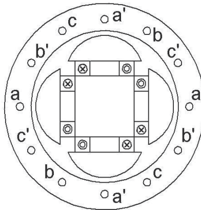
Fig. 1. Cross section of a three phase generator with a four salient pole rotor.
