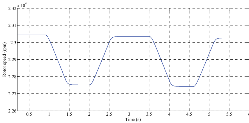
Fig. 12. Rotor speed of the PMSM
