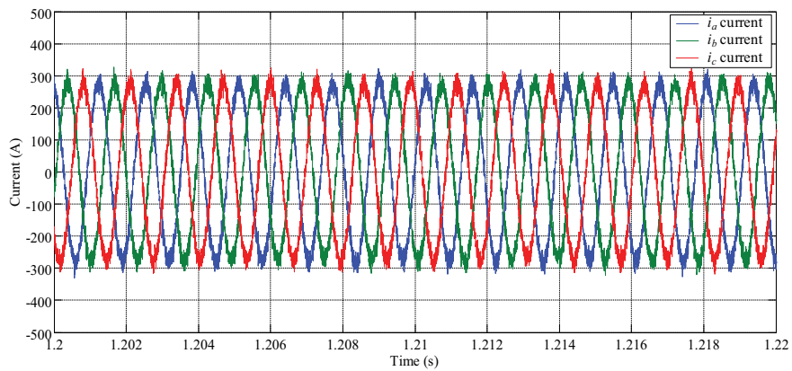
Fig. 16. PMSM i_a , i_b and i_c currents
