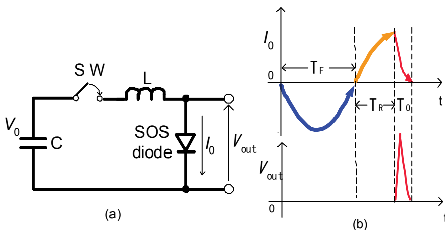
Fig. 1. Schematic of an inductive energy storage pulse power generator with semiconductor opening switch: (a) equivalent circuit; (b) circuit current and output voltage.
