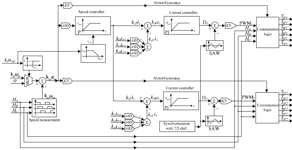
Fig. 28. The inverters' control system
