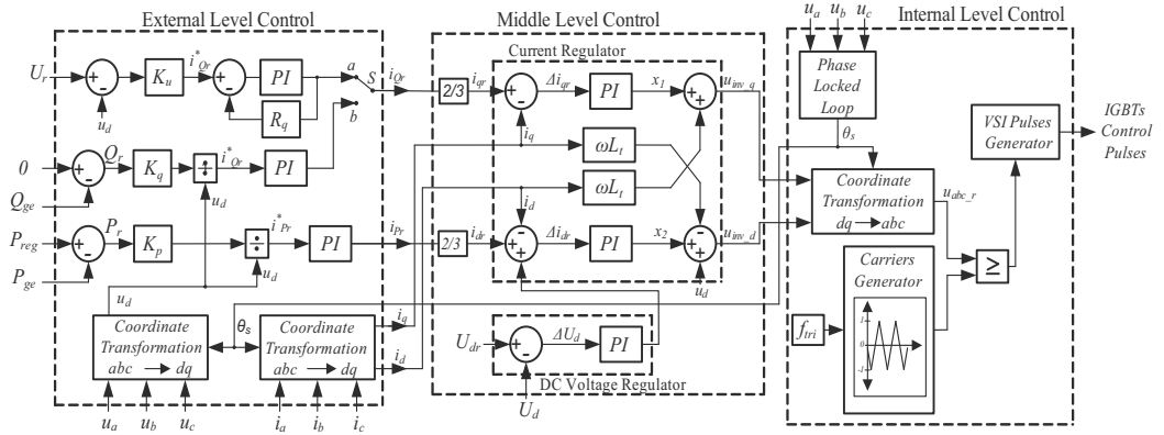
Fig. 3. Multi-level control scheme of the DSTATCOM device
