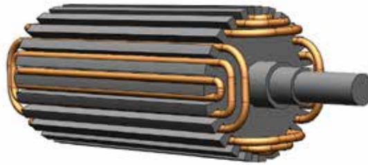
Fig. 11. Four pole rotor configuration of a BDFIM.
