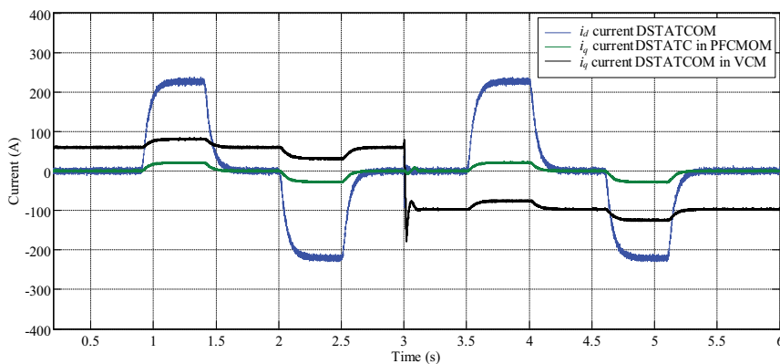
Fig. 13. DSTATCOM i_d and i_q currents
