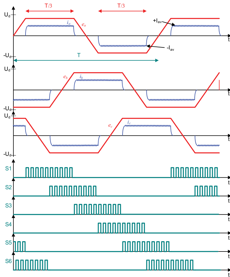
Fig. 7. Bipolar pulse width modulation: phase currents and switch control pulses
