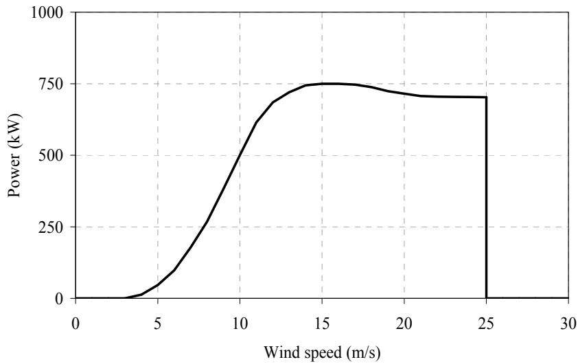
Fig. 19. Power curve of the wind turbine
