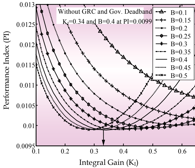
Fig. 8. The optimal integral controller gain, K_I and frequency bias factor, B
