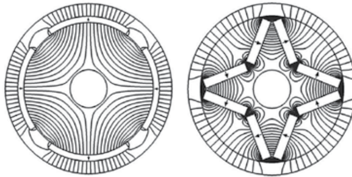
Fig. 5. Rotors with surface mounted (left) and internal mounted (right) magnets with the magnetic field lines induced in the airgap and in the rotor steel.
