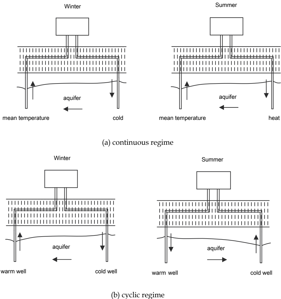
Fig. 1. Basic operational regimes for aquifer thermal energy storage (after Nielsen)
