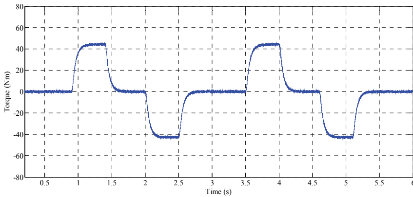
Fig. 11. Electromagnetic torque of the PMSM
