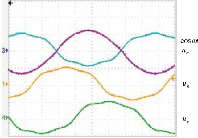
Fig. 18. The synchronizing voltage waveforms and the generated function \cos\omega t
