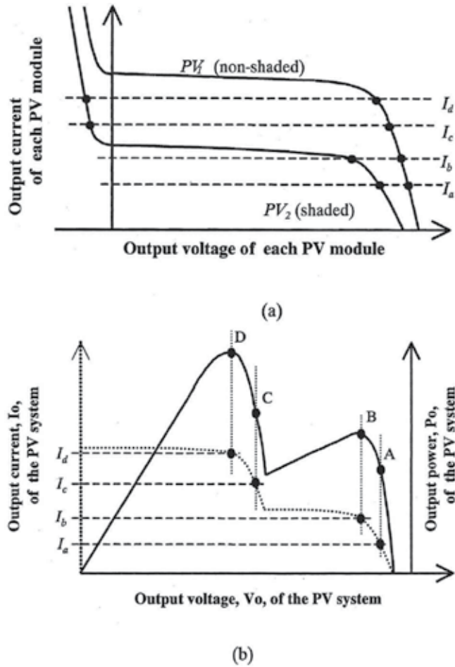
Fig. 2. PV module output current versus PV module output voltage, for different irradiation levels, 2(a), and effects of different solar irradiation levels on a string composed by two PV modules connected in series, 2(b). [Shimizu et Al., 2003]
