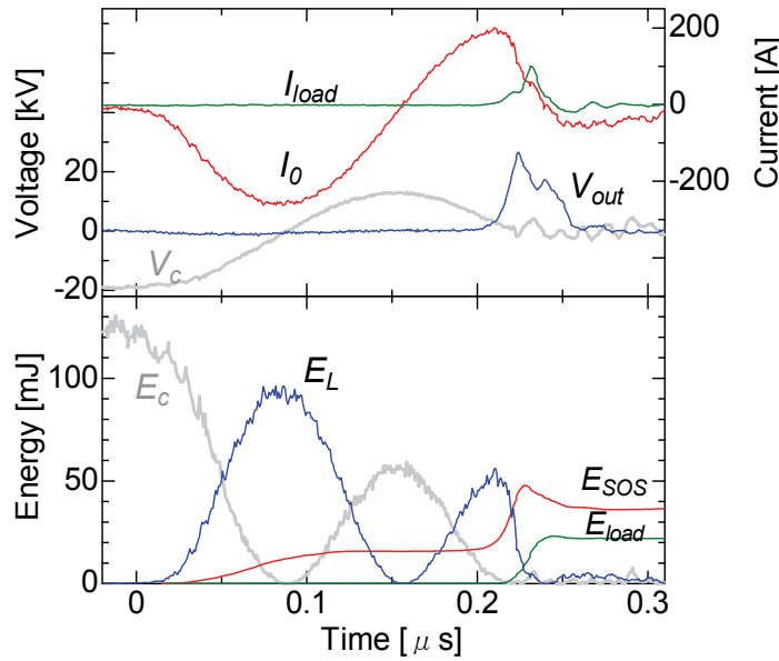
Fig. 4. Typical time-dependency of the discharge current I_{load} , the circuit current I_0 , the reactor voltage V_{out} and energy consumed in SOS, E_{SOS} and in the reactor E_{load} at C=0.68 nF, L=1.4 \mu H and V_{C0}=-20 kV. E_C and E_L mean energies stored in the capacitor and the inductor, respectively.
