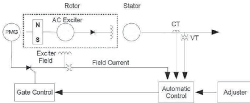
Fig. 4. Alternator-rectifier exciter employing rotating non-controlled rectifiers.
