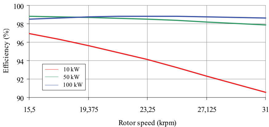
Fig. 17. Efficiency of the PMSM
