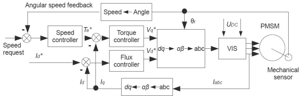
Fig. 8. Typical cascaded control structure for PMSM drivers.
