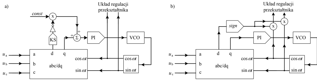
Fig. 19. Two versions of the synchronizing circuit enforcing the correct generation of \cos\omega t function
