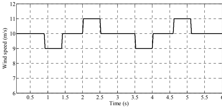
Fig. 6. Wind speed
