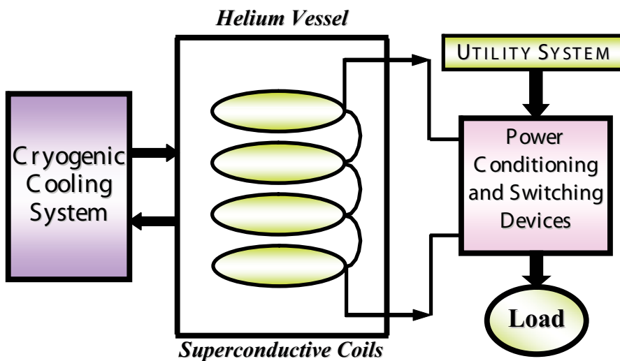
Fig. 1. Schematic diagram of the basic SMES system
