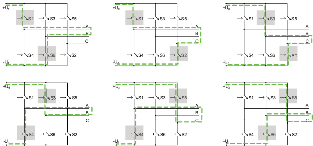
Fig. 8. Bipolar pulse width modulation: the sequence of switching
