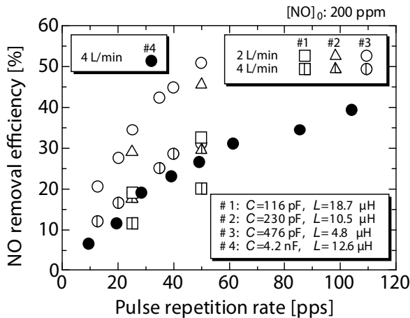
Fig. 7. Dependence of NO removal efficiency on pulse repetition rate for various gas flow rates and circuit parameters.
