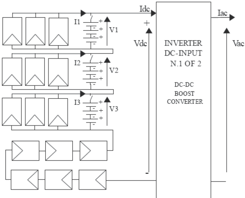
Fig. 4. Electrical scheme of the experimentally tested 3 kWp grid-connected PV plant
