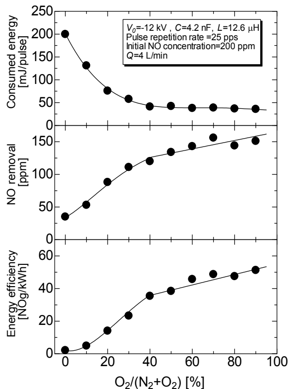
Fig. 14. Consumed energy, NO removal and its energy efficiency as a function of oxygen concentration in the NO contained gas mixture for the circuit condition; C=4.2 nF and L=12.6 \mu H at V_0 = -12 kV, 25 pps in pulse repetition rate and 4 L/min in gas flow rate.
