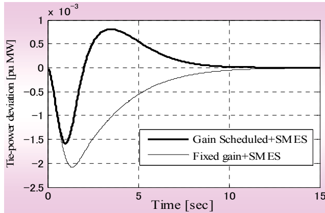
Fig. 13. performances of tie power deviation for a step load increase \Delta P_{L1}=0.015 pu in area1 & \Delta P_{L2}=0.01 pu in area2
