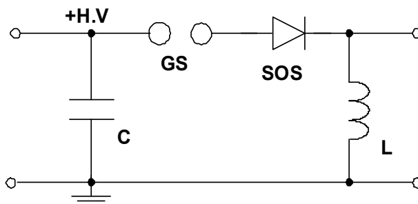
Fig. 15. Pulse power circuit for prevention of glow generation.
