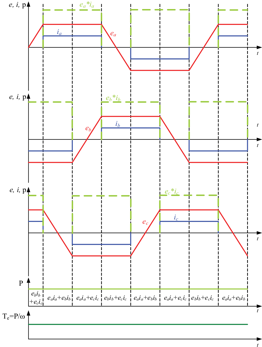
Fig. 5. Desired waveforms of electromotive force, phase currents, instantaneous power and electromagnetic torque
