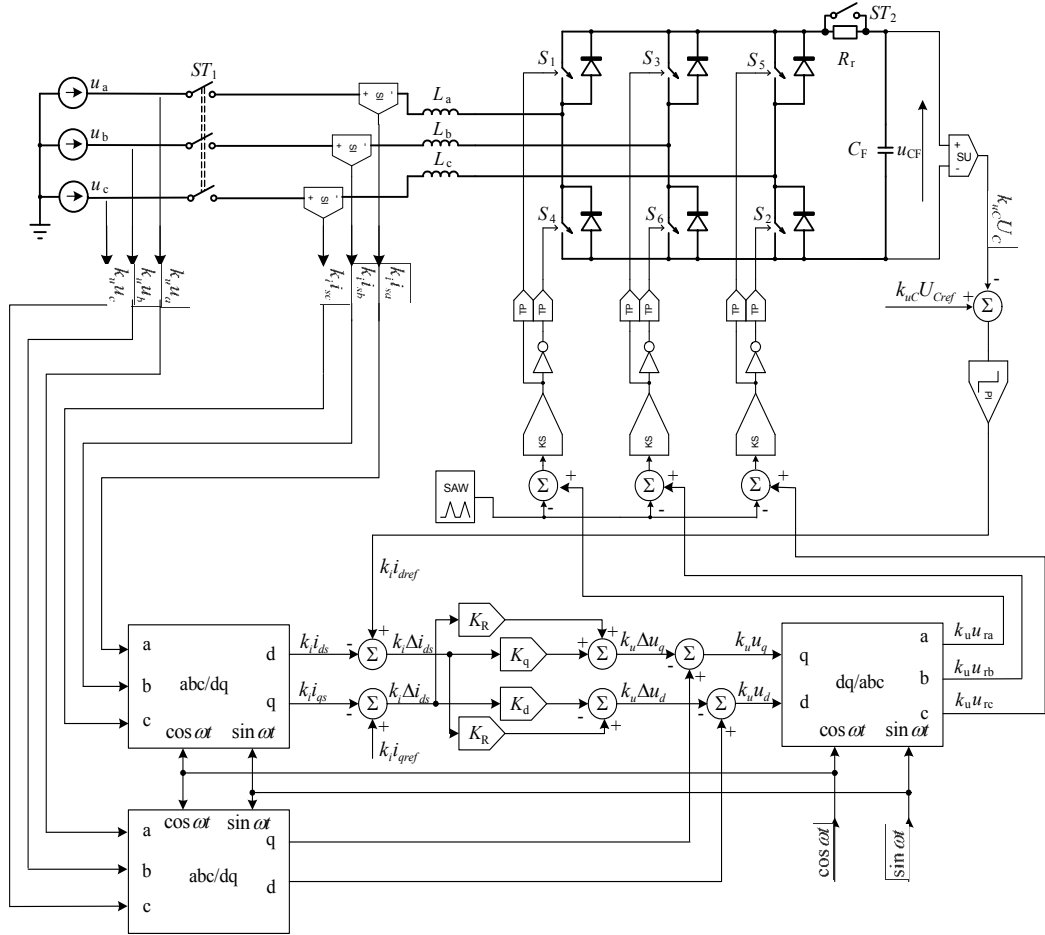
Fig. 15. Block diagram of the control system and the power circuit
