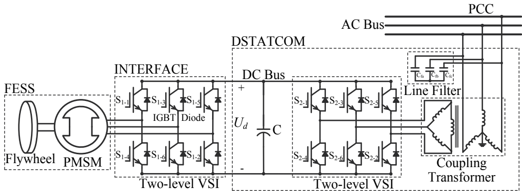
Fig. 1. Representation of the DSTATCOM/FESS controller
