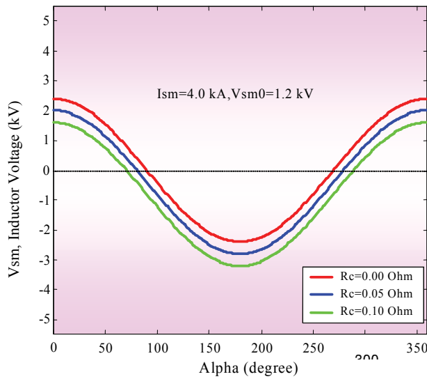
Fig. 3. Effect of inductor voltage, V_{sm} with the variation of firing angle of 12-pulse converter
