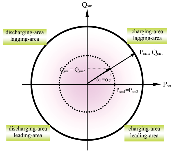
Fig. 4. Conceptual diagram of active and reactive power control of MES unit under equal- \alpha mode
