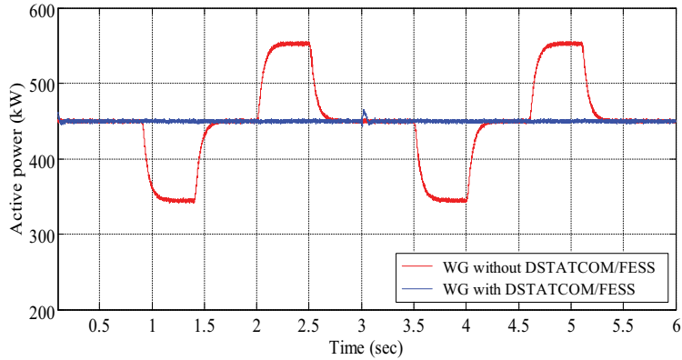
Fig. 7. Active power of the WG-DSTATCOM/FESS system
