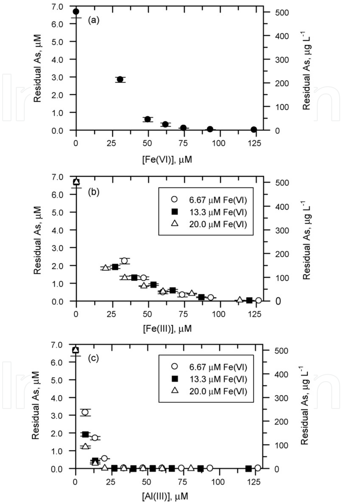
Fig. 17. Removal of arsenite by Fe(VI) (a), Fe(VI)/Fe(III) salts (b), and Fe(VI)/ Al(III) salts (c) at pH 6.5. Initial concentration = 500 μg As(III)/L [81].
