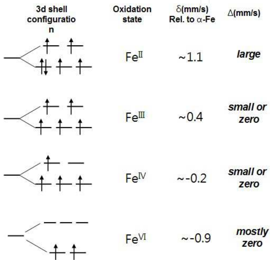
Fig. 2. Schematic representation of the 3d shell configuration of iron in selected oxidation states with characteristic Mössbauer parameters. Isomer shifts are given at room temperature relative to \alpha\text{-Fe} , note that, the ligand field splitting corresponding to the most common octahedral coordination for \text{Fe}^{\text{II}} to \text{Fe}^{\text{IV}} while it is tetrahedral for \text{Fe}^{\text{VI}} [15]. Among regular iron compounds, \text{Fe}^{\text{II}} has the highest isomer shift, and the 3d^6 configuration of the valence shell represents one more t_{2g} electron compared to 3d^5 of spherical symmetry, thus the quadrupole splitting is also large. \text{Fe}^{\text{III}} has only five 3d electrons, and therefore the isomer shift becomes smaller. Since the illustrated 3d splitting is only an idealized non-distorted case, the observed quadrupole splitting is very rarely zero, it is mostly below 1 mm/s and may even be larger. The distortion of the octahedron can be caused by the Jahn-Teller effect, lattice symmetry, neighboring charges, defects, etc.
