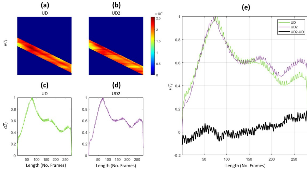
Figure 9 - wT_I for UD1 (a), wT_I for UD2 (b), aT_I for UD1 (c), aT_I for UD2 (d), aT_{I_{sub}} (e).
