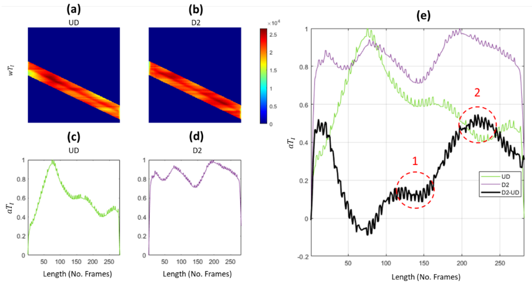
Figure 13 - wT_I undamaged baseline (a), wT_I image for D2 (b), aT_I undamaged baseline (c), aT_I profile for D2 (d), aT_{I_{sub}} (e).
