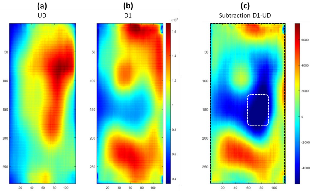
Figure 10 - Thermal dT_I images for undamaged baseline (a), damaged sample D1 (b), baseline subtraction dT_{I_{sub}} (c).
