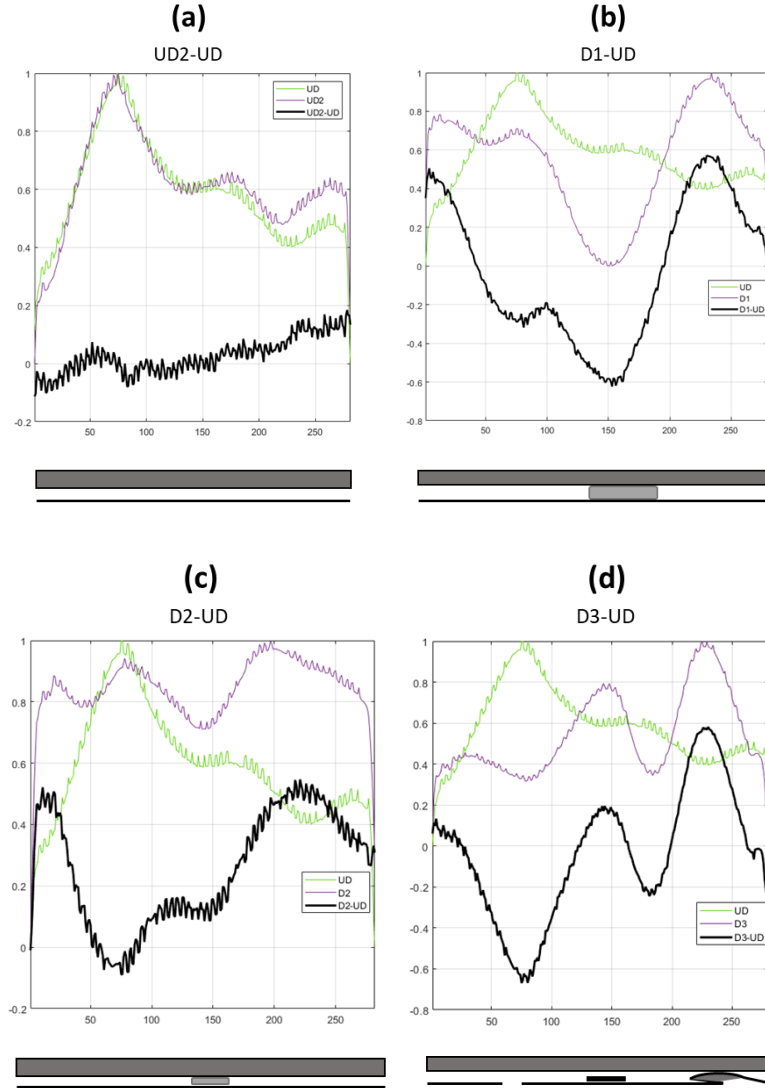
Figure 16 - dT_{I_{sub}} profiles for UD2 (a), D1 (b), D2 (c) and D3 (d) samples with samples illustration
