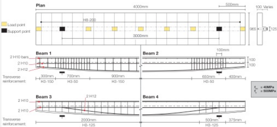
Figure 12 - T-Beam general arrangement
