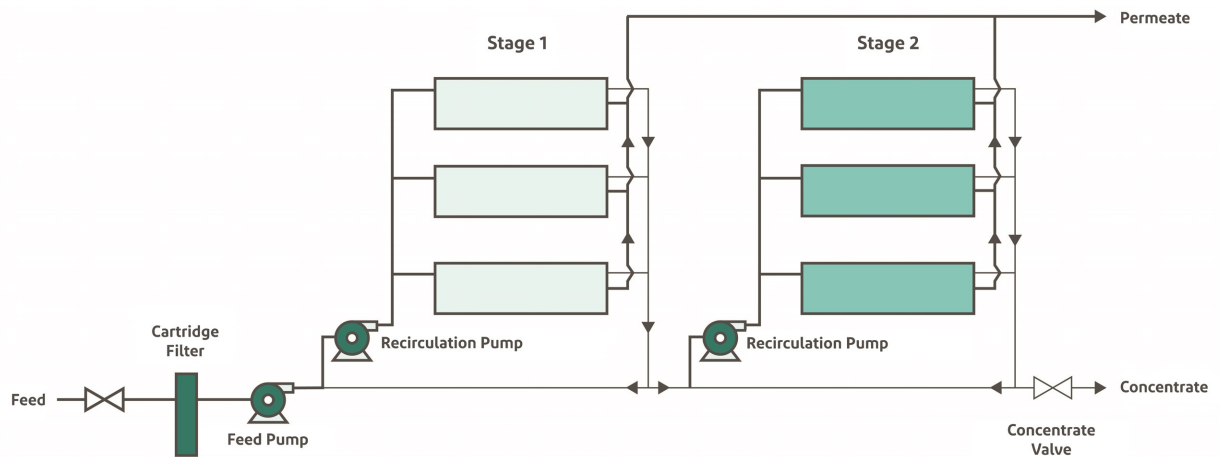
Figure 34. Two-stage system with internal concentrate recirculation
