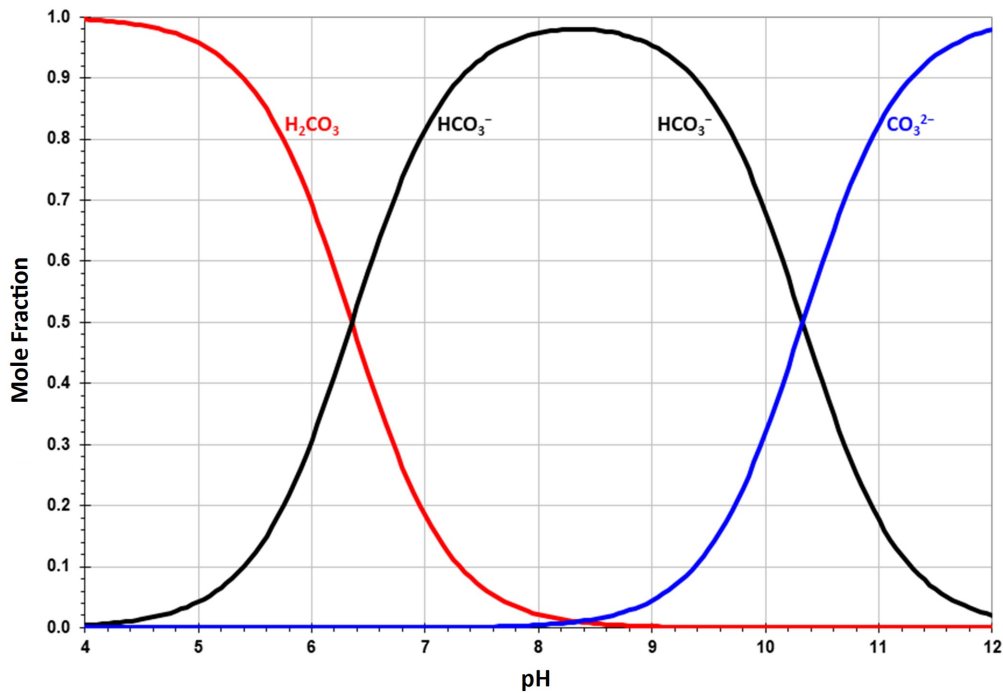
Figure 38. Bicarbonate Equilibrium
