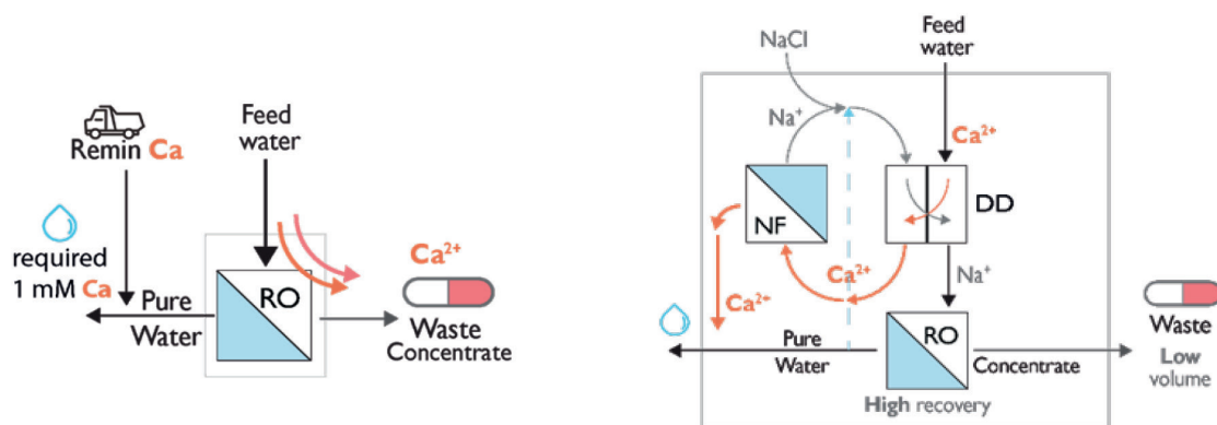
Fig. 1. A) Current status of drinking water treatment to guarantee the removal of micropollutants. B) DoReMi process for drinking water production (Dutch patent NL2021733). The feed water is pre-treated with Donnan dialysis and the hardness minerals are recovered with a nanofiltration unit.
