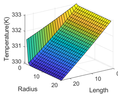
Fig. 3. Radial and longitudinal temperature profile for a T_{in} = 60^{\circ}\text{C} , T_w = 70^{\circ}\text{C} , v = 0.5 \text{ m/s} .
