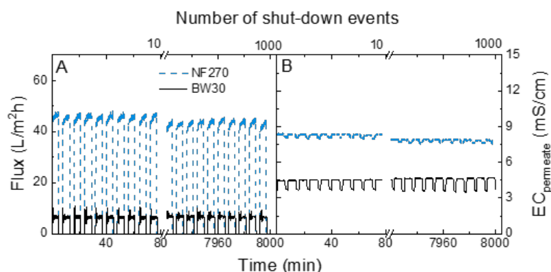
Fig. 1. Membrane performance (A) flux and (B) electrical conductivity of permeate as a function of time with 1000 shutdown events. Feed solution: 10 g/L NaCl with 1 mM NaHCO 3 , 24 ± 1°C. Each cycle: high-level solar irradiance 800 W/m 2 (namely 10 bar operating pressure) for 5 min dropping to zero (namely pump-off) for 3 min.
