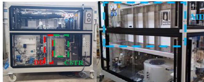
Fig. 1. Pilot plant installed at Electróniquel S.A. company. Front side (left) and back side (right).
