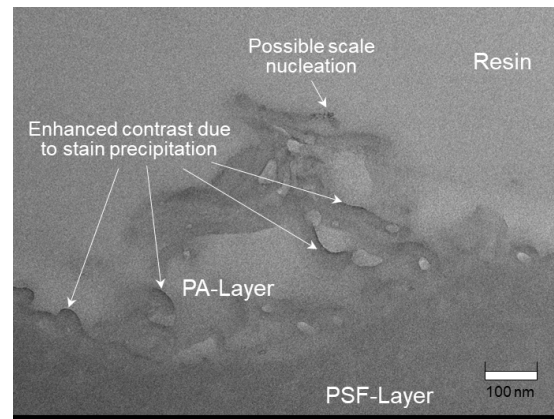
Fig. 4. TEM image of a RuO 4 -stained BW30 membrane cross-section. It shows a complex fold of the polyamide (PA)-layer nodules with dense stain precipitations present on the edges of the ridge-valley structures of the PA-layer as well as within the void spaces in the PA-layer.
