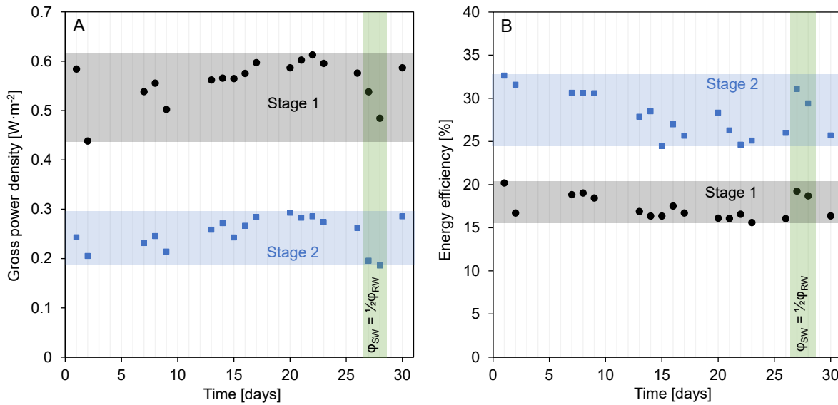
Fig. 1 (attached) – Stage 1 (dots) and stage 2 (squares) contributions to gross power density (A) and energy efficiency (B) over the experiment run. Different flow rate conditions were used on days 27 and 28, shadowed in green.
