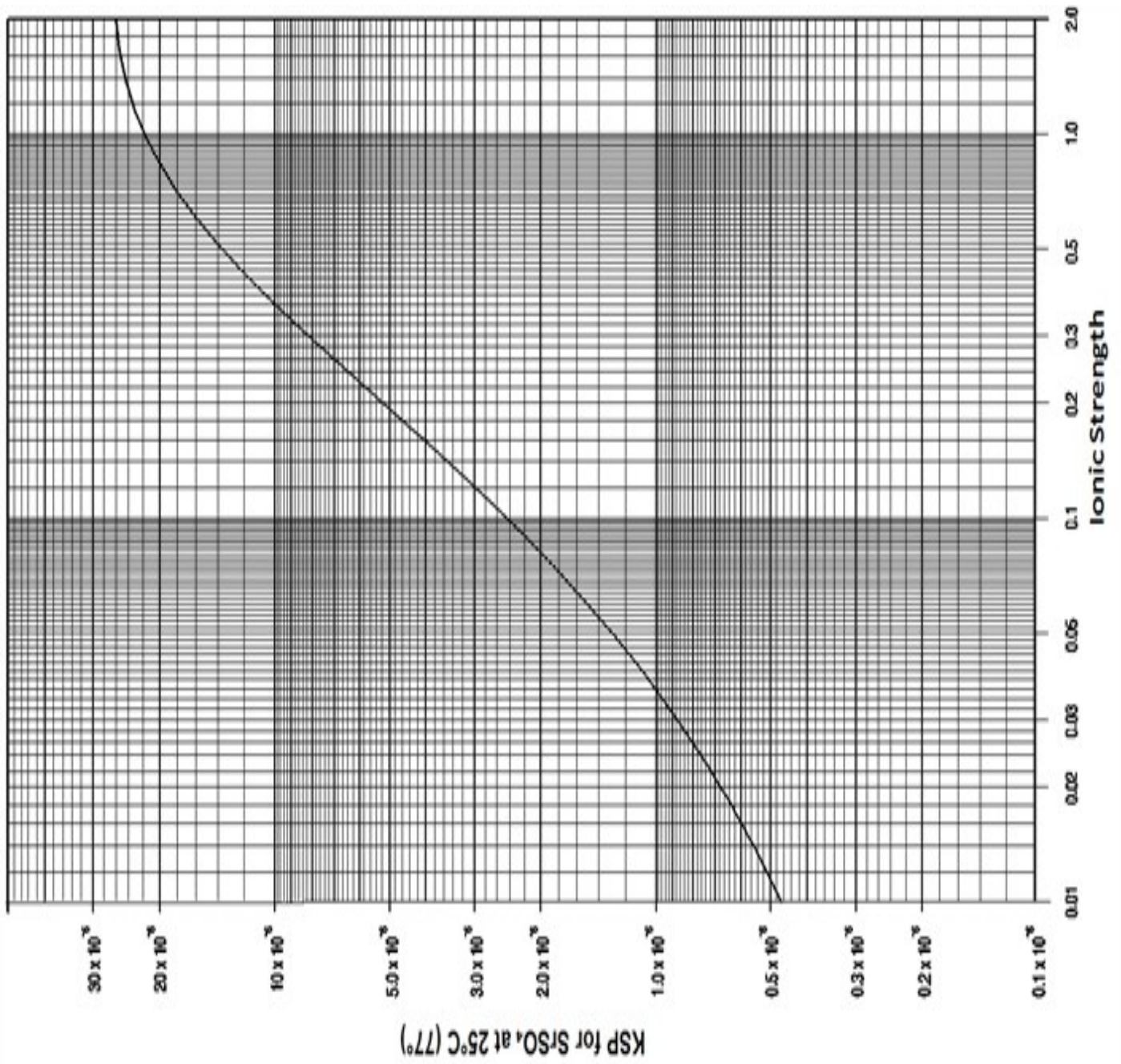
Figure 23. K_{sp} for SrSO_4 versus ionic strength / 10/
