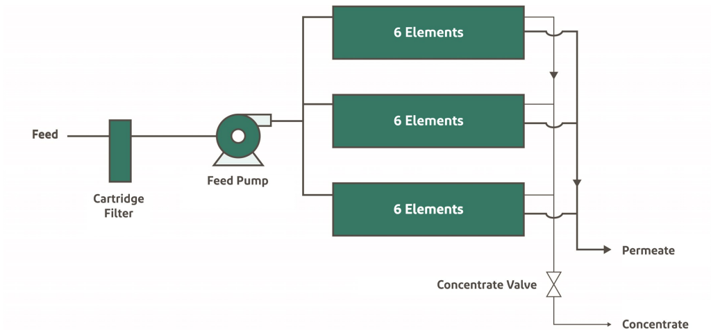
Figure 32. Single-stage system
