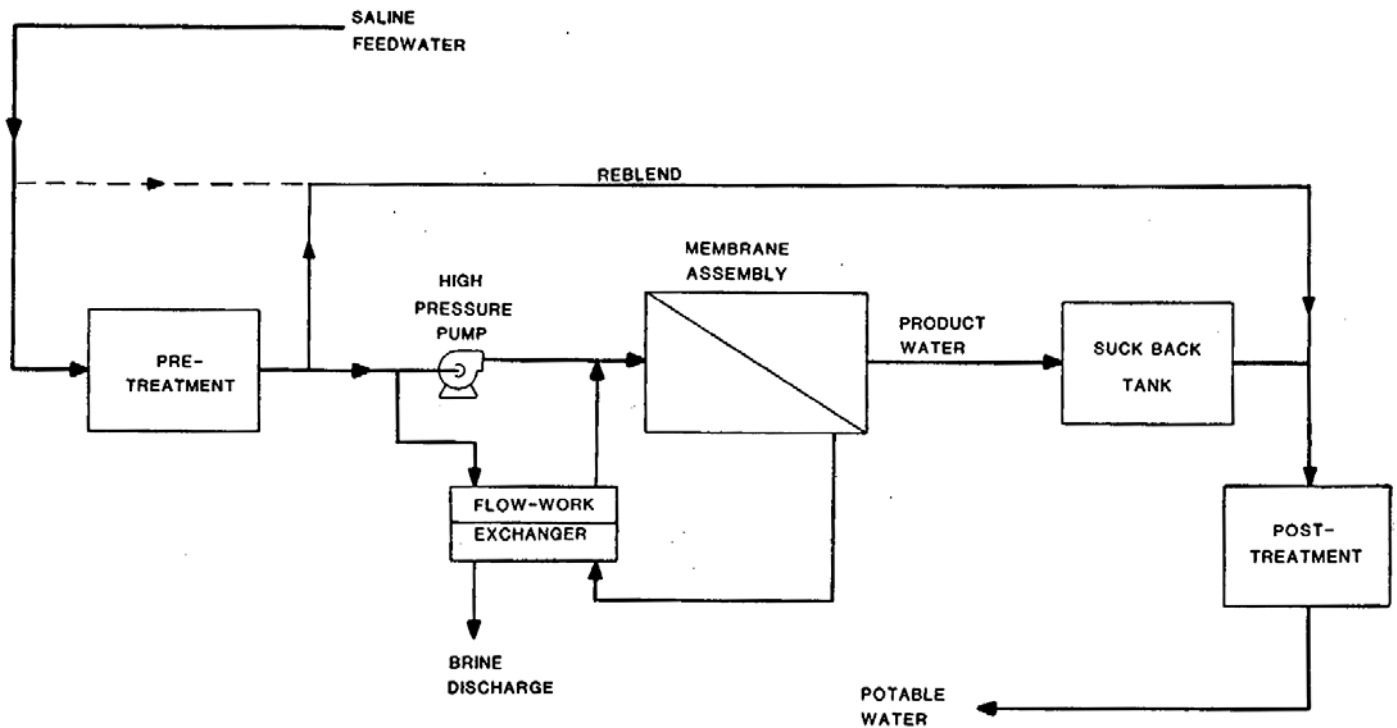
Figure 4-3 Reverse osmosis desalination system
