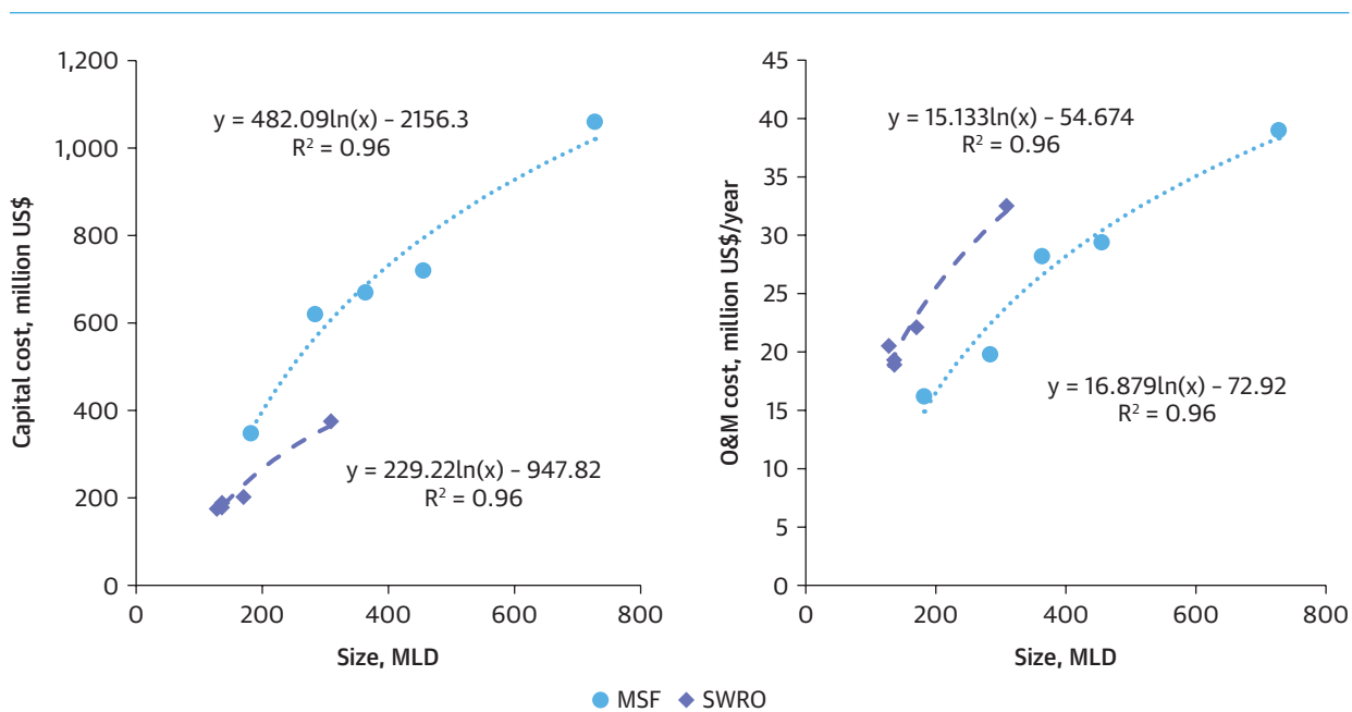
FIGURE 4.4. Capital and Operation and Maintenance Costs of Hybrid Desalination Plants as a Function of Freshwater Production Capacity
