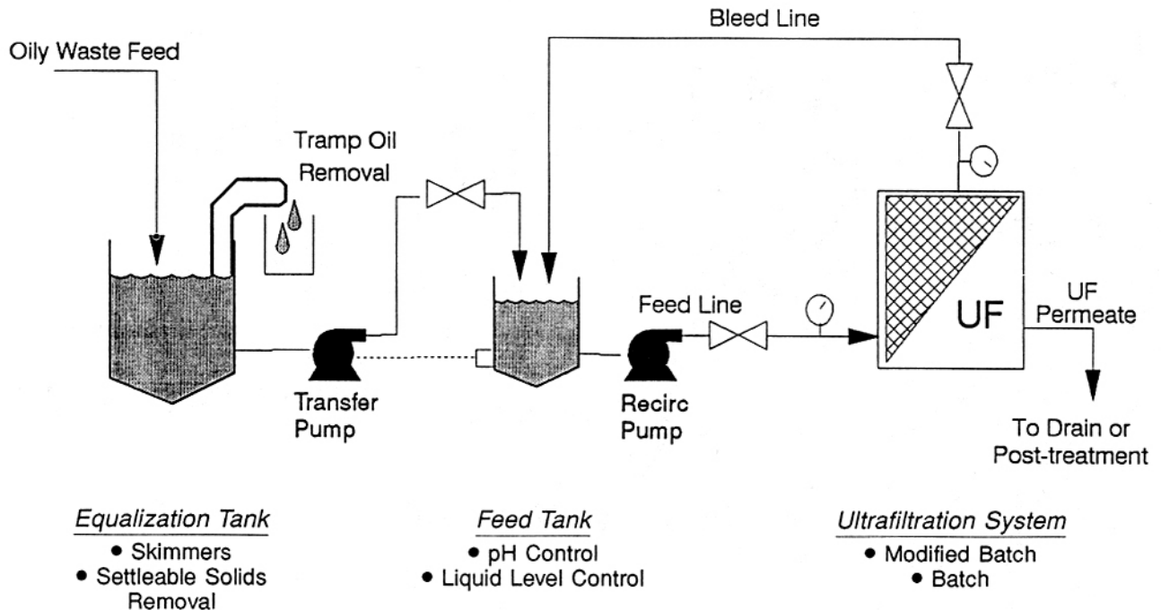
Figure 2.19 Typical Ultrafiltration Wastewater Treatment Flow Schematic 19
