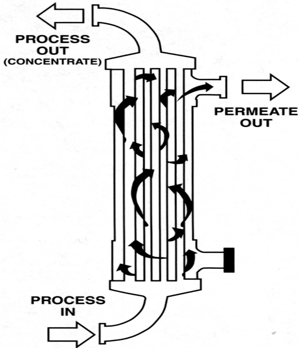
Figure 2.22 Hollow Fiber Cartridge 22
