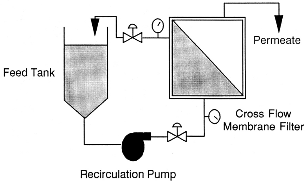
Figure 2.24 Tubular Arrangement and Batch Process 24
