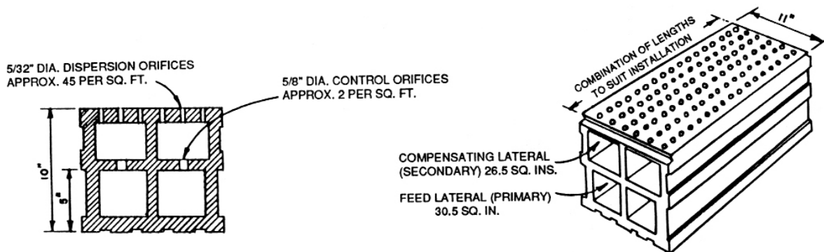
B. LEOPOLD BLOCK SYSTEM (Courtesy of F.B. Leopold Co.)
