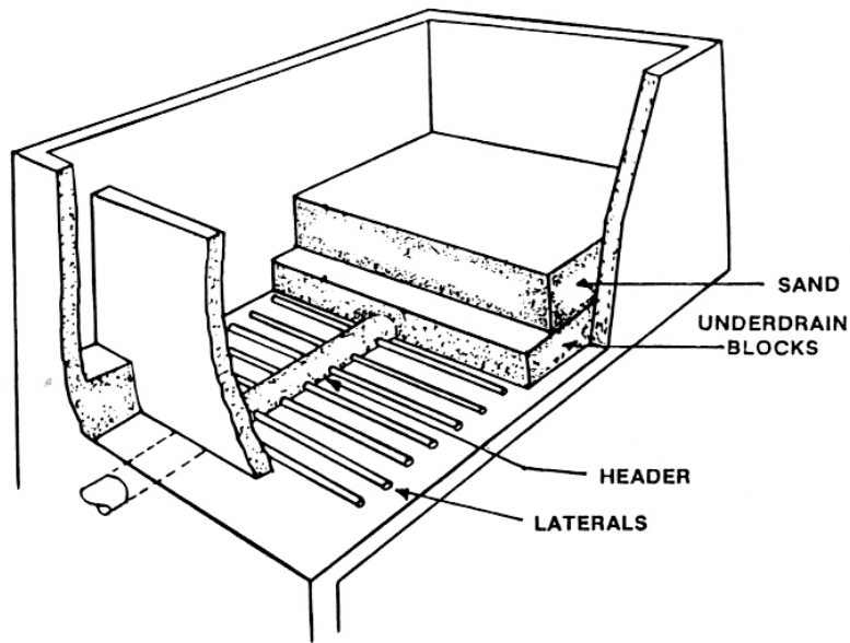
A. HEADER LATERALS (Courtesy of the AWWA)
