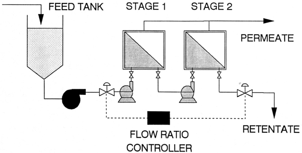
Figure 2.25 Modified Batch Process and Stages in Series Process 25
