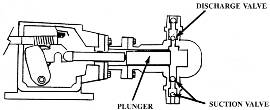
PLUNGER PUMP
