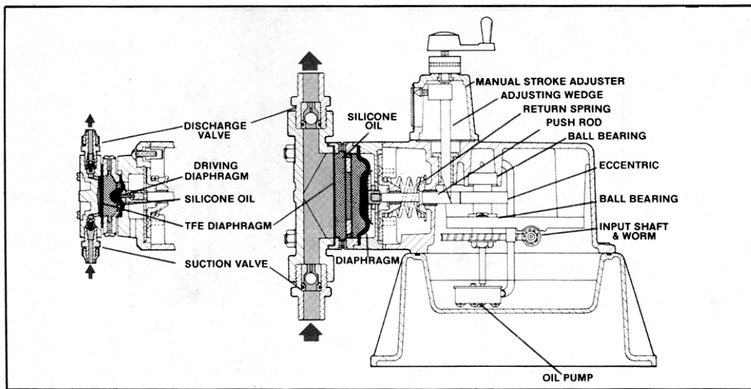
Diaphragm Pump
