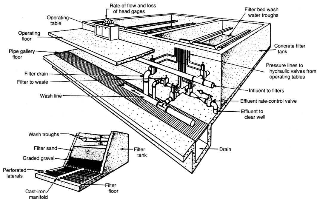
Figure 2.13 Rapid Sand Filter 13
