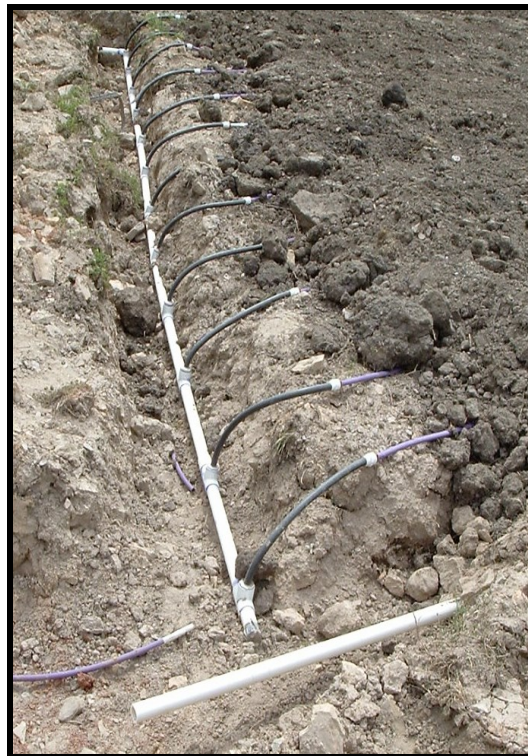
Subsurface Drip Dispersal. A manifold trench and supply manifold line is shown with flexible pipe connected to the small diameter drip irrigation lines. The return manifold from the opposite end of the zone is shown in the foreground. Drip lines are often plowed into the soil; this photo shows suitable imported soil used to cover the drip lines.
