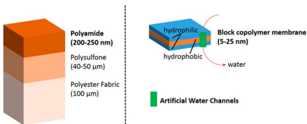
Figure 3. Scheme showing membrane structure and characteristic sizes. A typical composite membrane with the three layers based on polyamide, polysulfone, and polyester (left). A biomimetic block copolymer membrane with an artificial water channel incorporated as a functional motif (right).
