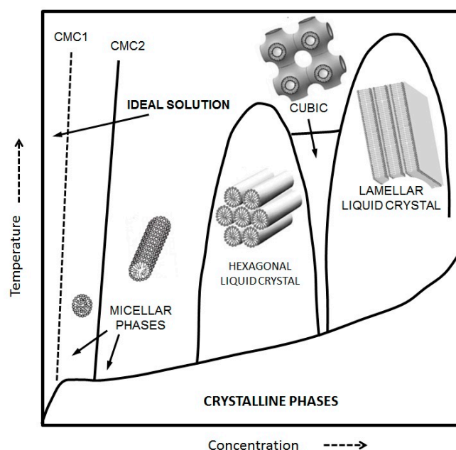
Figure 2. Typical phase diagram showing the different self-assembled structures as a function of concentration and temperature for a general amphiphile.
