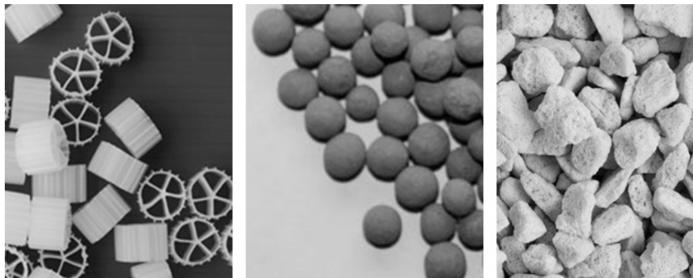
Figure 5. Examples of different types of carriers. From left to right, Kaldnes Miljøteknologi (KMT) , porous ceramsite, and recycled porous glass.
