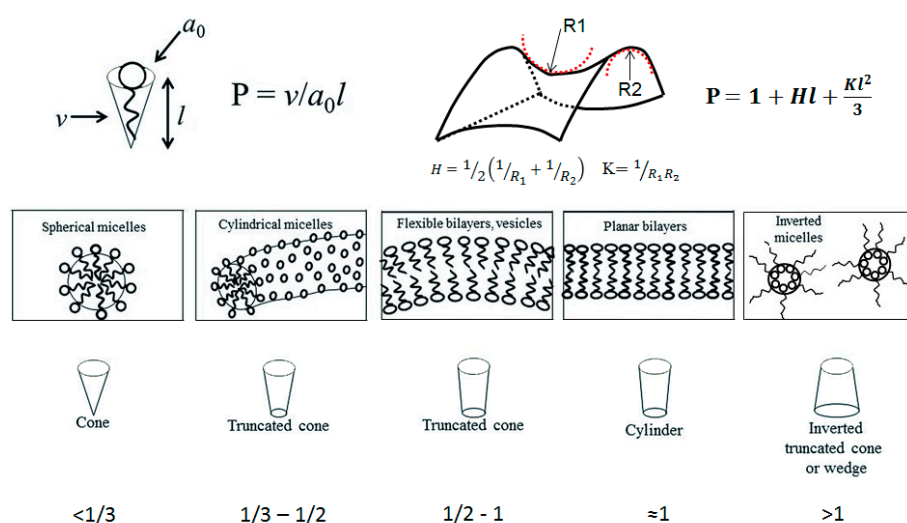
Figure 1. Above: the figure shows the packing parameter versus the geometrical constraints of a typical amphiphile (left) and the correlation with the curvature parameters (right); Below: different self-assembled structures with their corresponding packing parameter values.
