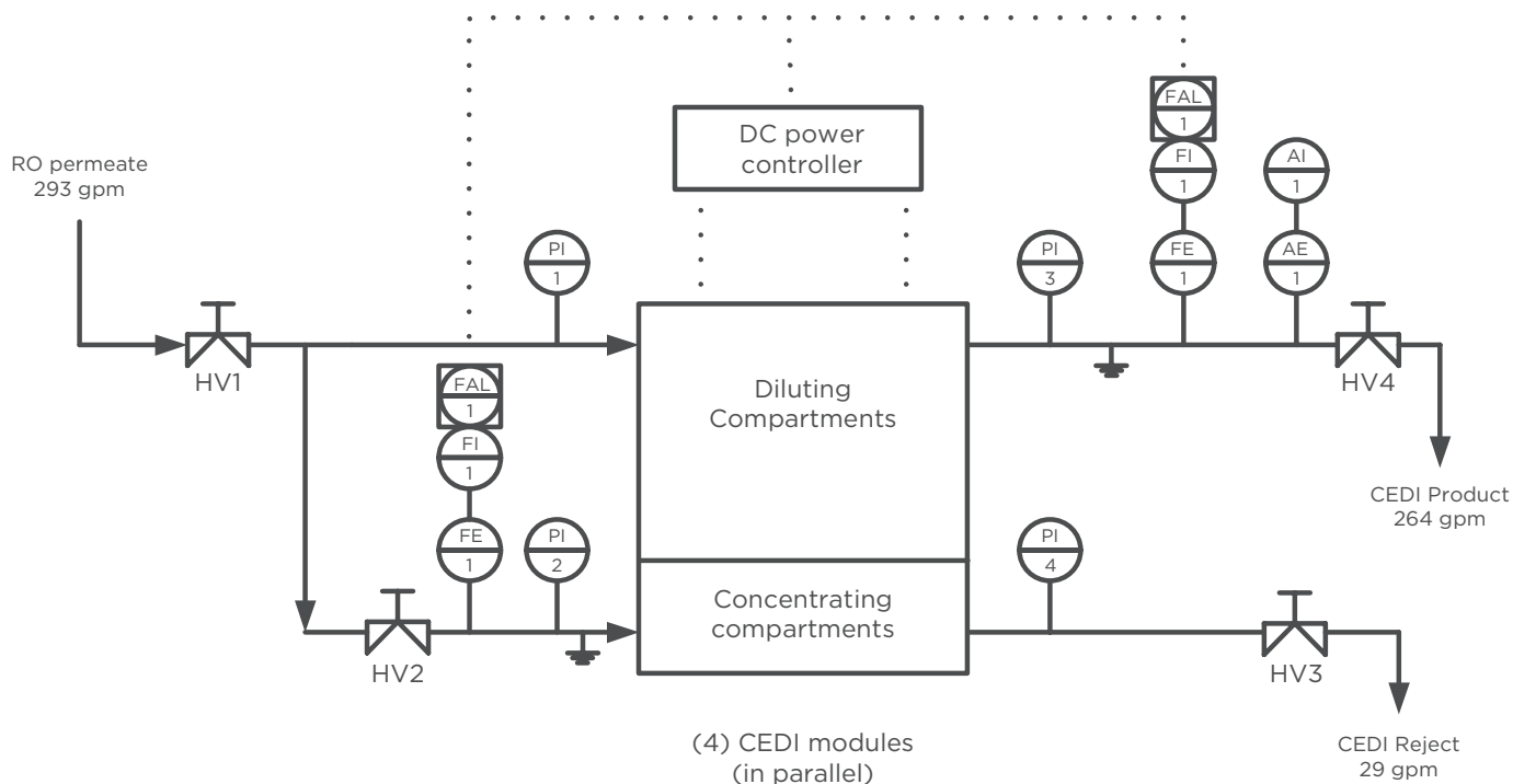
Figure 3 P&ID of 264 gpm (60 m³/h) CEDI system
