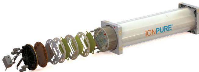
Figure 2 Stacked-disk CEDI module—exploded view
