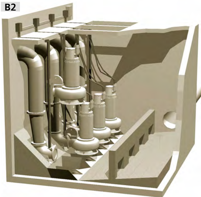
Side - low level entry intake structure
