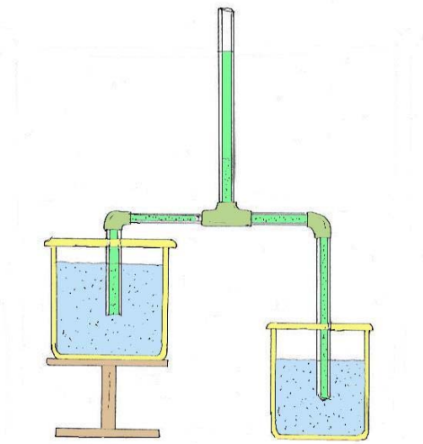
PASCAL'S SIPHON
