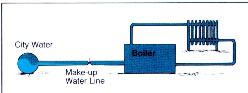
Backpressure Example
