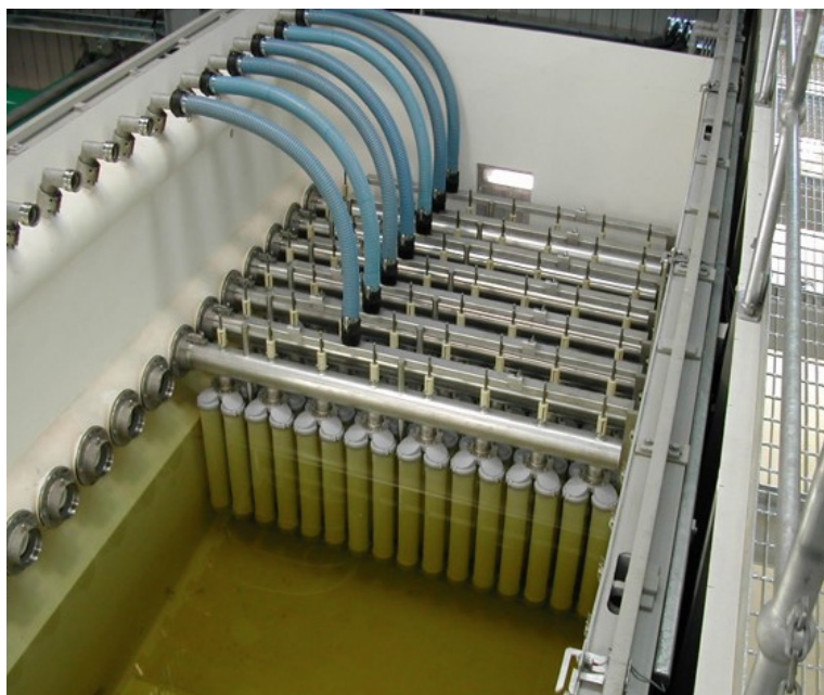
Figure 8.6: Example of submerged membrane.
