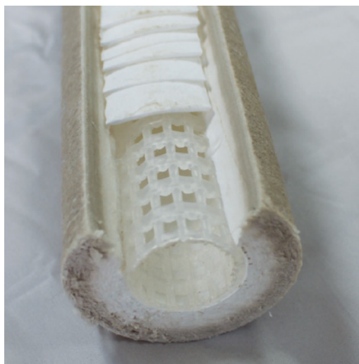
Figure 7.2: Example cross-section of cartridge filter.
