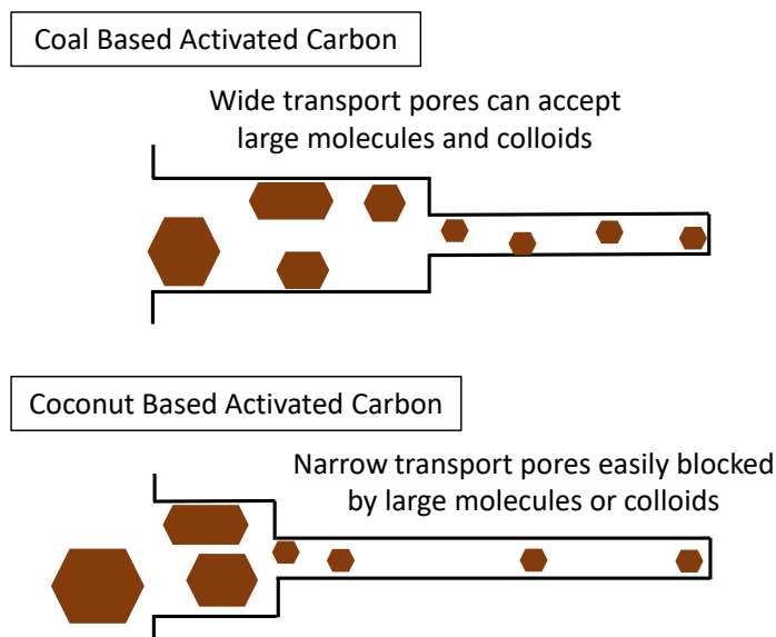
Figure 6.4: Example of pore structure for different carbon media types.
