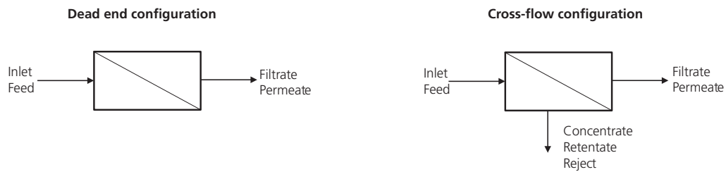
Figure 8.7: Hydraulic configuration of membranes.
