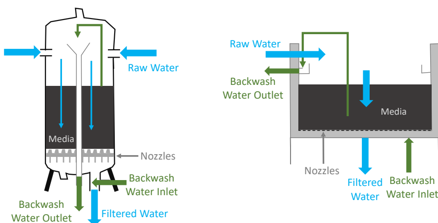
Figure 6.2: Layout of activated carbon.
