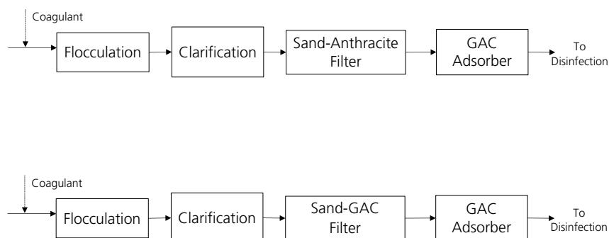
Figure 6.1: Use of GAC media in drinking water typical process trains.
