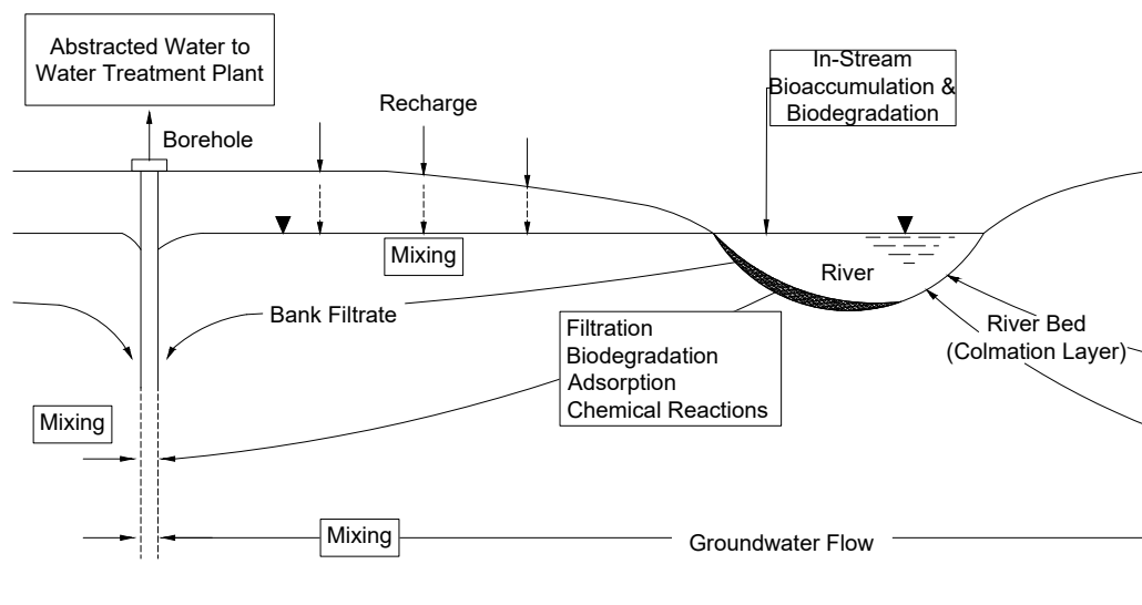
Figure 9.1: Overview of bank filtration.
