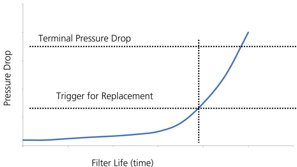
Figure 7.3: Example head loss profile across cartridge filter life.
