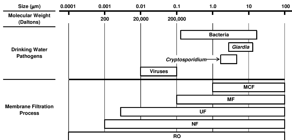
Figure 8.2: Filtration application guide for pathogen removal. 5
