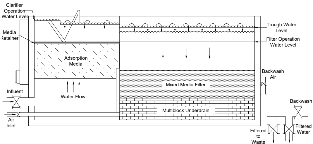
Figure 5.17: Cross-section of adsorption clarifier. 2
