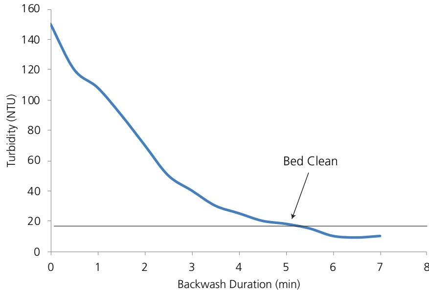
Figure 5.14: Example backwash removal profile.
