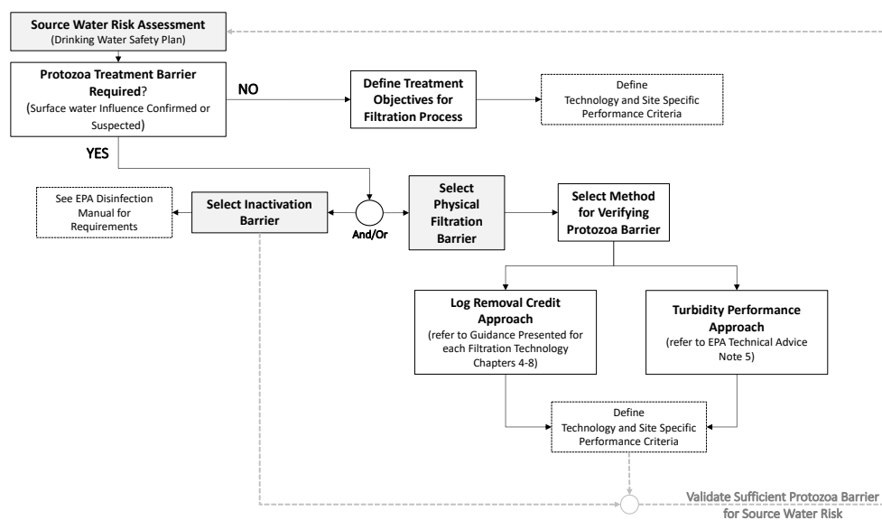
Figure 3.1: Decision tree for verifying protozoa barrier for filtration processes
