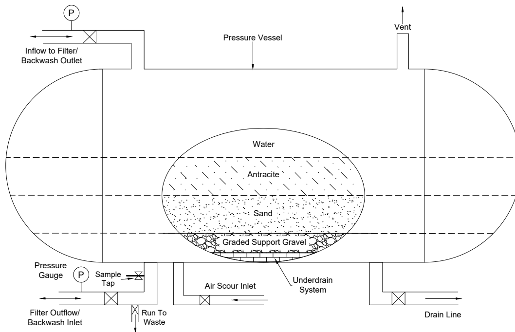
Figure 5.6: Cross-section of a typical horizontal pressure filter.
