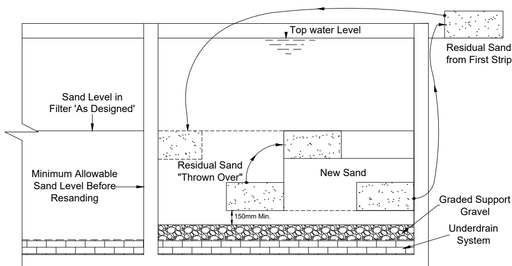
Figure 4.4: Cross-section overview of re-sanding a slow sand filter using the trenching method.
