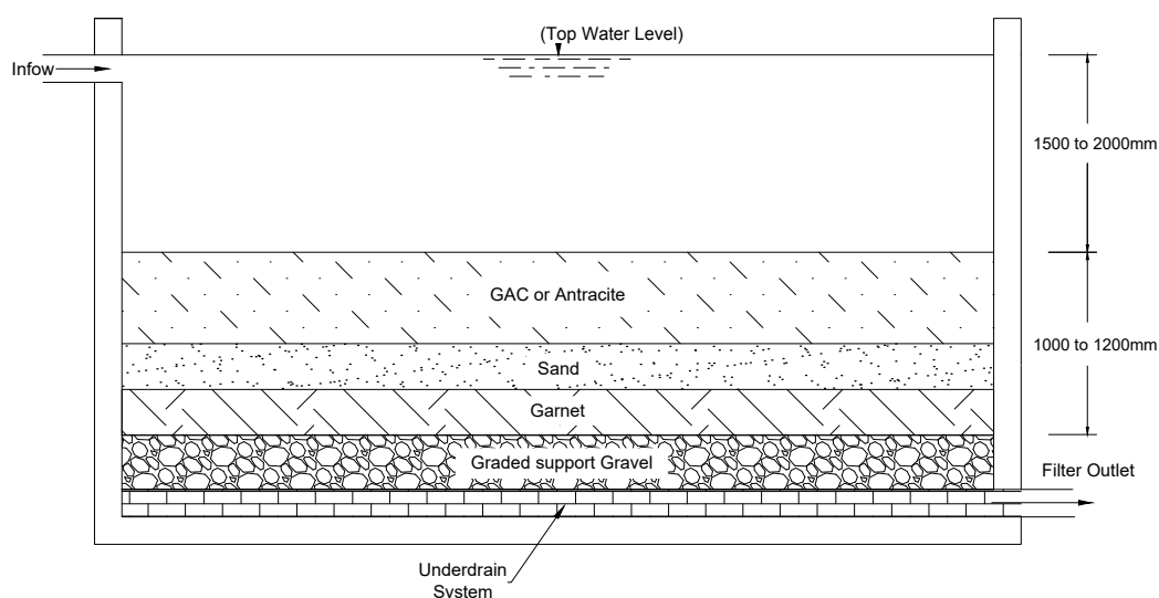
Figure 5.9: Mixed media, tri-media or multi-media configuration.
