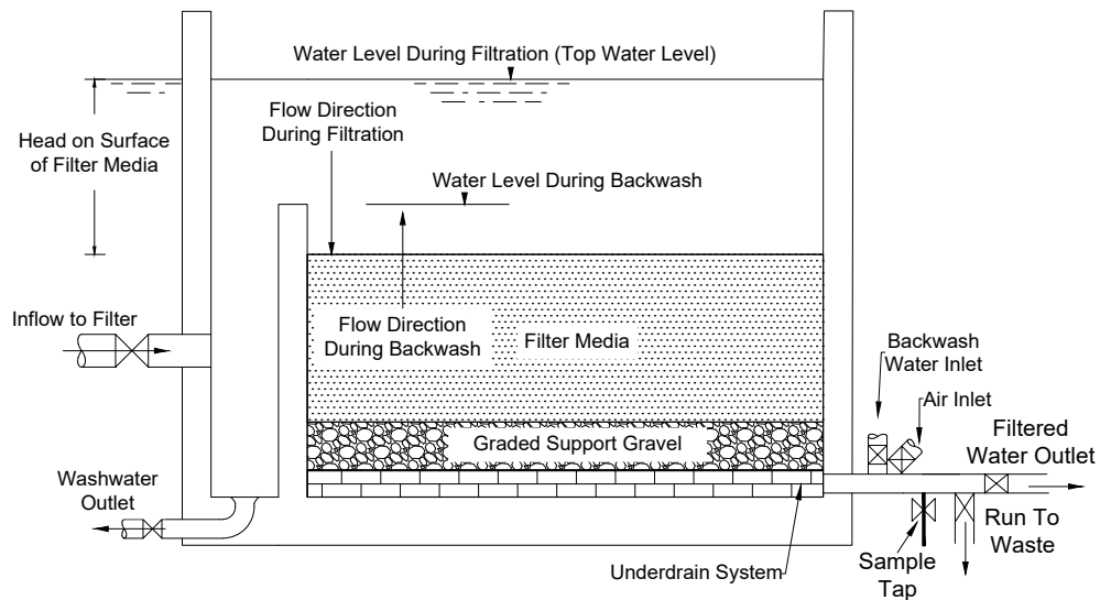
Figure 5.1: Cross-section of a typical RGF filter.
