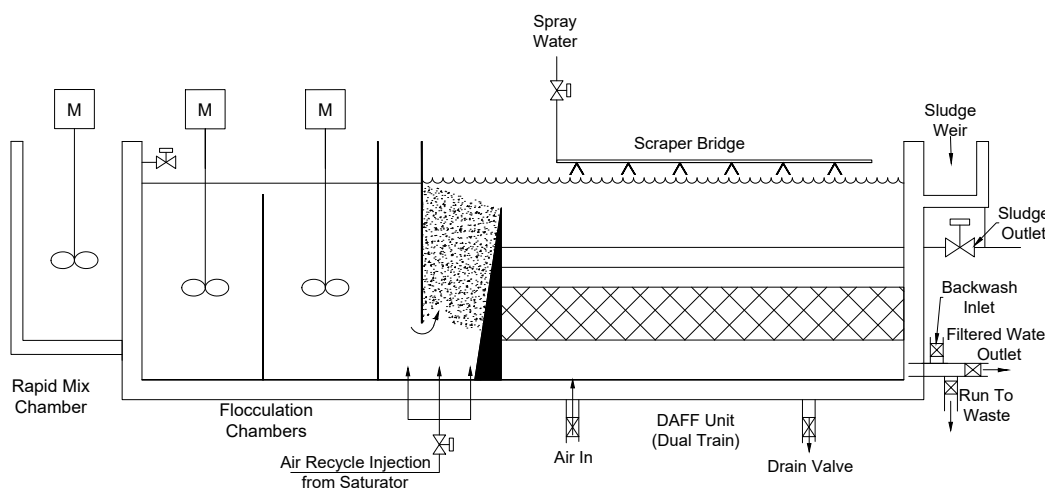
Figure 5.18: Cross-section of dissolved air flotation with filtration unit.
