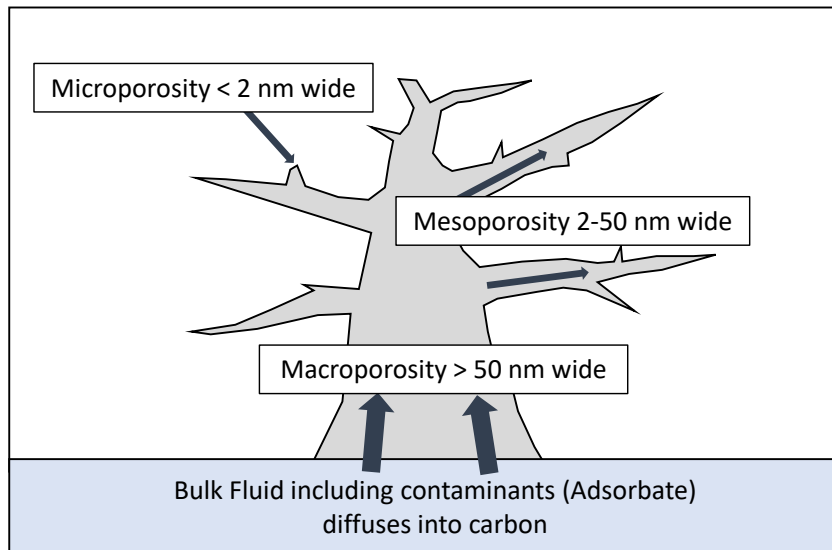
Figure 6.3: “Tree root” structure of activated carbon.
