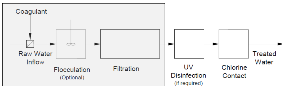
Figure 2.2: Direct filtration
