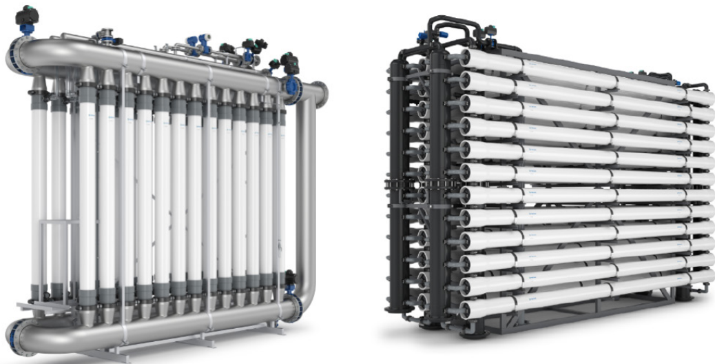
Figure 8.5. Example of pressurised horizontal and vertical configurations.
