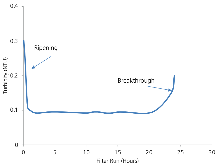
Figure 5.15: Filter performance curve.
