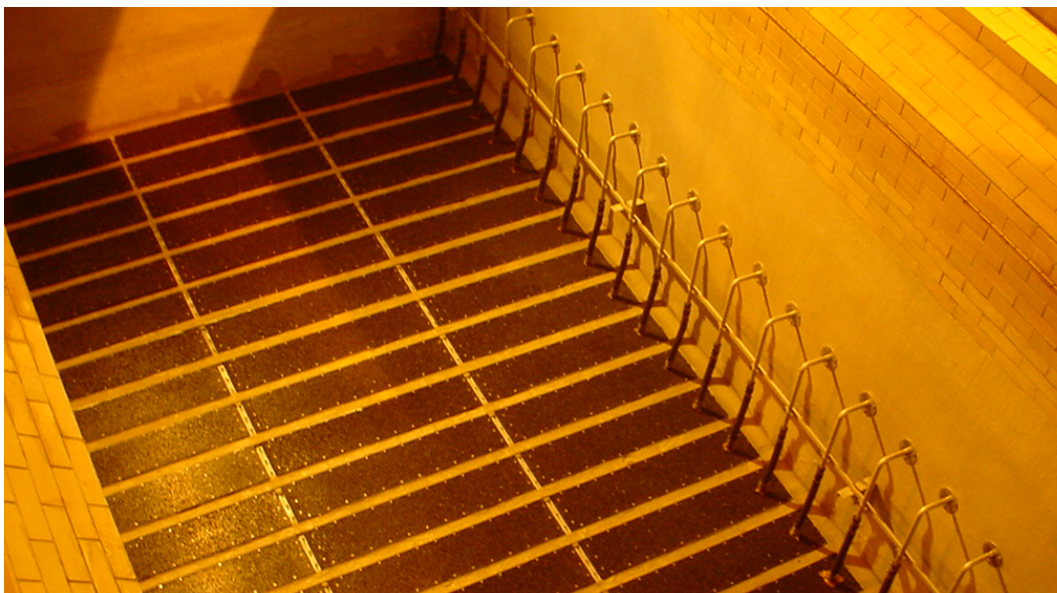
Figure 5.4: Example of a proprietary block floor installation (Leopold® Block Floor System).
