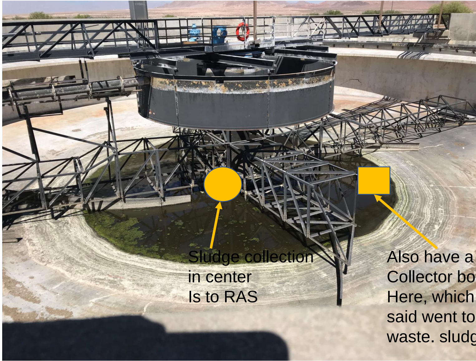
Henderson, Nevada Secondary Clarifiers
