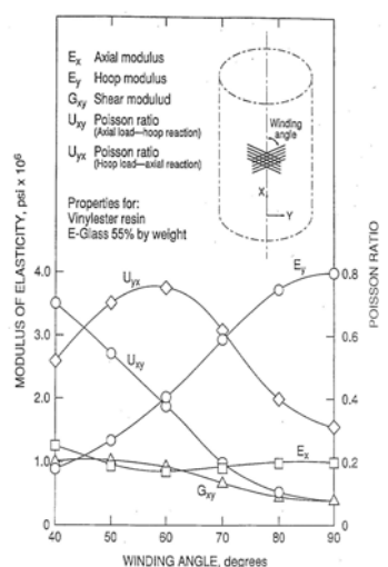
Shell Properties vs. Winding Angle
