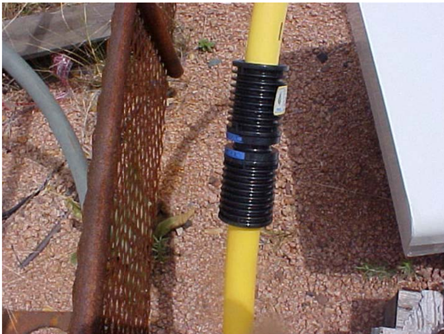
Mechanical (compression) joint on plastic.
