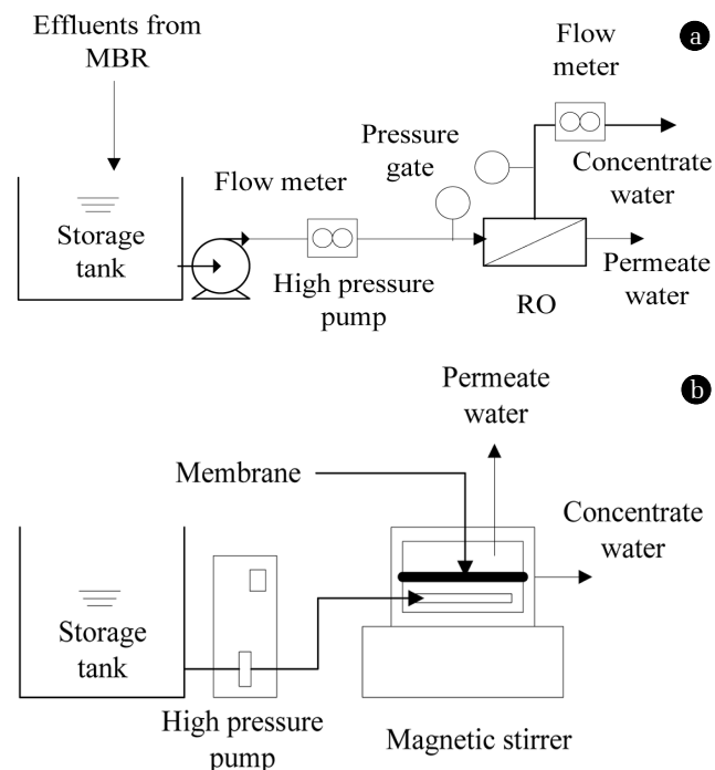
Fig. 2. Schematic diagram of the filtration experimental units. (a) spiral-wound membrane filtration unit; (b) stirring membrane filtration unit.
