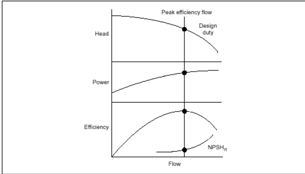
Fig 1. Pump characteristics
