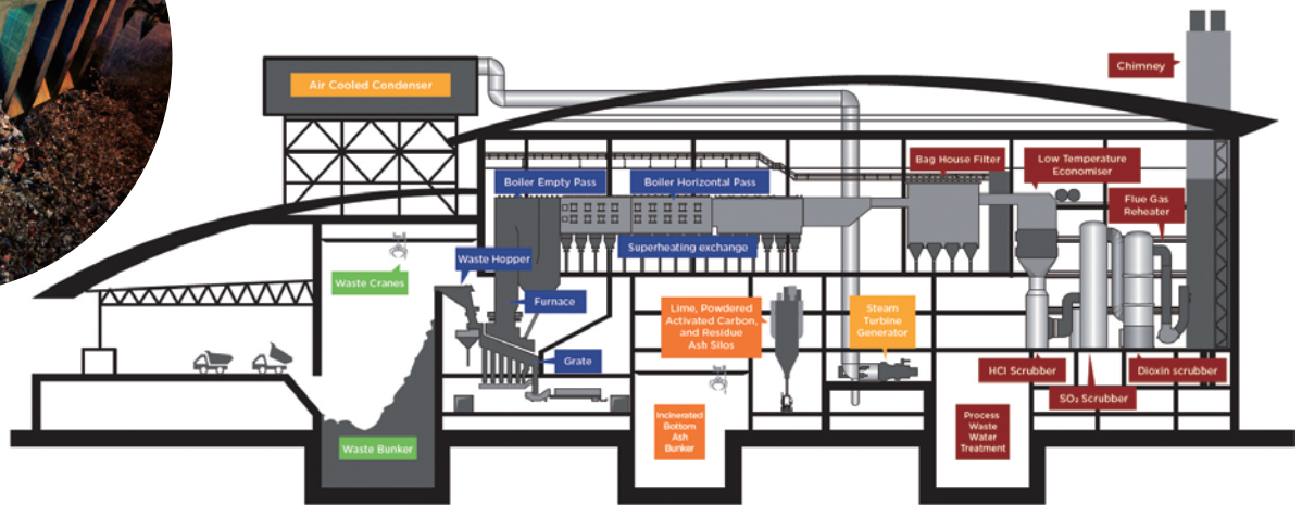
Figure 4. In addition to a Materials Recovery Facility (MRF), the IWMF will also feature a 2,900 tonnes per day Waste-to-Energy (WTE) facility using Keppel Segher's proprietary design which has been tried and tested at the Tuas WTE plant since 2009 (left image). The IWMF will feature air-cooled grates, an advanced combustion system, a segregated boiler system designed to minimise the corrosive impact of flue gases, and a wet flue gas cleaning system to achieve clean air emissions (right image). Photos credit: Keppel (left), National Environment Agency (right)
