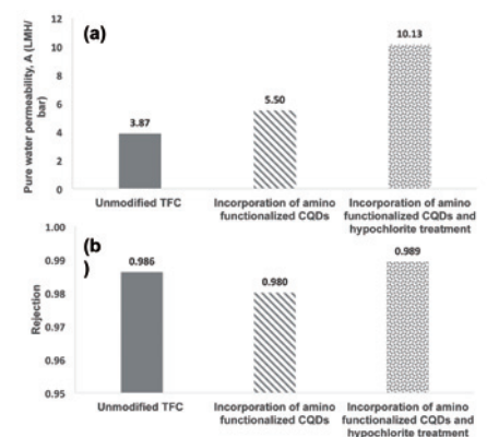
Figure 2. (a) Pure water permeability (Feed: DI water) and (b) salt rejection (Feed: 2000 ppm NaCl aqueous solution) of the unmodified TFC membrane, TFC membranes incorporated with amino functionalised CQDs and TFC membranes incorporated with amino functionalised CQDs after hypochlorite treatment. (Measured at 15 bar after the membranes had been stabilised at 20 bar for 1h.)
