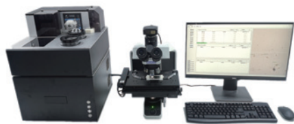
Figure 1. A photo of the automated phytoplankton monitoring system based on deep learning. It consists of a batch sample feeder and controller, a scanning digital microscope and a computer with the plankton identification software.
