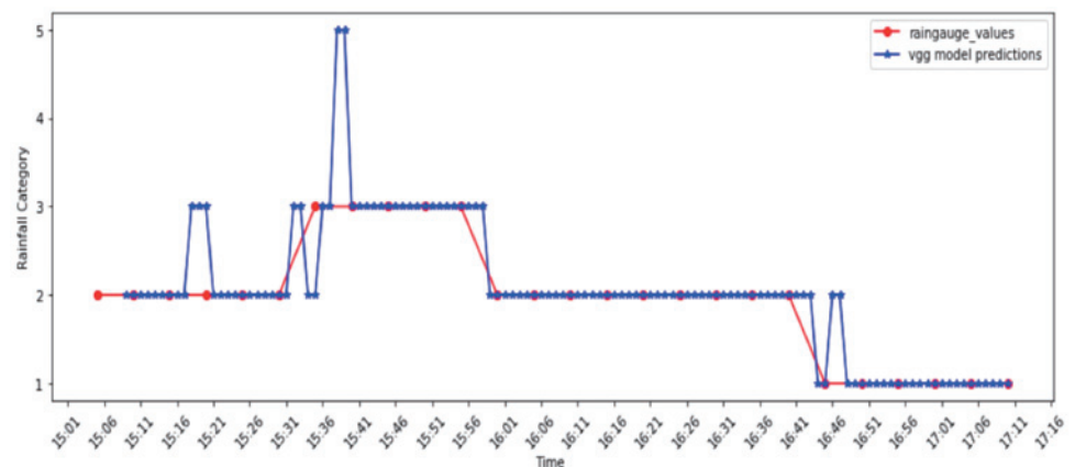
Figure 2. This chart compares the CCTV's rainfall readings (VGG model) with that of a nearby rain gauge. Note that rainfall category 1 refers to no rain and the CCTV and rain gauge are within 123m of each other.
