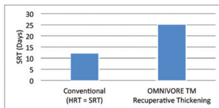
Comparison of specific solids retention times (SRT)
