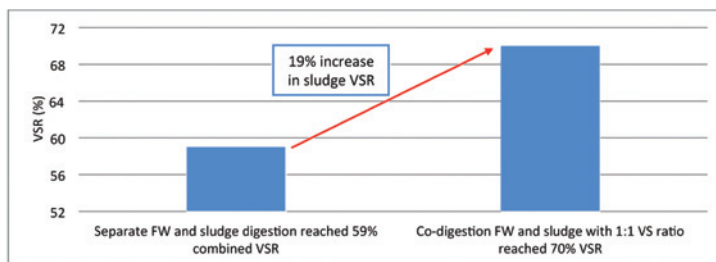
Comparison of volatile solids reduction (VSR) between separate and co-digestion operation
