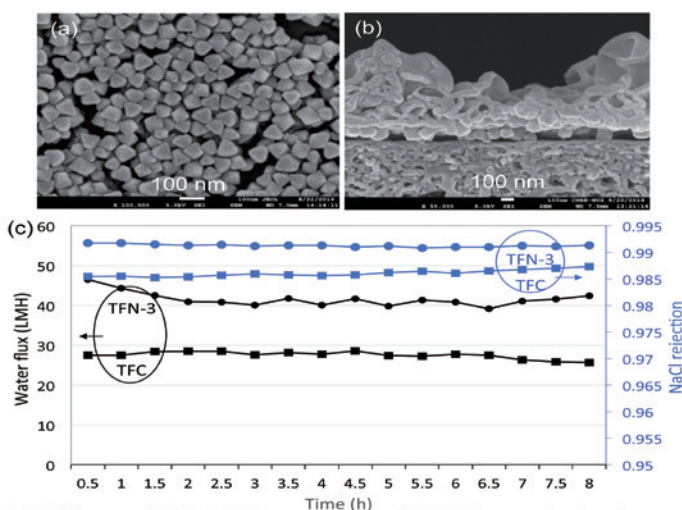
Figure 1. (a) Scanning electron microscope (SEM) image of UiO-66-NH 2 nanoparticles, (b) SEM image showing the cross section of UiO-66-NH 2 incorporated TFN membranes and (c) performance of TFC and TFN membranes in seawater reverse osmosis processes (Feed: 32,000 ppm NaCl; flow rate: 2 L/min; operation pressure: 50 bar).
