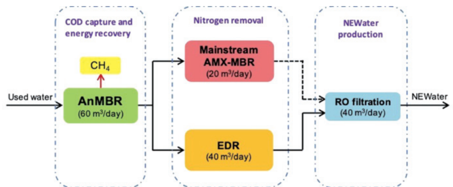
Figure 2. The Novel A-B processes.
