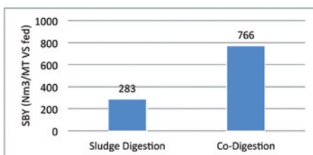
Comparison of specific biogas yields (SBY)
