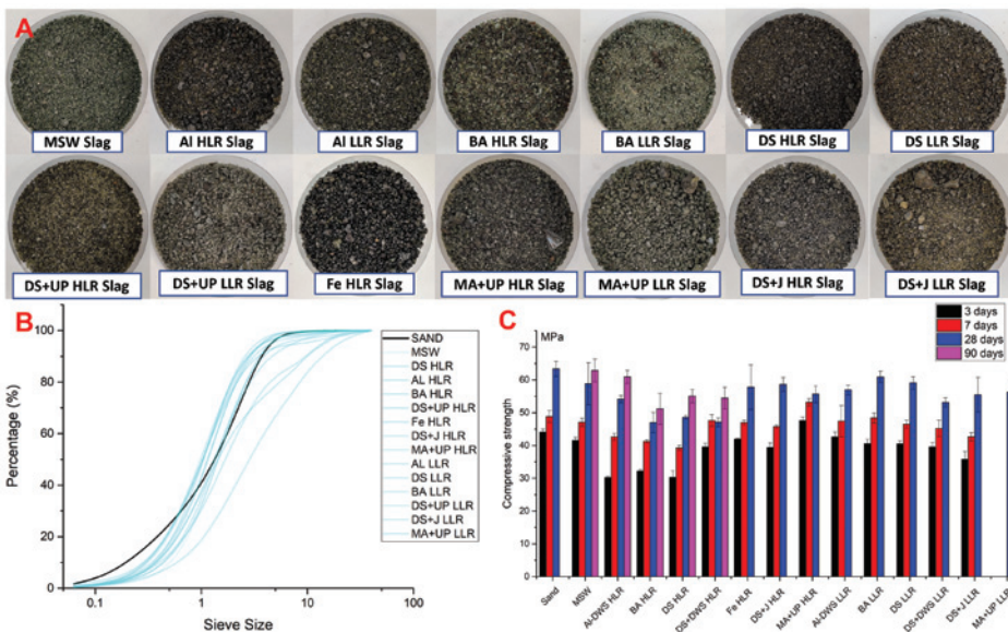
Figure 1. Photos illustrating different types of slag generated from the co-gasification research at the WTERF. The chart below shows the particle size distribution analysis of slag and sand, and the test results for compressive strength of mortar produced from using this slag, which replaces sand as the fine aggregate. The testing is currently ongoing.
