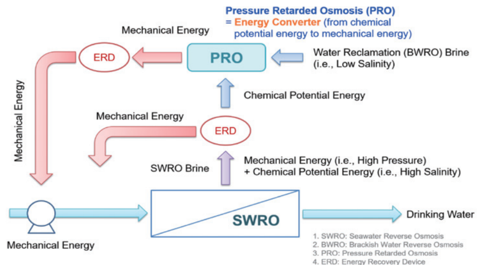
Figure 1. Energy recovery based on high salinity PRO in an SWRO desalination process.
