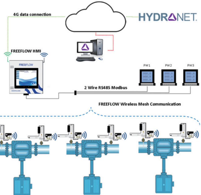
Figure 2. Data transmission landscape in the Riventa FREEFLOW system, from pump to operator.
