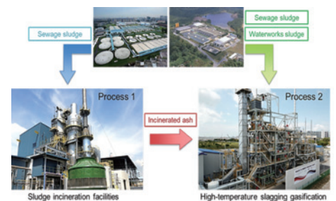
Figure 2. An overview of the thermal treatment processes that go into creating NEWSand from a combination of different waste streams.
