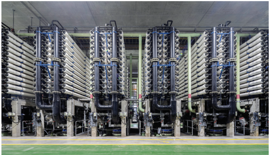
Figure 4. Direct coupling of the ultrafiltration process (on the right) with the downstream reverse osmosis process eliminates the need for intermediate break tanks and pumping, reducing energy and footprint. Photo credit: Keppel
