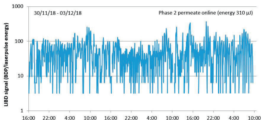
Figure 2: An example of the LIBD online measurement at KNF.
