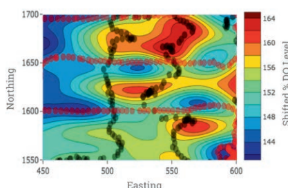
b) Predicted field from data collected along the standard lawnmower path. Time taken 1256s, Root Mean Square Error=6.6.
