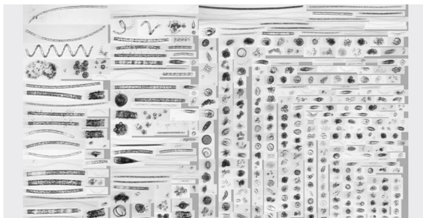
Figure 2: Dashboard showing IFCB images of phytoplankton (single-celled algae) from a sample collected from Marina Reservoir. Considerable diversity is evident, from long chains or colonies of cells to solitary cells. These images were collected just a few minutes after the sample was put in the IFCB.
