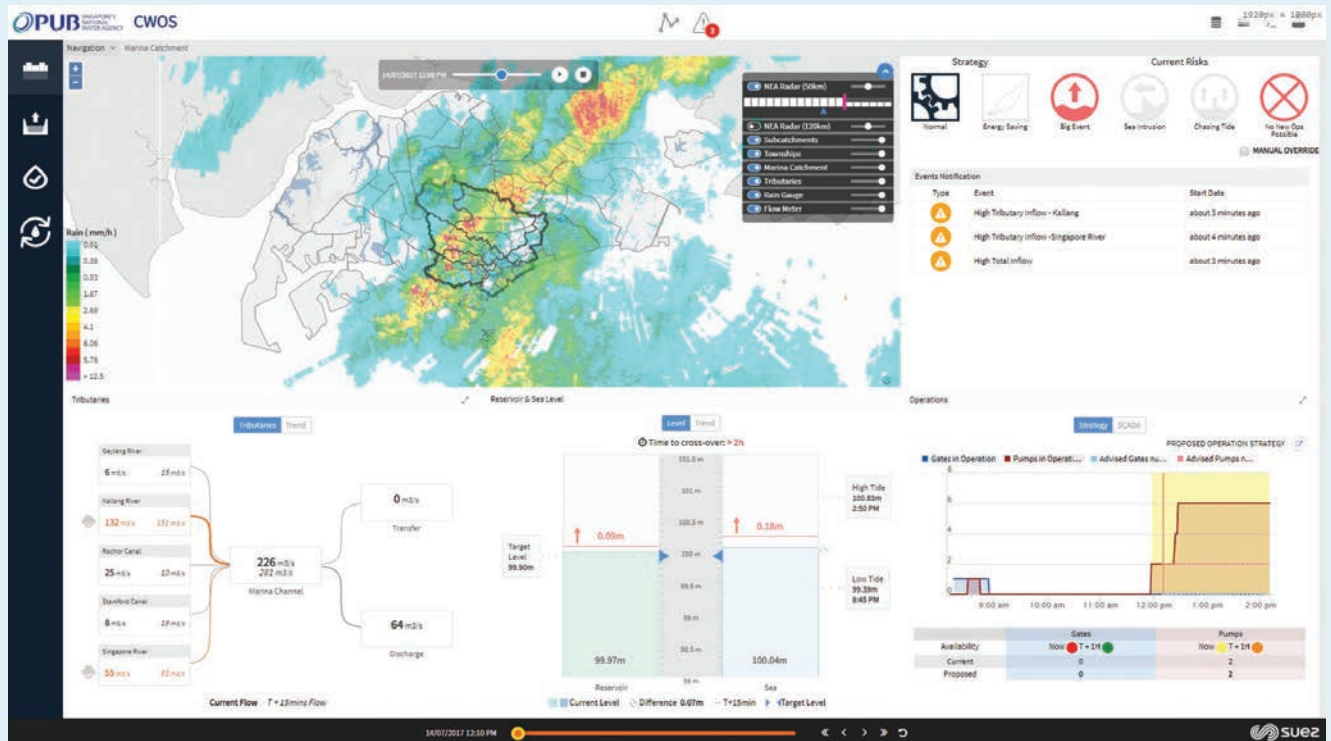
Figure 3: Marina Barrage operations overview – Numbers and values are for illustration purposes only.
