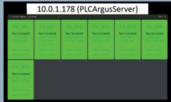
Real time monitoring of cyber-physical health of each component of a particle stage. Image shown is the panel for monitoring of Stage 4 of SWaT (i.e. de-chlorination process).
