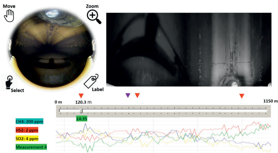
Figure 2: Automated generation and visualisation of the UAV's inspection results.
