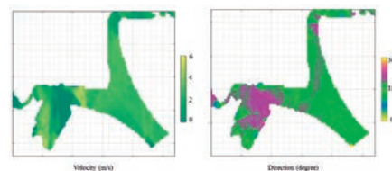
Figure 3: Wind velocity and direction at noon for the South West Monsoon season on 1 August 2014, generated using a combined three-dimensional computational fluid dynamics and probability model with 20 m x 20 m grid cells over the Marina Reservoir. Wind directions are generally from 180-degree with the exception of Marina Bay, where wind direction is shifted to 270-degree due to structures close to the reservoir. Wind velocity is also altered in the Marina Basin, where winds in excess of 5 m/s are observed around the edges of the Marina Bay Sands while velocities are substantially reduced in the wake region.
