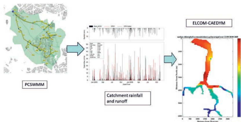
Figure 1: Representation of how a catchment model (PCSWMM) translates rainfall data into runoff input for a reservoir model (ELCOM-CAEDYM), to predict Kranji Reservoir water quality.
