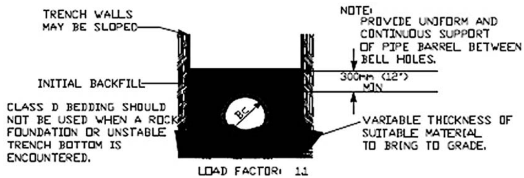
(a) CLASS D, FLAT OR RESTORED TRENCH BOTTOM
