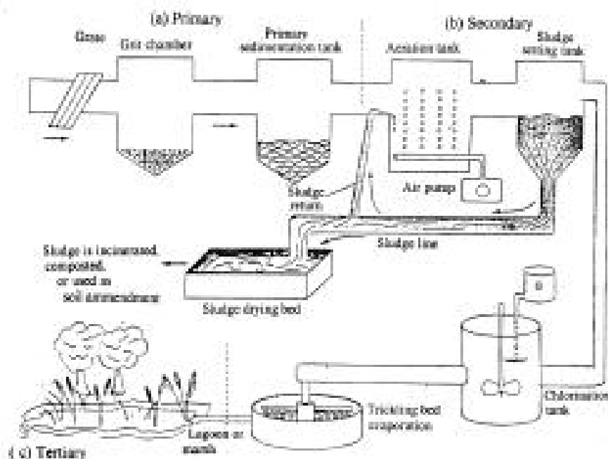
Fig 34.3 : Treatment process of sewage
