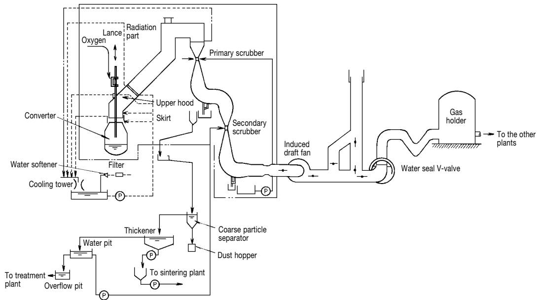
Fig. 8.7 Flow diagram of a oxygen converter gas recovery system (OG system)
