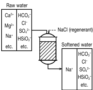
Fig. 2.31 Softening treatment
