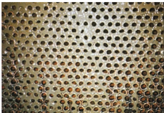
Photo 5.3 Condition of a refrigerating machine condenser treated without slime control agent
