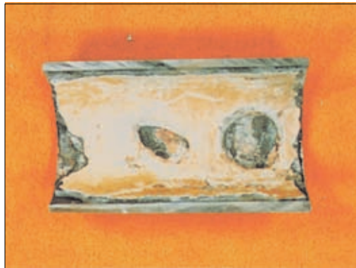
Photo 2.2 Expansion of an evaporation tube by scaling of silica
