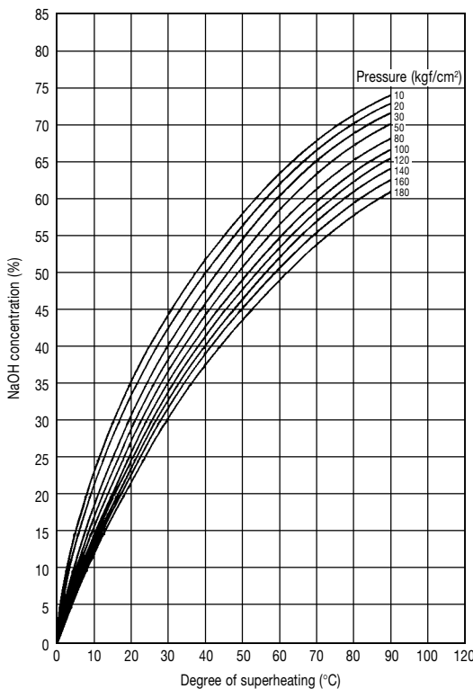
Fig. 2.24 Relationship between the degree of superheating at the inner surface of boiler tube and the highest concentration of NaOH in the concentrated film
