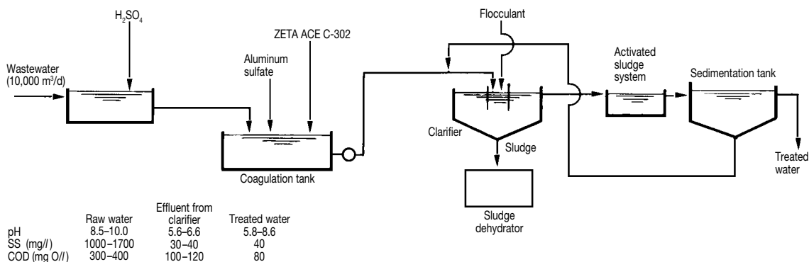
Fig. 4.16 Case 2, wastewater treatment of a toilet paper factory
