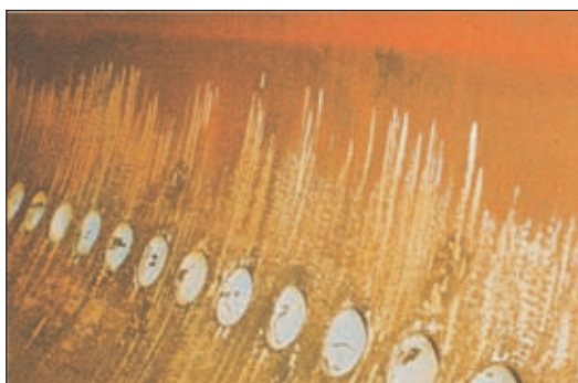
PHoto 2.17 Inside of a boiler treated with a phosphate based boiler compound during 1 year
