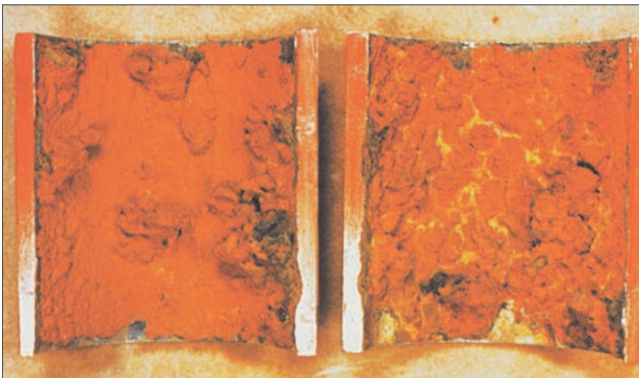
Photo 2.3 Corrosion of an economizer tube
