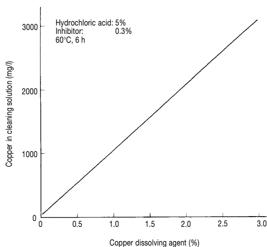
Fig. 9.10 Effect of a copper dissolving agent on a metallic copper scale
