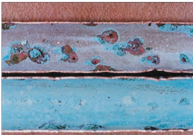
Photo 5.8 Corrosion of the copper tube of an air handling unit without chemical treatment
