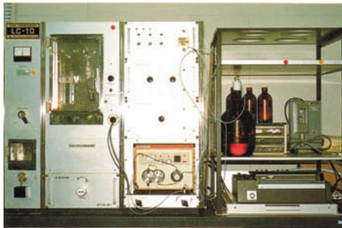
Photo 11.12 Ion chromatograph
