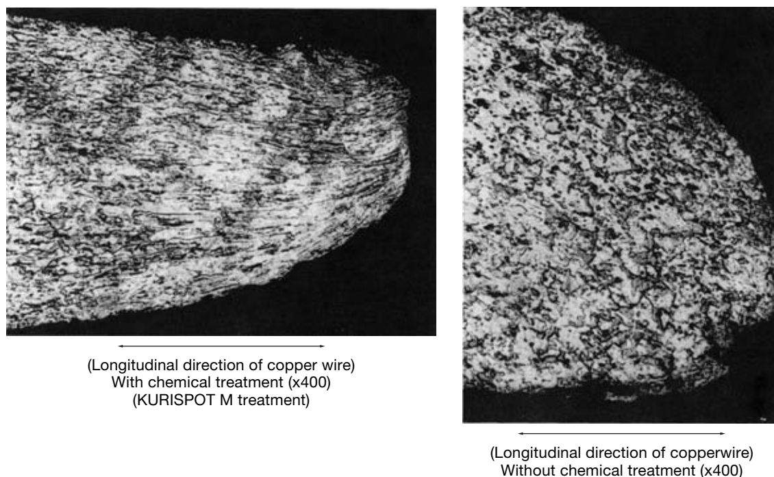
Photo 10.5 Comparative microstructures of broken copper wires with and without a chemical treatment
