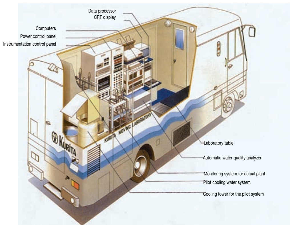
Fig. 3.78 Illustration of main equipments loaded on the KML
