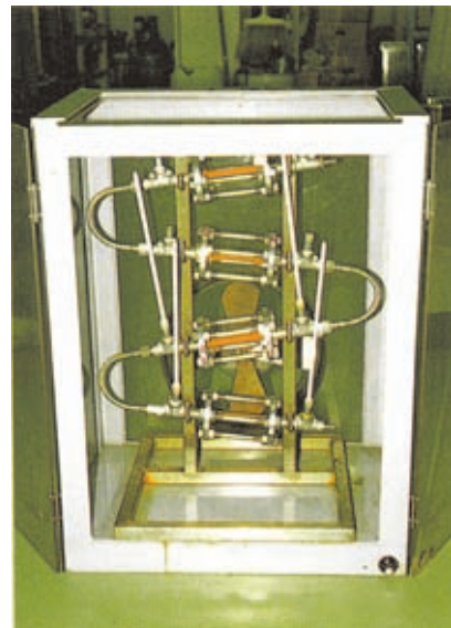
Photo 7.4 Corrosion test apparatus for the initial condensation zone of fractionators
