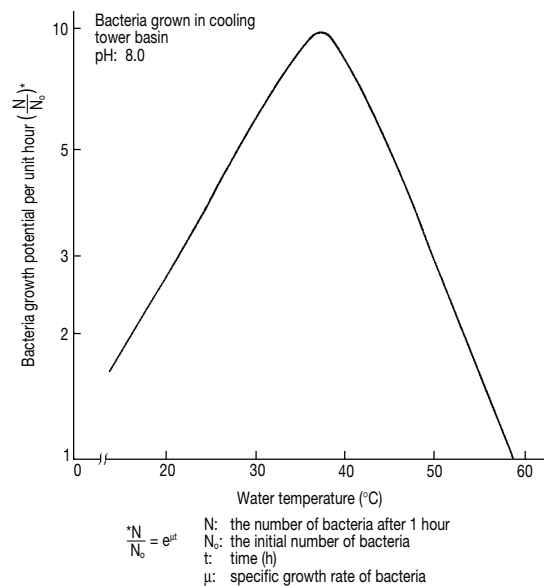
Fig. 3.50 Influence of water temperature on the growth rate of bacteria
