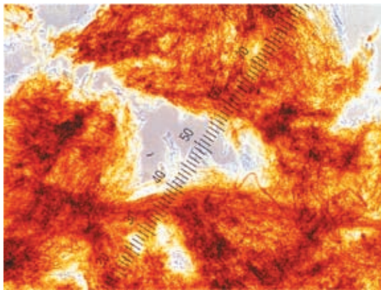
Photo 11.22 Leptothrix sp. (iron bacteria) (x 200)
