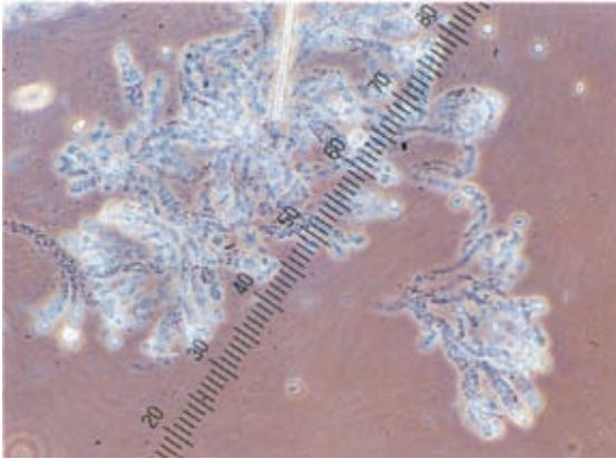
Photo 11.20 Zooglea sp. (bacteria) (x 200)
