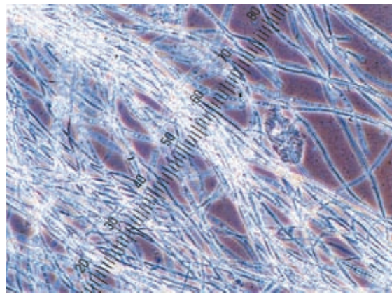
Photo 11.23 Geotrichum sp. (fungi) (x 400)
