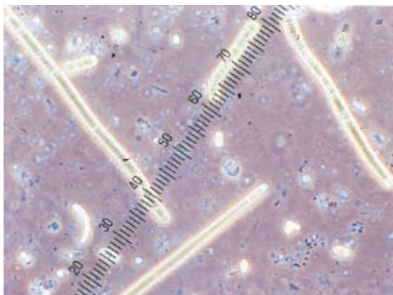
Photo 11.17 Oscillatoria sp. (blue-green algae) (x 400)
