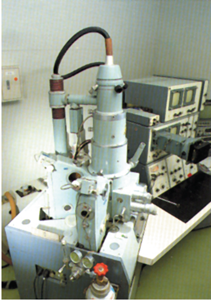
Photo 11.5 Electron probe X-ray microanalyzer
