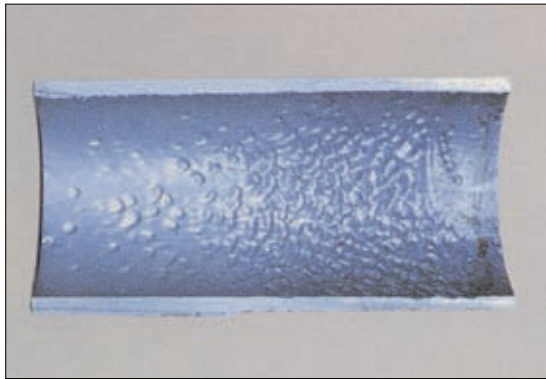
Photo 2.7 Inlet attack of an economizer tube (tube inside)
