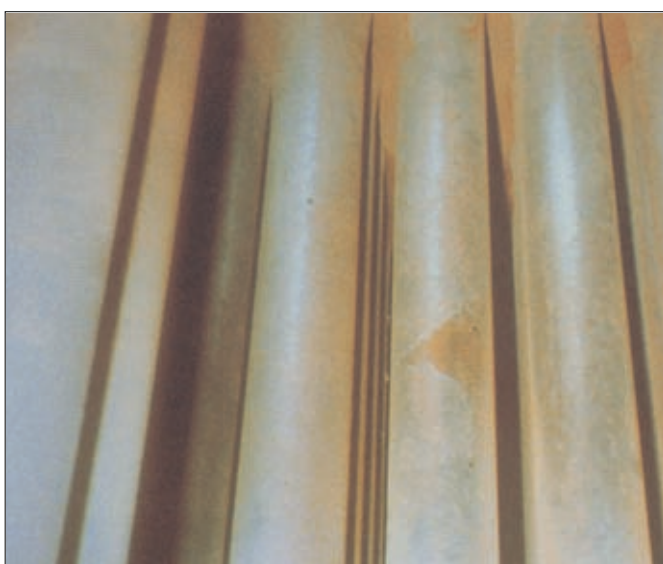
Photo 2.27 Inside condition of a smoke tube boiler treated by a saccharide based oxygen scavenger
