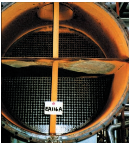
Photo 3.13 Appearance of a heat exchanger treated by an alkaline treatment
