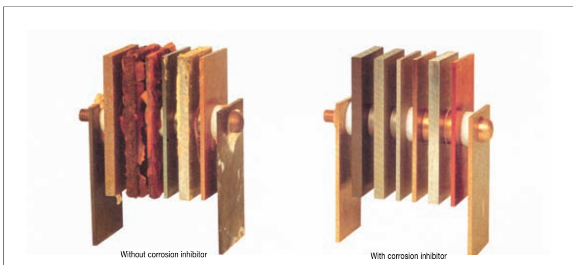
Photo 5.13 Corrosion inhibition effect of a formulated inhibitor on multi-metal coupling in a propylene glycol antifreeze (materials: copper, solder, brass, carbon steel, cast iron and cast aluminum from the right side)
