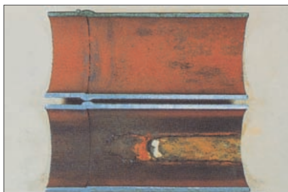
Photo 2.6 Corrosion of a steam condensate line
