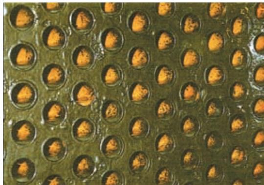
Photo 5.2 Tube sheet of a centrifugal refrigerating machine condenser treated by a Non-P multi-chemical
