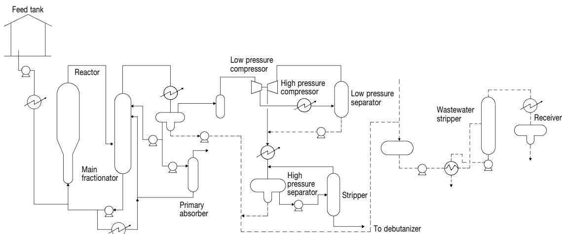
Fig. 7.18 Flow diagram of a fluid catalytic cracking unit
