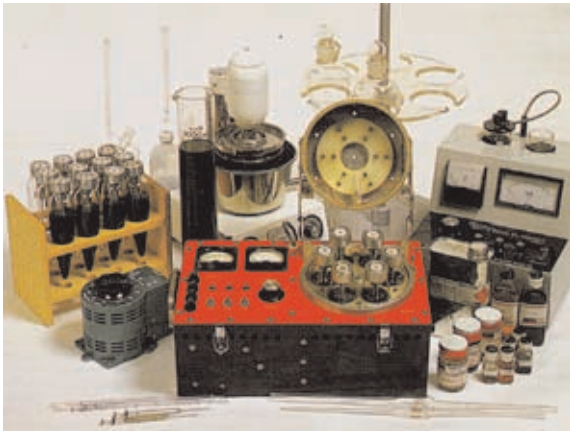
Photo 7.1 Electric dehydration and desalting apparatus (EDDA)
