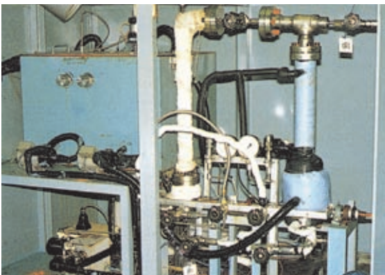
Photo 7.3 Testing apparatus of antifouling agents for depropanizers (dynamic tester)
