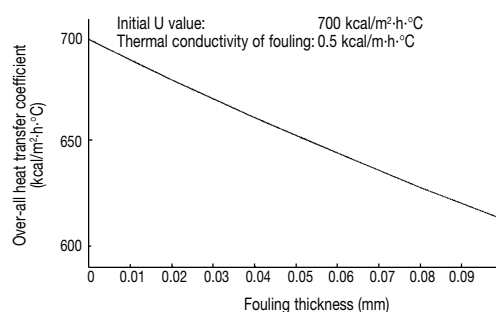
Fig. 3.8 Relationship between the fouling thickness of an heat exchanger and the reduction of the overall heat transfer coefficient
