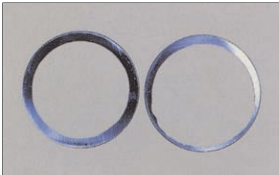
Photo 2.8 Inlet attack of an economizer tube (cross-section of tube)
